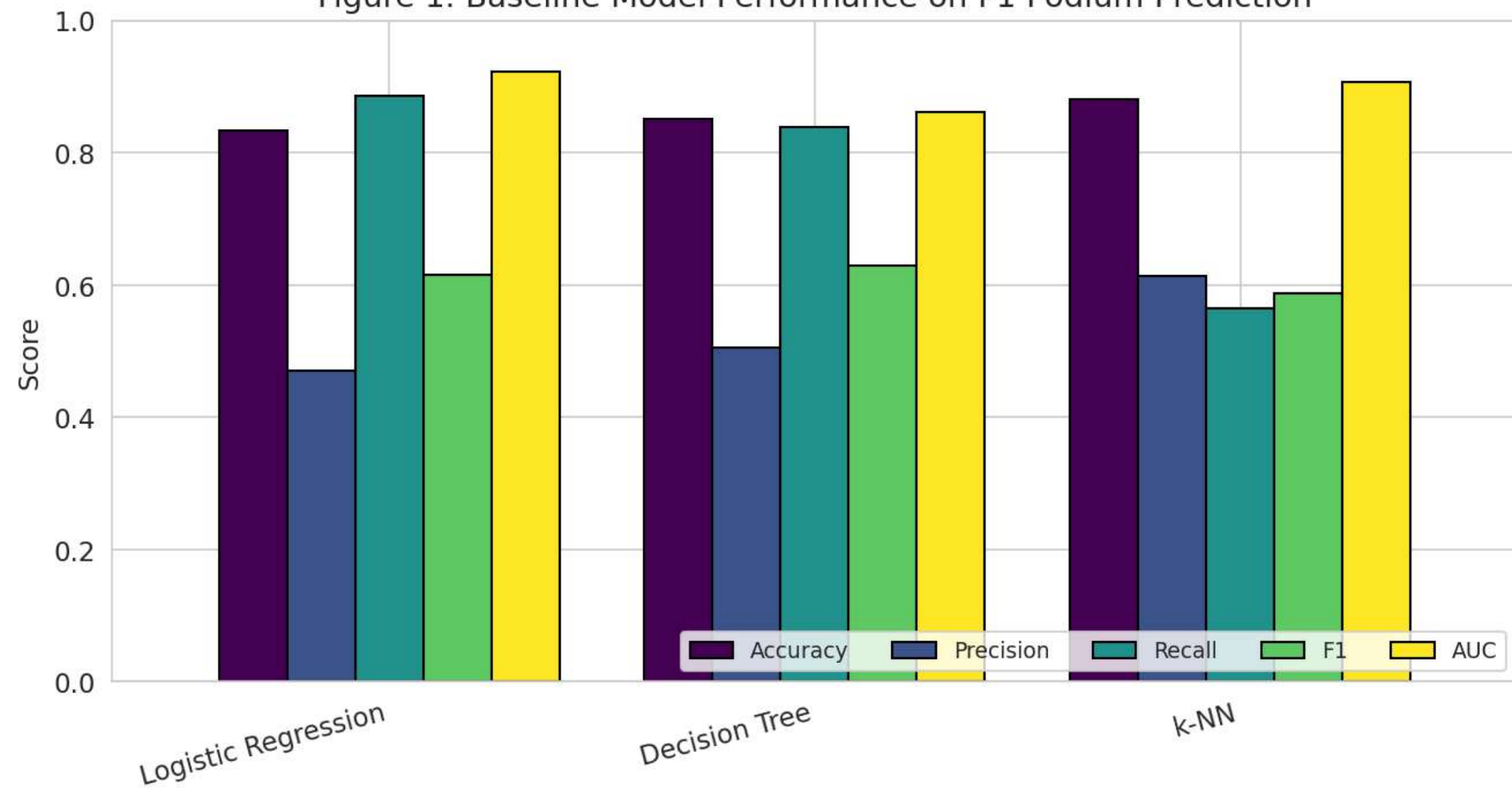
Figure 1. Baseline Model Performance on F1 Podium Prediction
