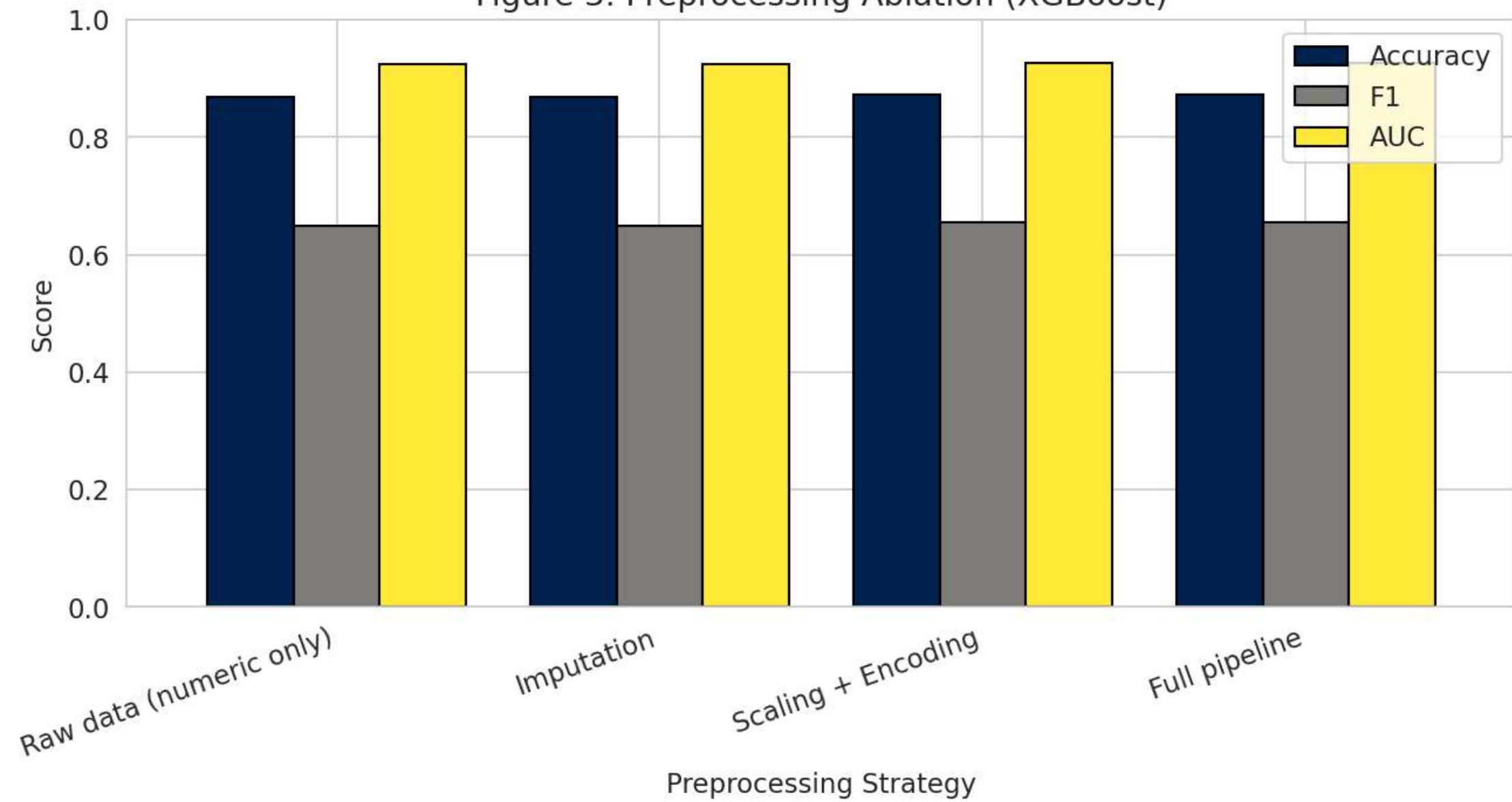
Figure 3. Preprocessing Ablation (XGBoost)
