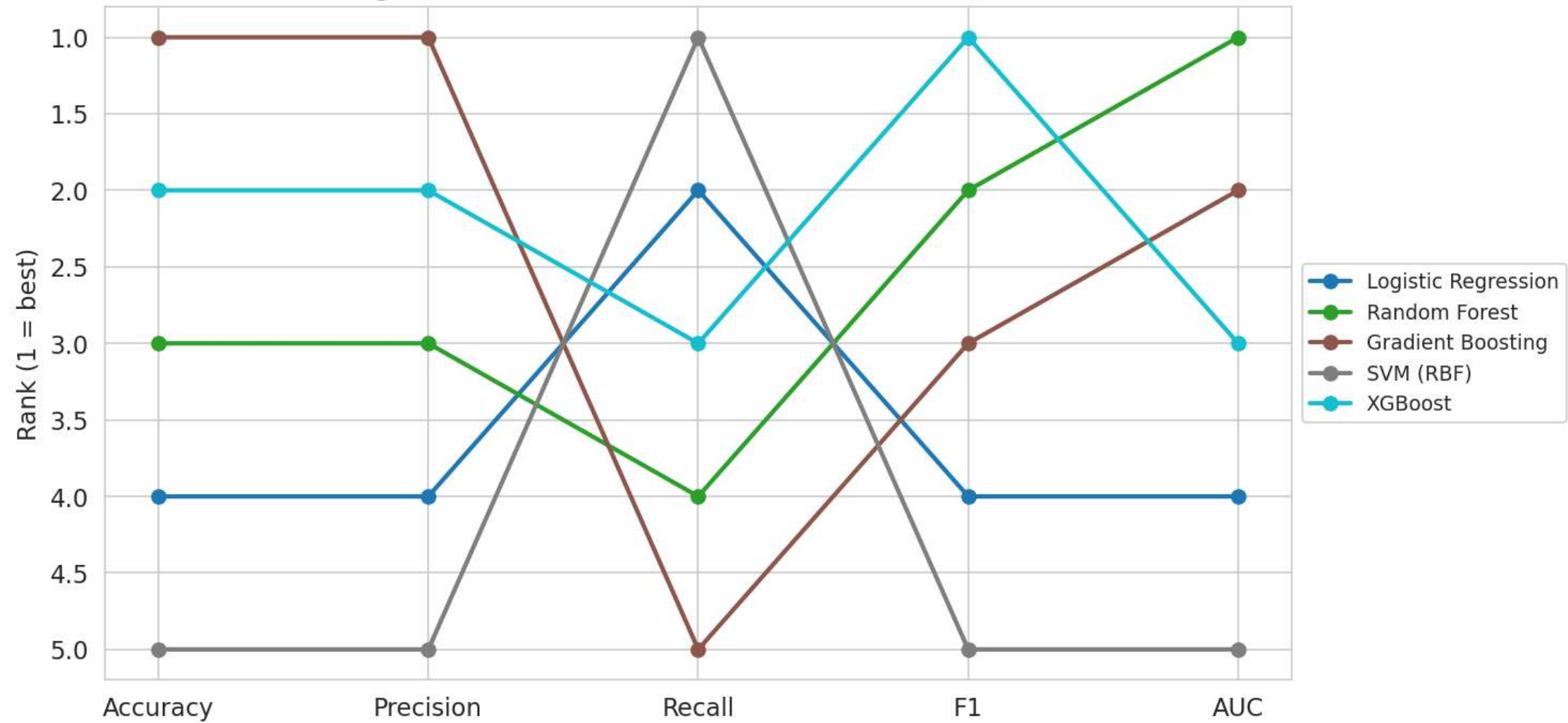
Figure 5. Model Rank Across Evaluation Metrics
