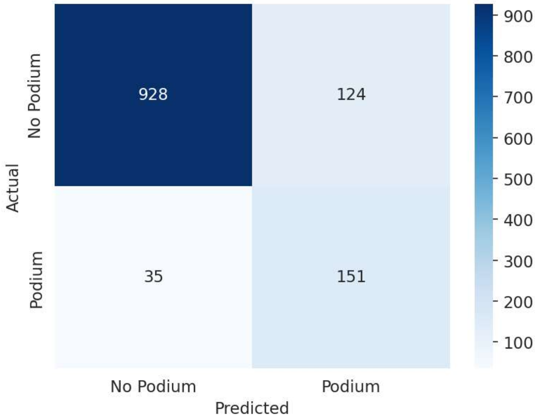
Confusion Matrix — XGBoost (Test Set)
