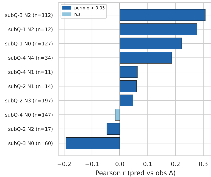
D Per-niche concordance (4 slices)
