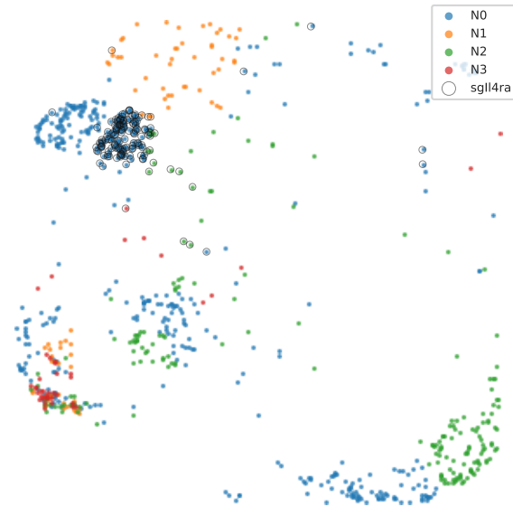
A \beta -Leiden niches + sgll4ra cells subQ-1 immune
