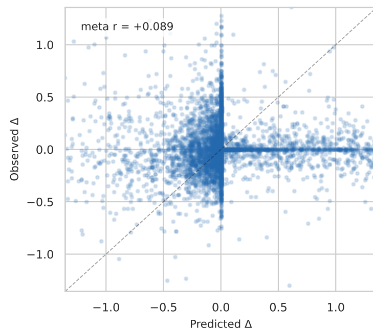
sgCks1b | immune median niche r = +0.055
