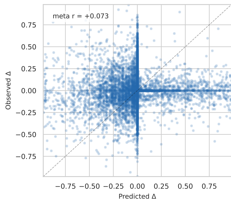
sgCks1b | myeloid median niche r = +0.073
