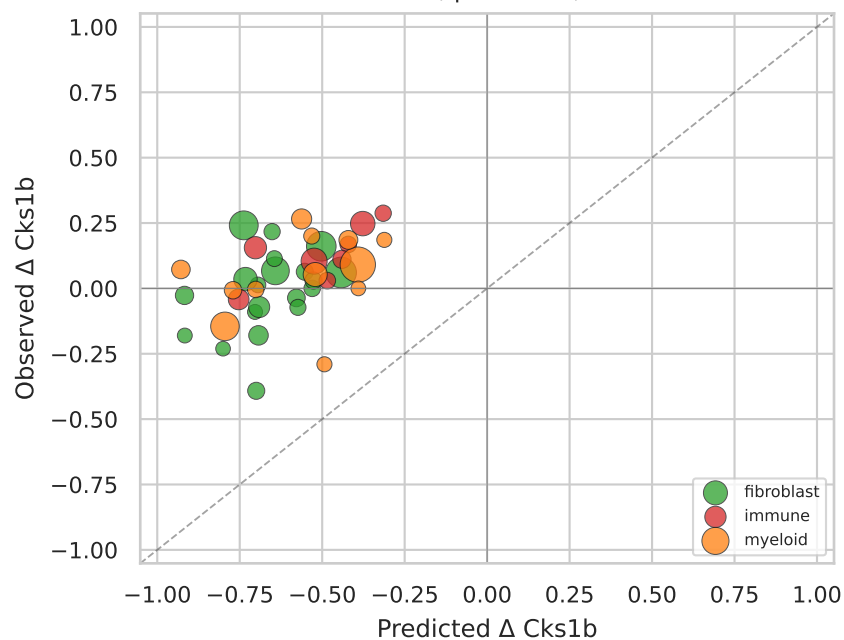
sgCks1b on-target (niche pseudobulk) r = +0.593 , p = 0.000 , n = 45
