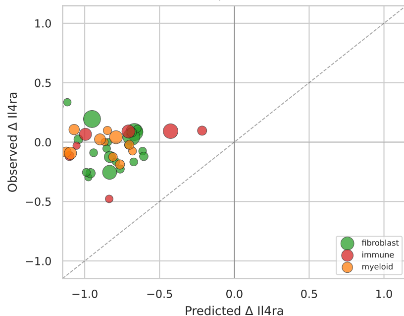
sgIl4ra on-target (niche pseudobulk) r = +0.170 , p = 0.264 , n = 45
