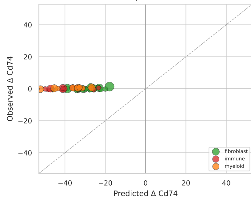
sgCd74 on-target (niche pseudobulk) r = +0.234 , p = 0.083 , n = 56
