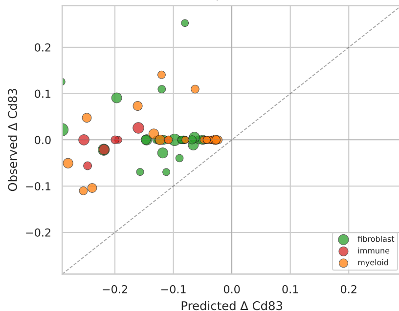
sgCd83 on-target (niche pseudobulk) r = +0.356 , p = 0.005 , n = 61
