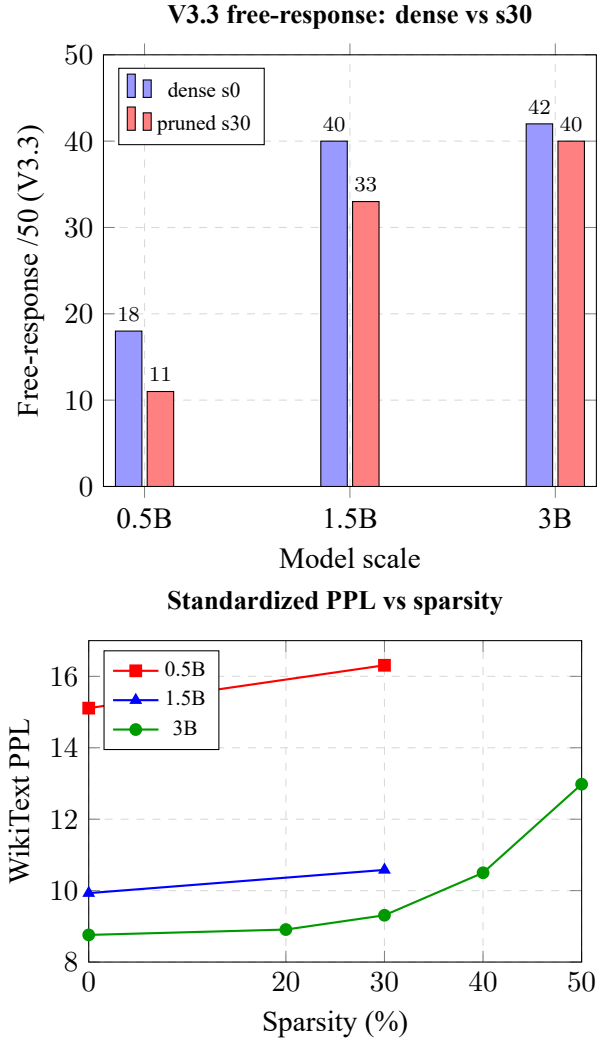
Figure 1: V3.3 free-response scores, dense vs s30 (top), and standardized PPL vs sparsity (bottom).
