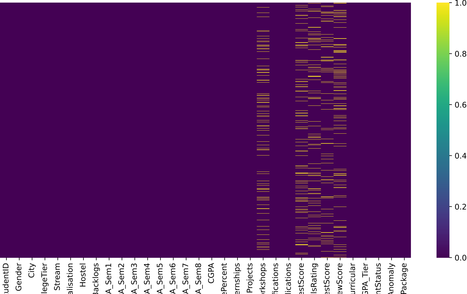
Missing Value Heatmap
