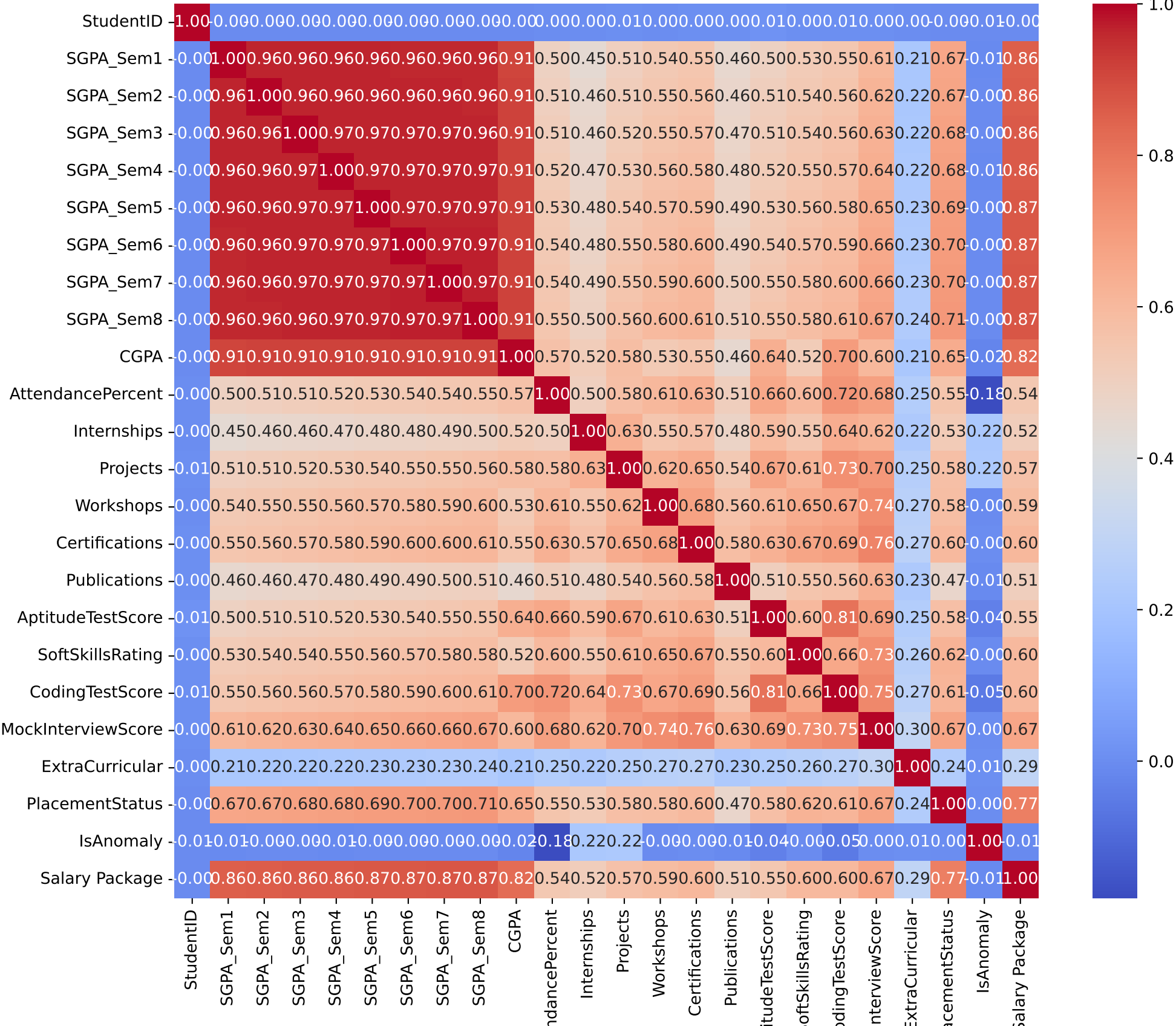
Correlation Heatmap
