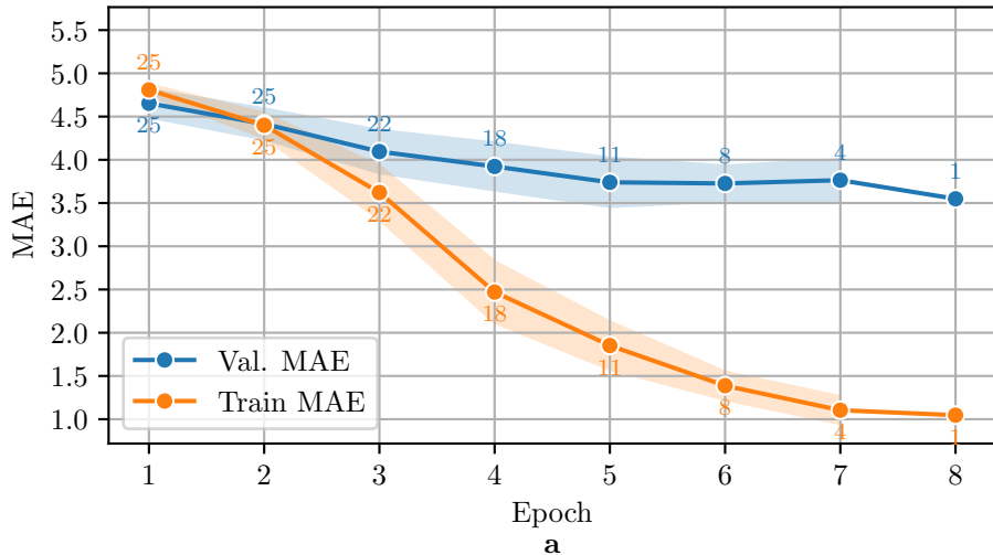
With subject leakage
