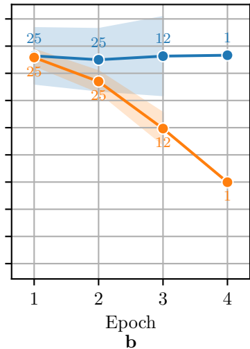
Without subject leakage
