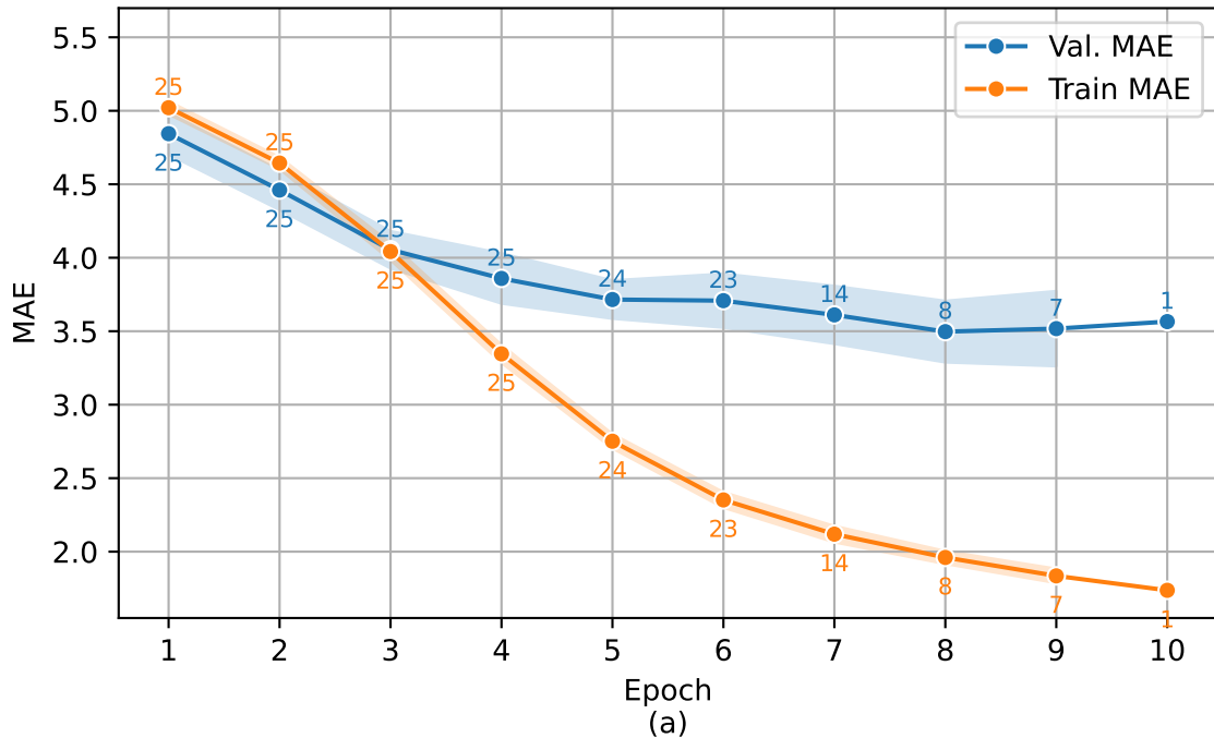
With subject leakage
