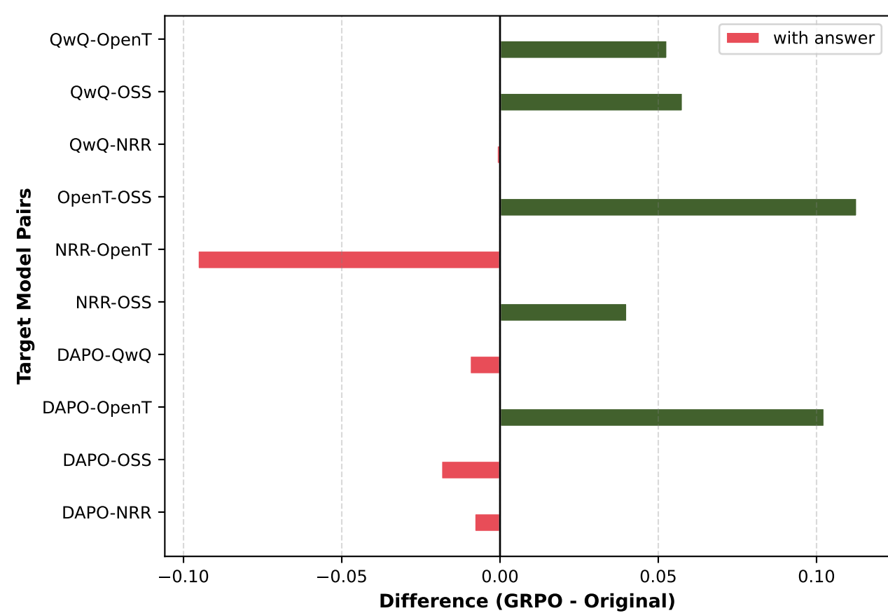
Effect of GRPO Training
