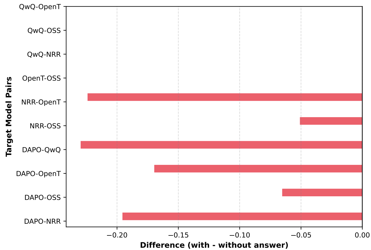
Effect of Including Answer in Thoughts
