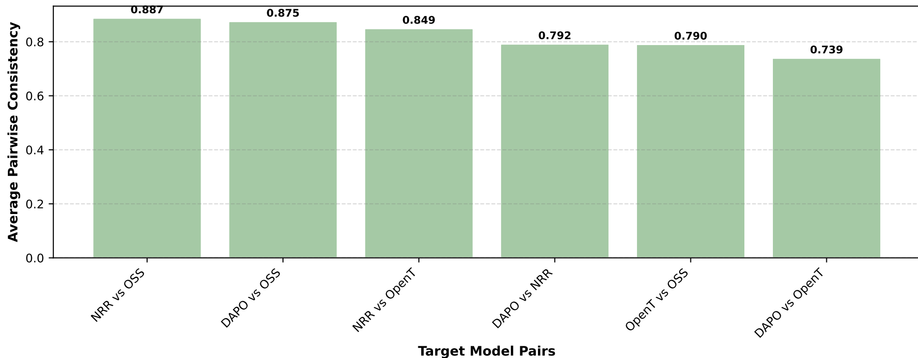
Average Pairwise Consistency Between Target Models
