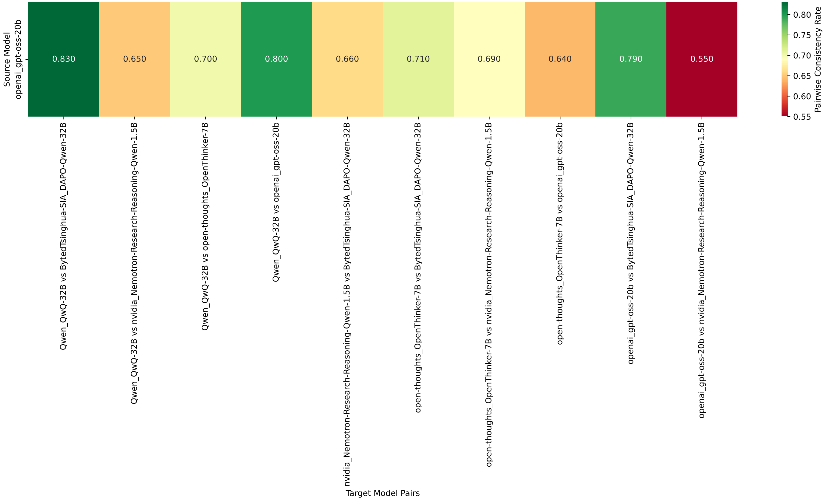
Average Pairwise Consistency Between Target Models
