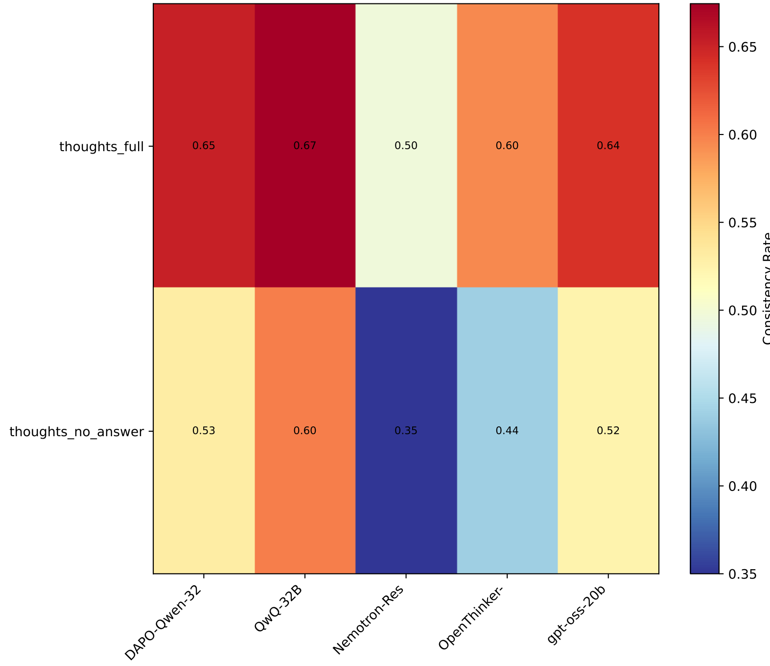
Thoughts Transfer Analysis - Model Performance
