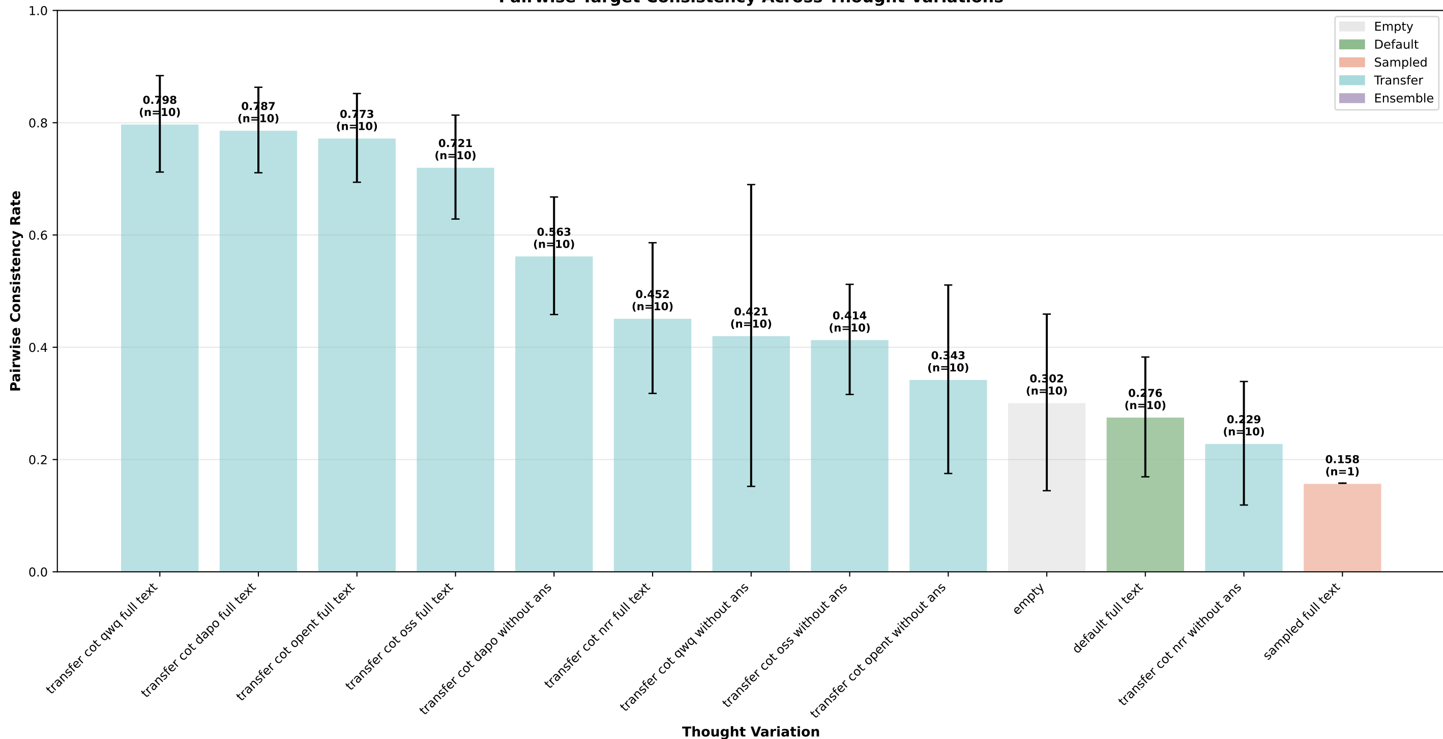
Pairwise Target Consistency Across Thought Variations
