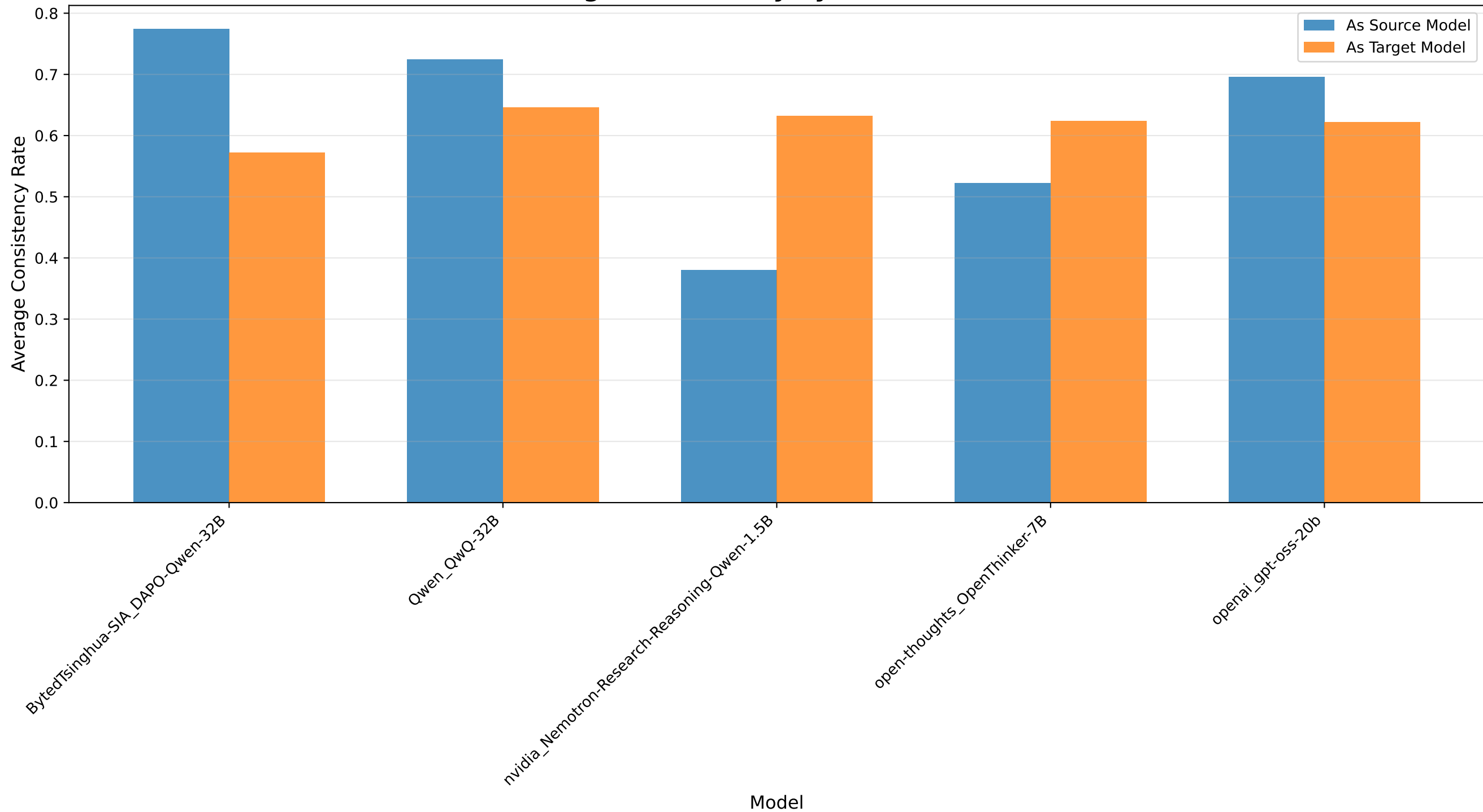
Average Consistency by Model and Role
