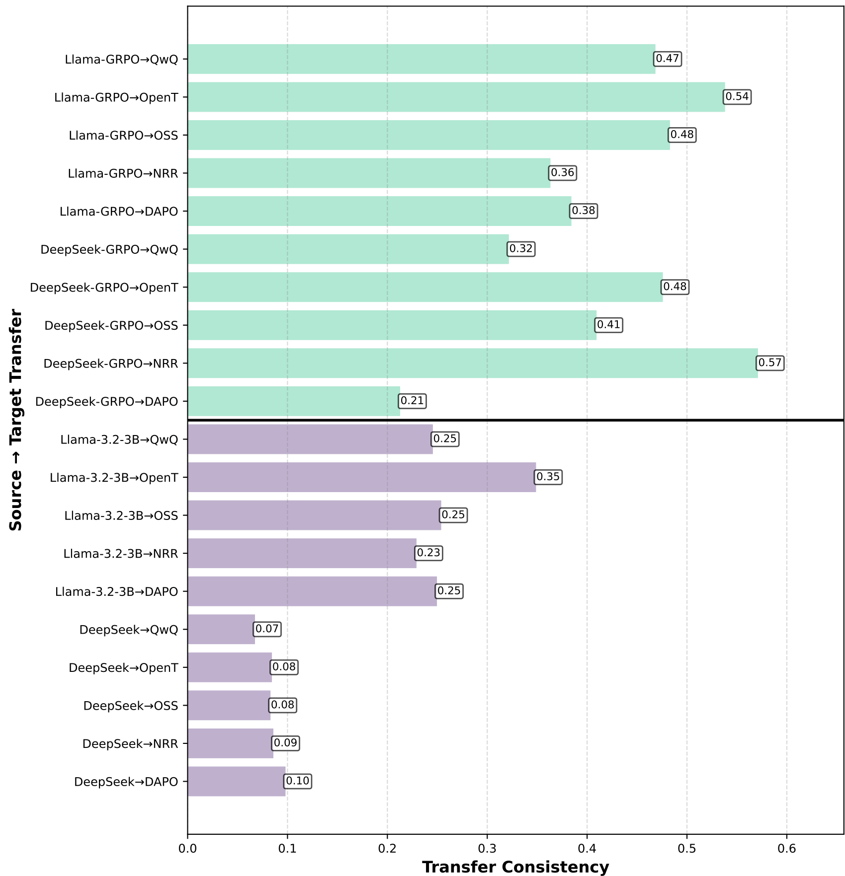
Individual Transfer Consistencies (Without Answer)
