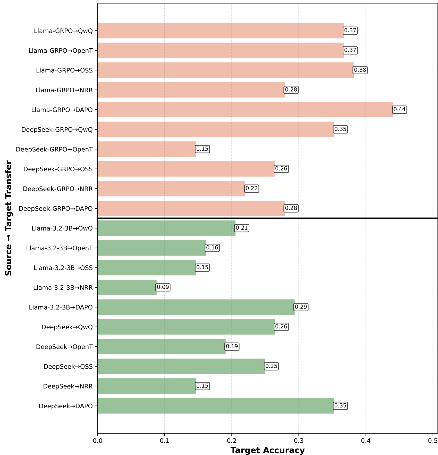
Individual Transfer Accuracies (Without Answer)
