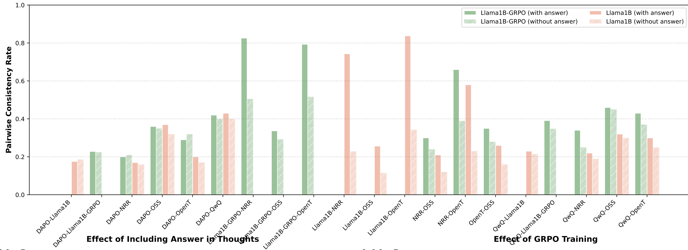
Pairwise Consistency: Source Model × Answer Condition (Including Source Models)
