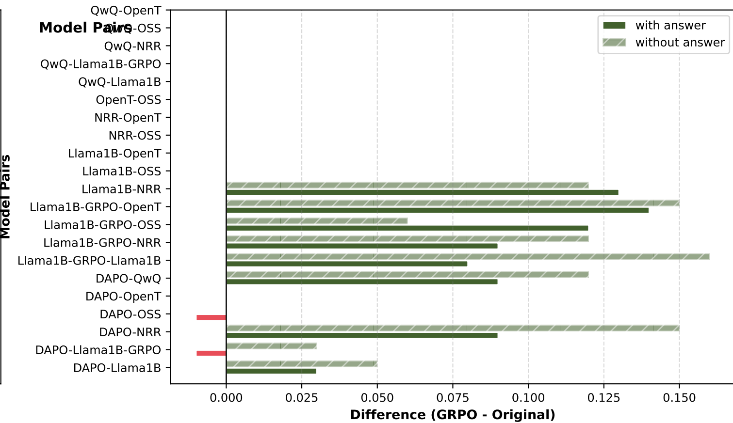
Effect of GRPO Training
