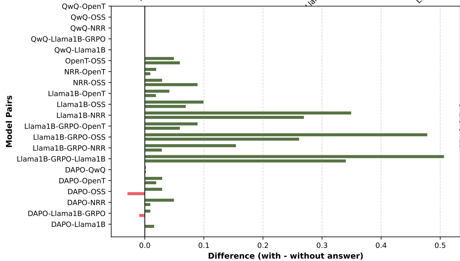
Effect of Including Answer in Thoughts
