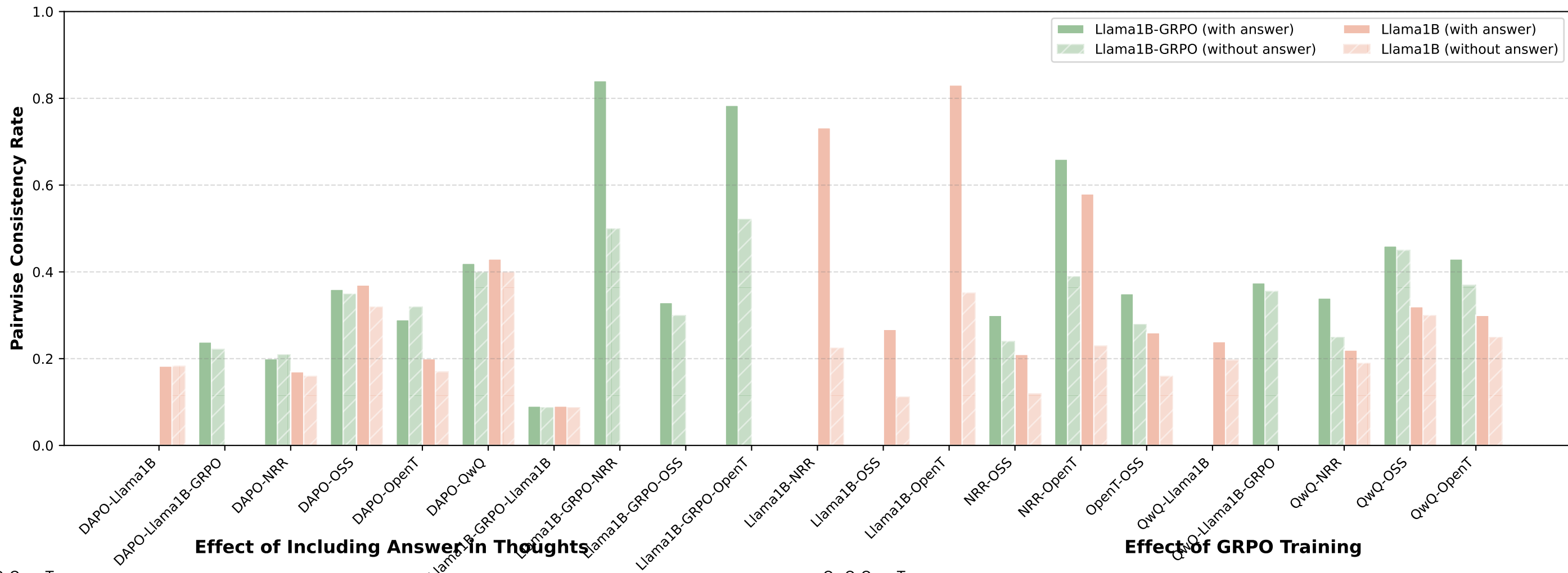
Pairwise Consistency: Source Model × Answer Condition
