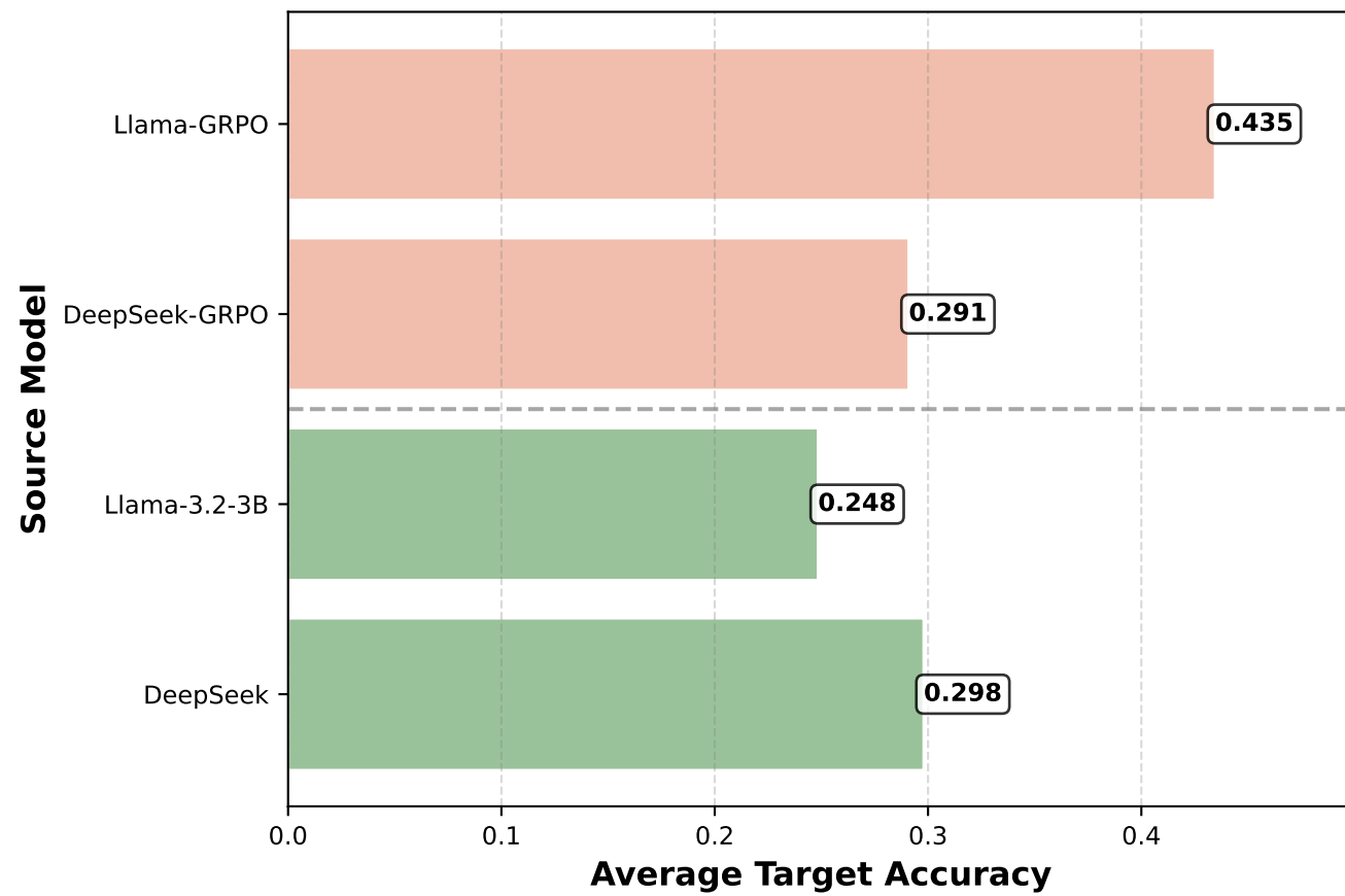
Target Accuracy by Source Model (Without Answer)
