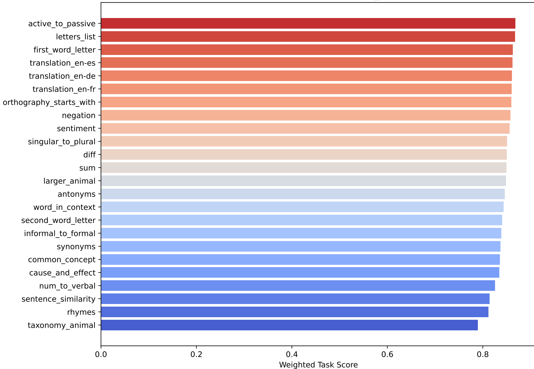
Weighted Scores Across Tasks (openai_gpt-oss-20b)
