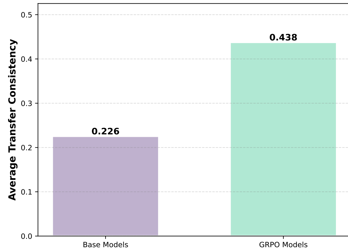
Average Transfer Consistency (With Answer)
