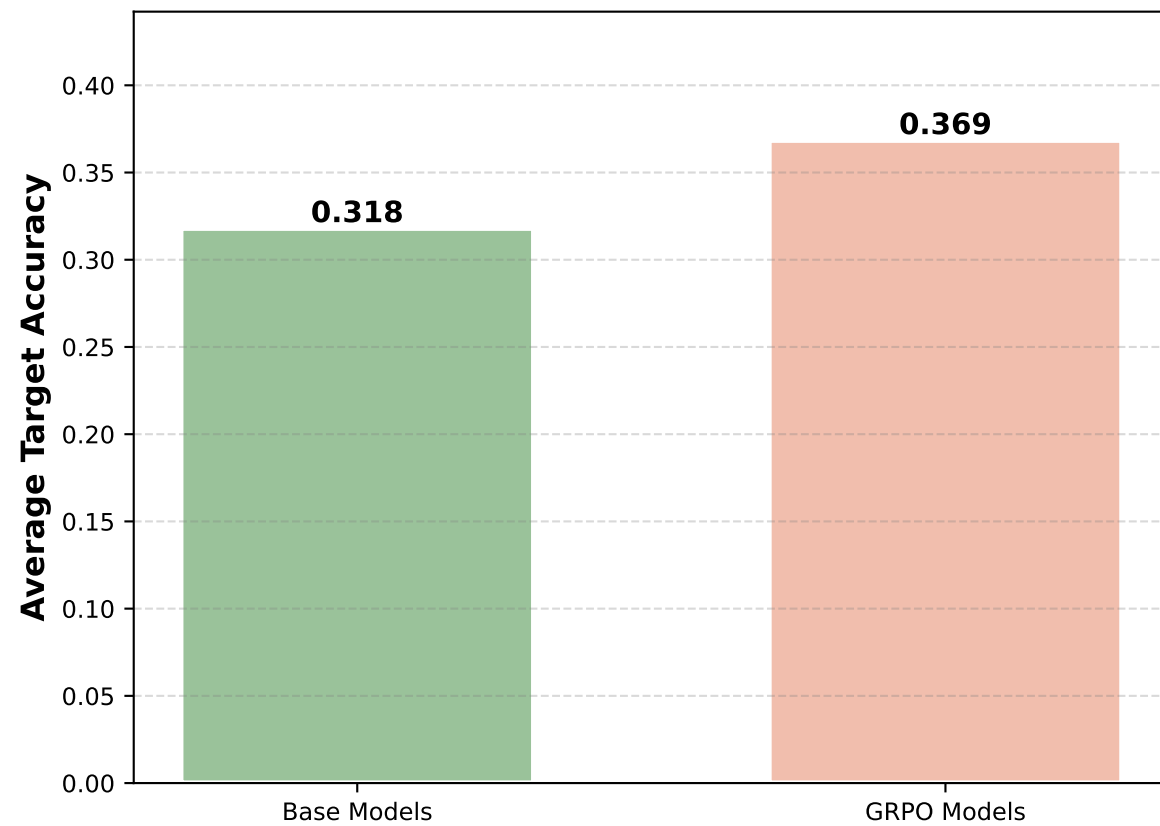
Average Target Accuracy (With Answer)
