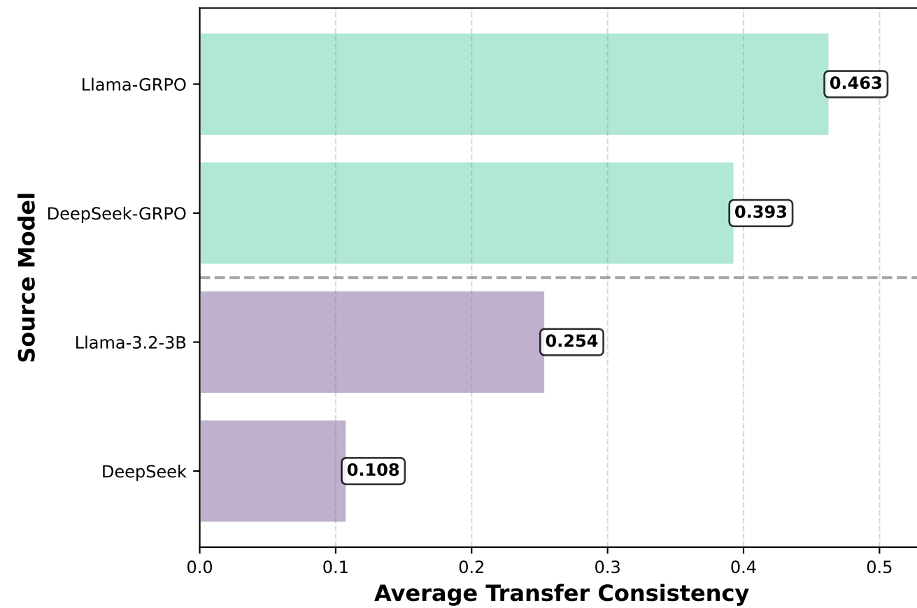
Transfer Consistency by Source Model (Without Answer)
