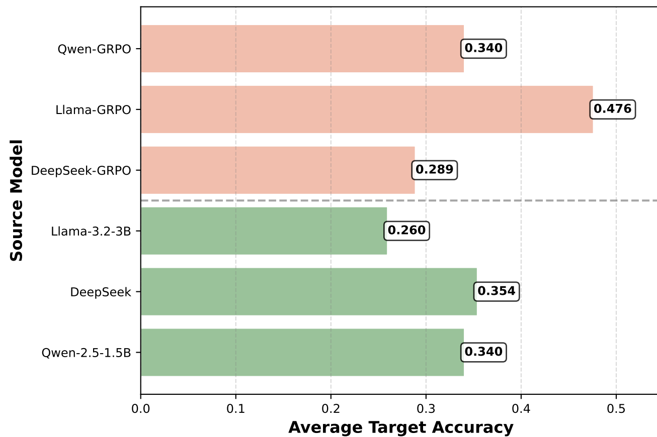
Target Accuracy by Source Model (With Answer)
