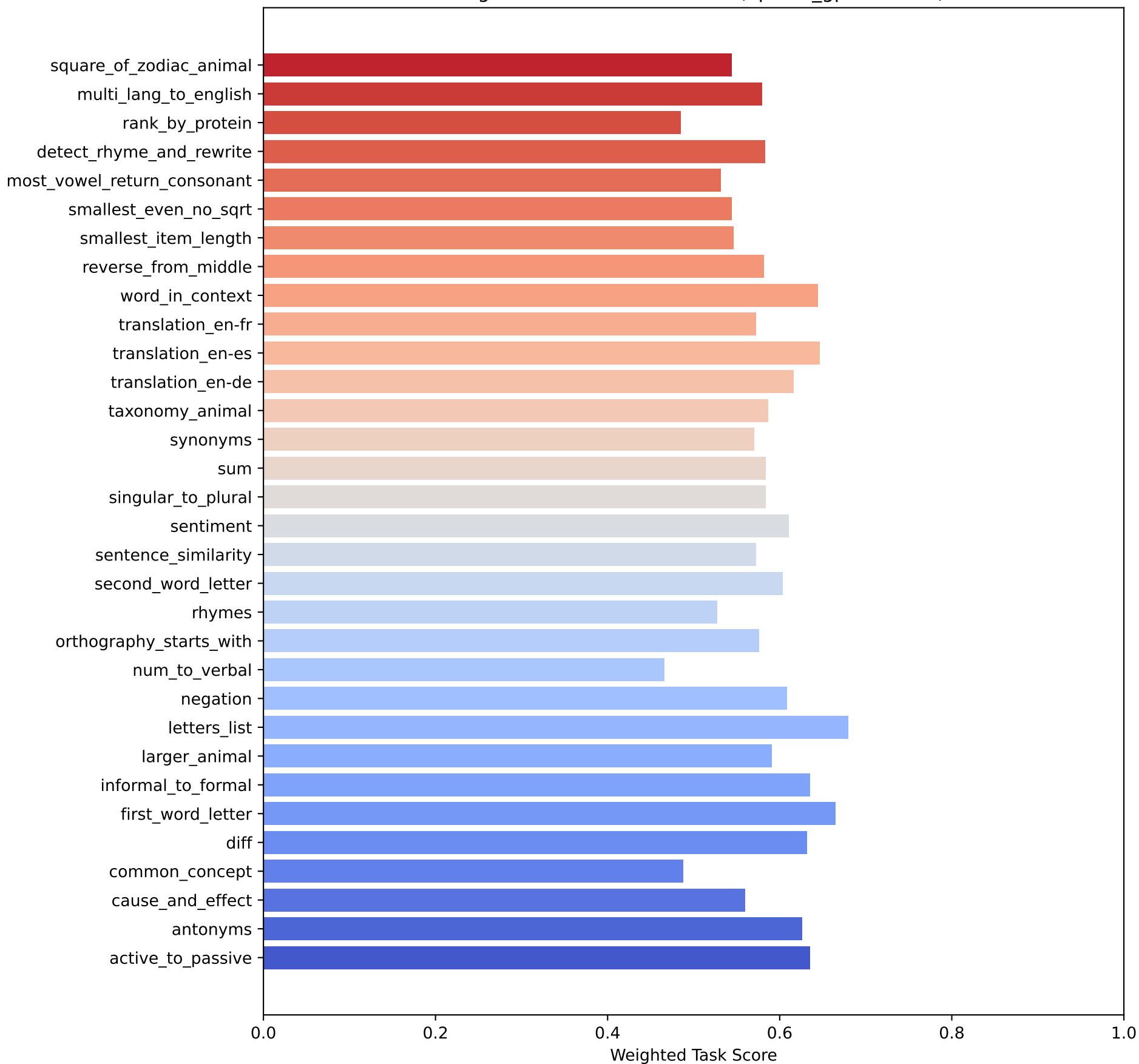
Weighted Scores Across Tasks (openai_gpt-oss-20b)
