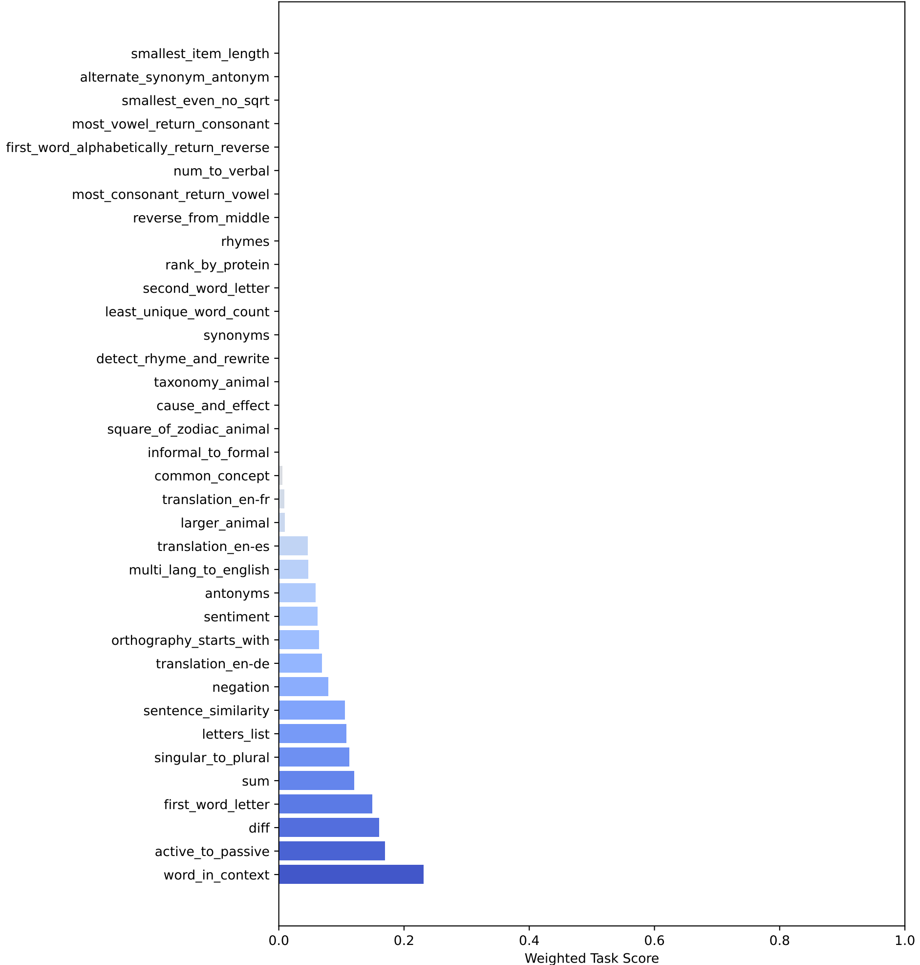
Weighted Scores Across Tasks (open-thoughts_OpenThinker-7B)
