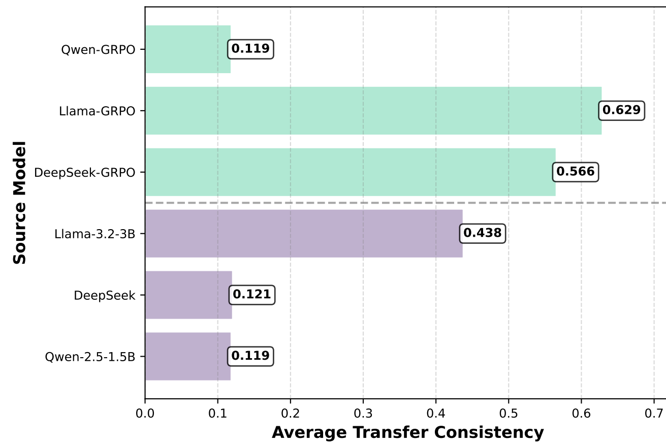
Transfer Consistency by Source Model (With Answer)
