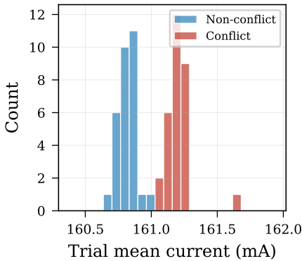
(b) VCCO_PSDDR Burst per-trial
