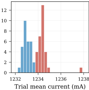
(c) VCCPSINTFP Burst per-trial
