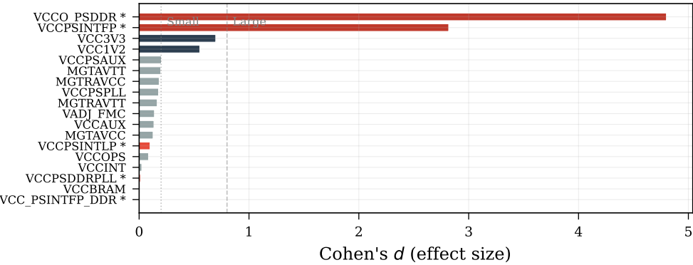
(g) Summary of Discriminability Metrics
