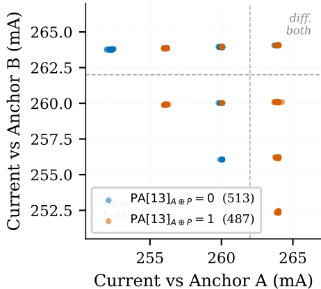
(a) Dual-anchor current plane
