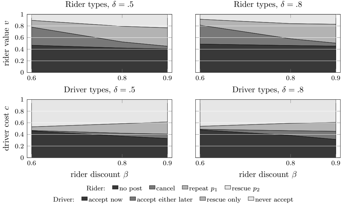
Figure 3: Equilibrium type maps for six optimal active menus. A vertical slice partitions the full type interval [0, 1] ; hence its shaded heights are the uniform-population shares reported above. The vertices are the recomputed calibrations at \beta = .6, .8, .9 and the connecting segments are visual guides, not a continuous comparative-statics claim. Continuation labels describe actions conditional on initial failure, not realized path probabilities.
