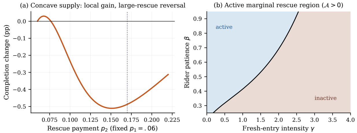
Figure 4 Where the rescue comparison changes sign or becomes inactive. Panel (a) fixes F(c) = \sqrt{c} , G(v) = v , (m, \alpha, \beta, \delta, \gamma) = (.5, .75, .3, 1, 0) , and p_1 = .06 ; the dotted line marks p_2 = .17 . The plotted value is the conservative minimum across numerical cutoff roots. Panel (b) plots \mathcal{A}_{\alpha, \gamma}(p) at m = 5 , p = .2 , and \alpha = .6 ; the blue region satisfies the strict activity condition.
