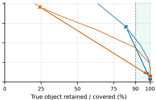
Downstream-query coverage
