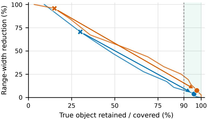
Matching-set retention
