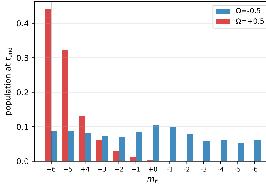
(e) spin distribution at end — Barnett pumping
