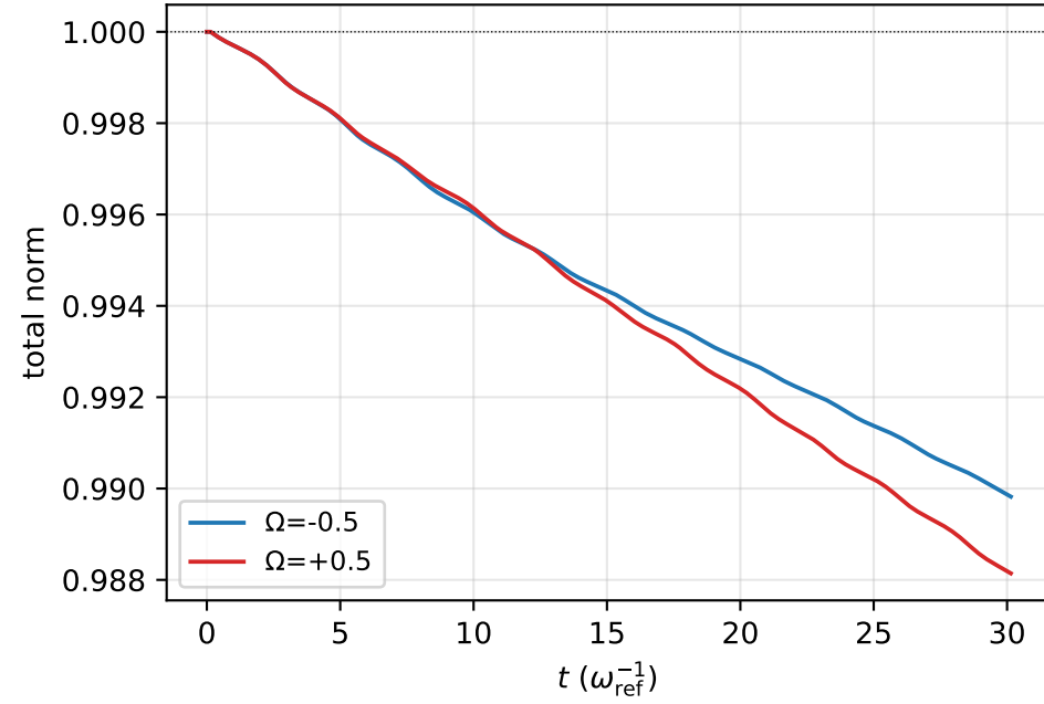
(a) atom-number decay
