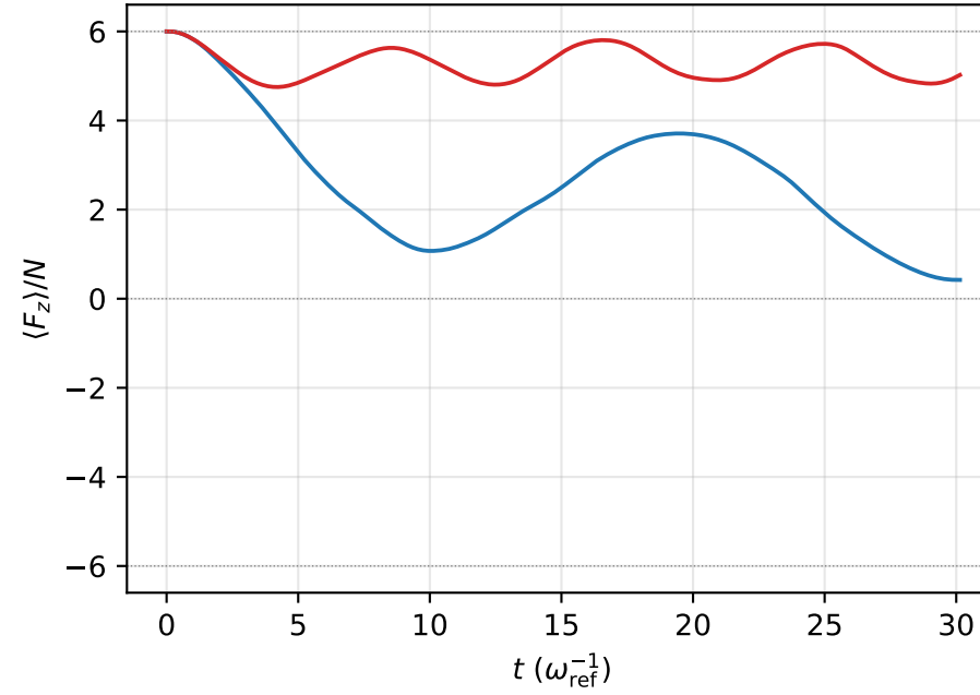
(b) Barnett pumping — headline
