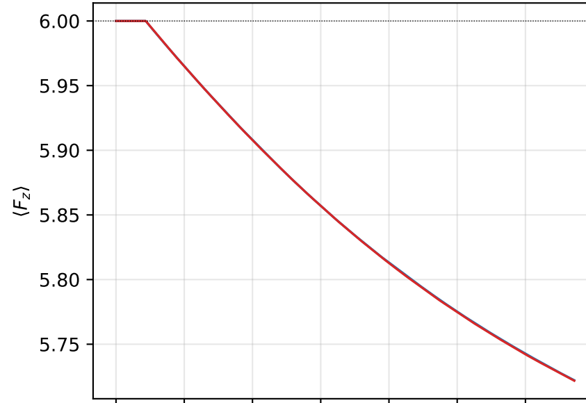
(b) Barnett pumping signature
