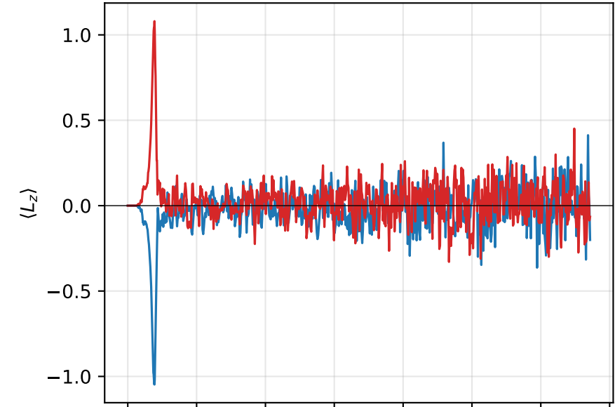
(c) orbital response (sign-flipped \pm\phi )
