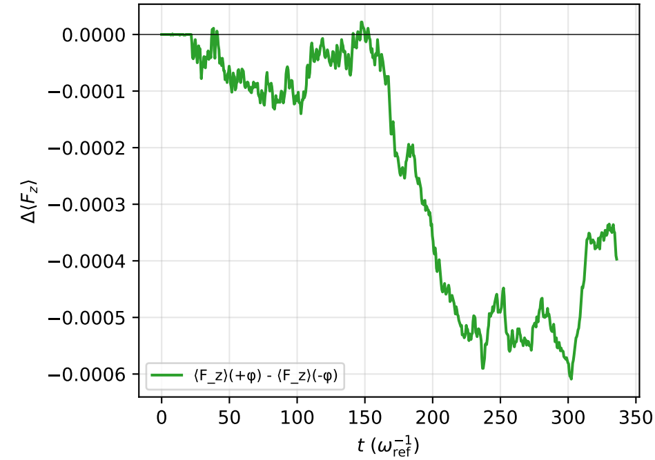
(f) Barnett antisymmetry — headline
