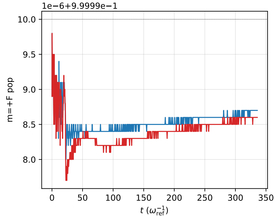
(e) m = +F population (spinor unfreezing)
