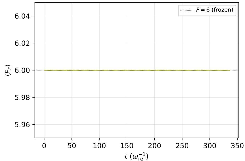
(b) spin sector frozen (no loss channel)
