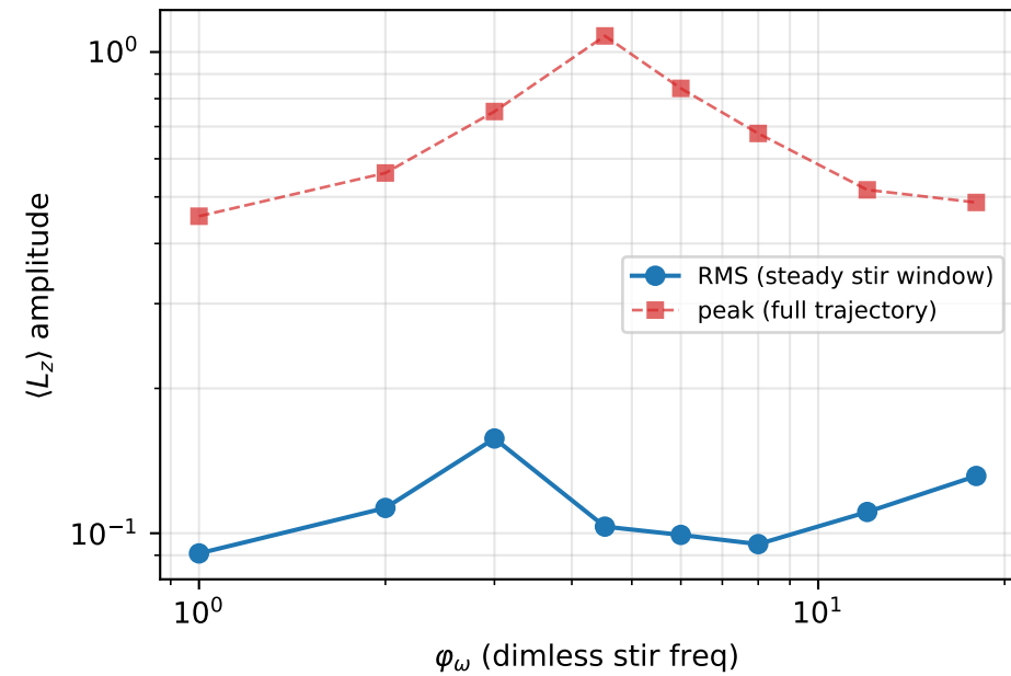
(c) orbital response scaling
