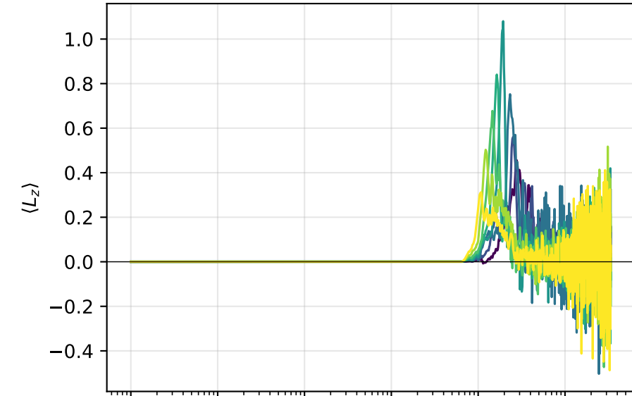
(c) orbital response (Klaus signature)
