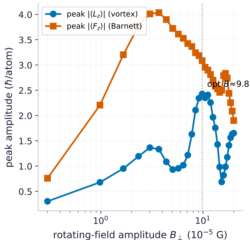
(b) vs rotating-field B_{\perp} ( \Omega=0.5 )
