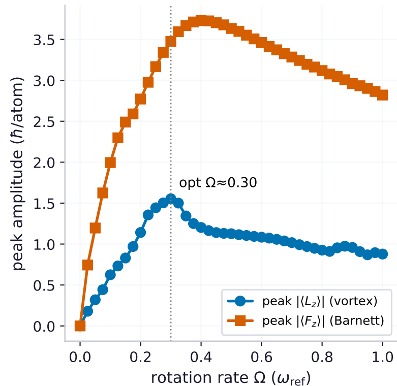
(a) vs rotation strength \Omega
