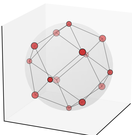
F=11 octa O:A 2 (supp) — 22 stars on 14 sites (mixed mult.)
