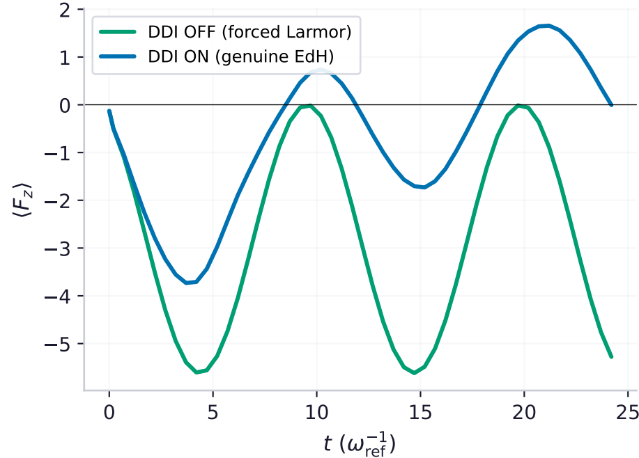
(b) \langle F_z \rangle (spin along rotation axis)
