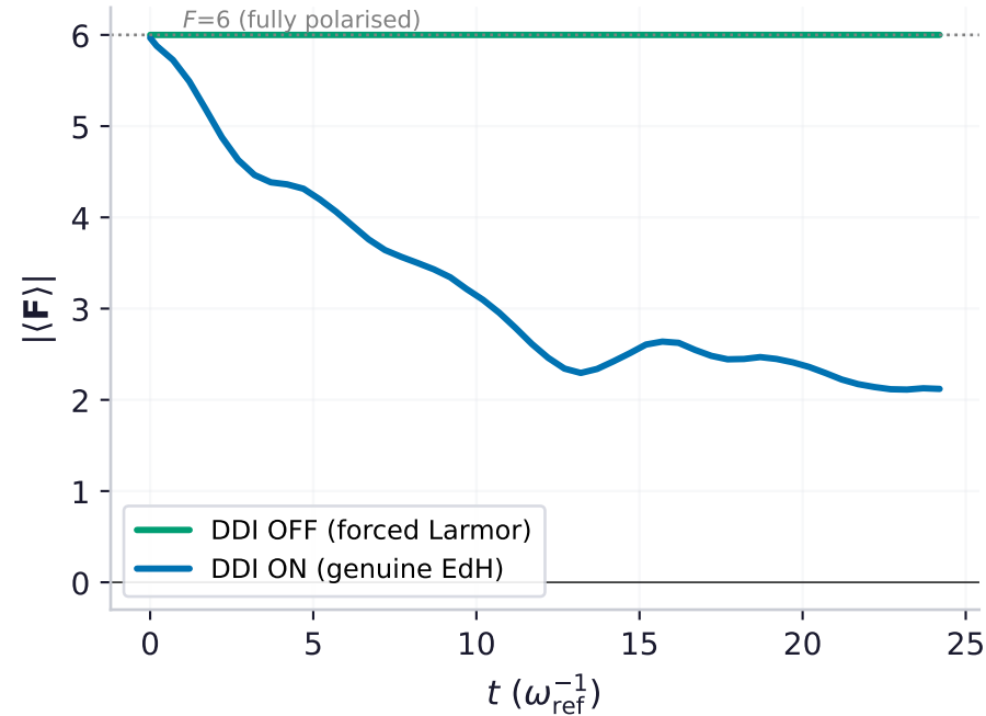
(a) spin length |\langle F \rangle|
