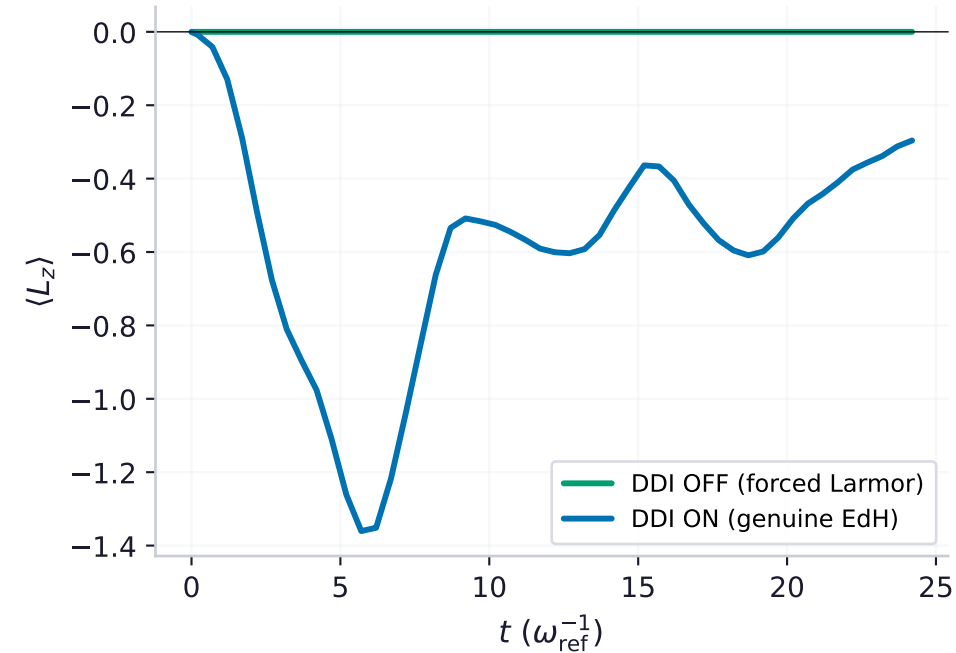
(c) \langle L_z \rangle (vortices) — 0 without DDI
