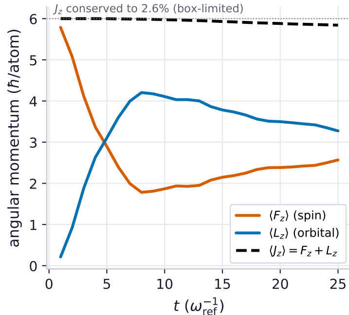
(b) Einstein-de Haas: spin \rightarrow orbital, J_z conserved
