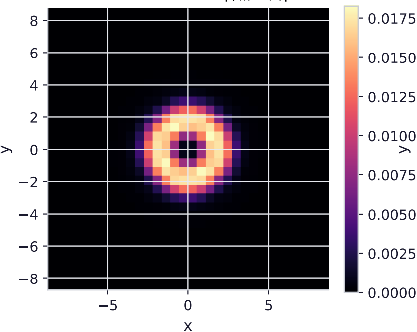
(e) transferred |\psi_{m=+4}|^2
