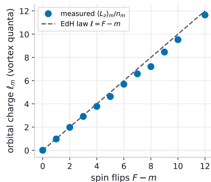
(c) quantised vortices: \ell_m = F - m
