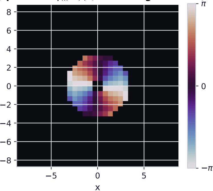
(f) phase of \psi_{m=+4} ( 2\pi winding = vortex)
