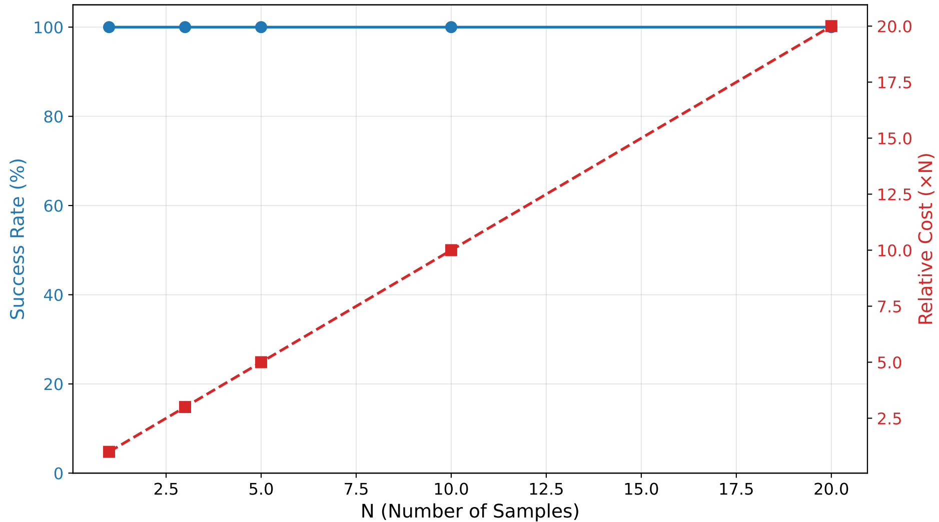
Best-of-N: Cost-Performance Trade-off
