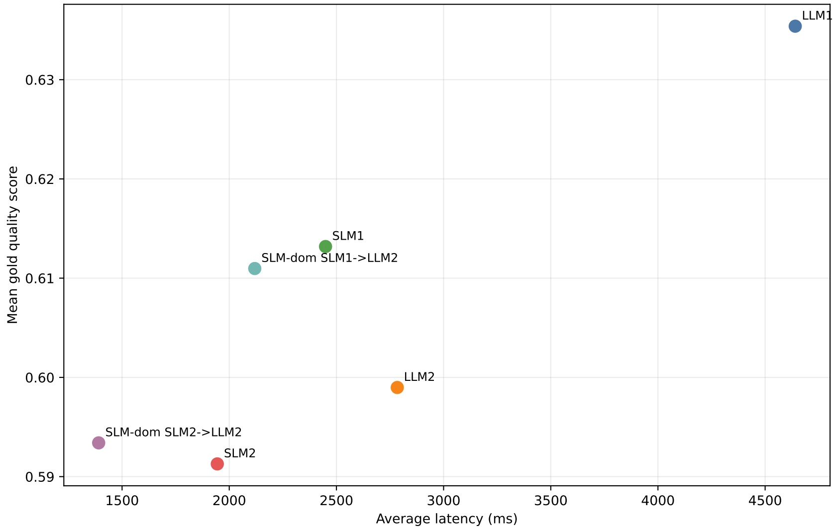
Gold Resolution Quality vs Latency
