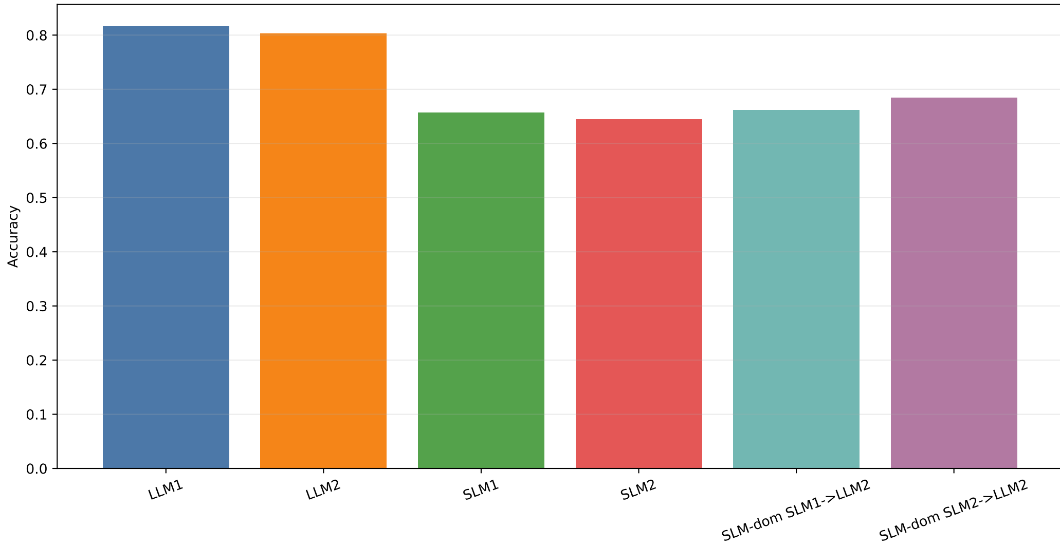
Generated Category Accuracy by Config
