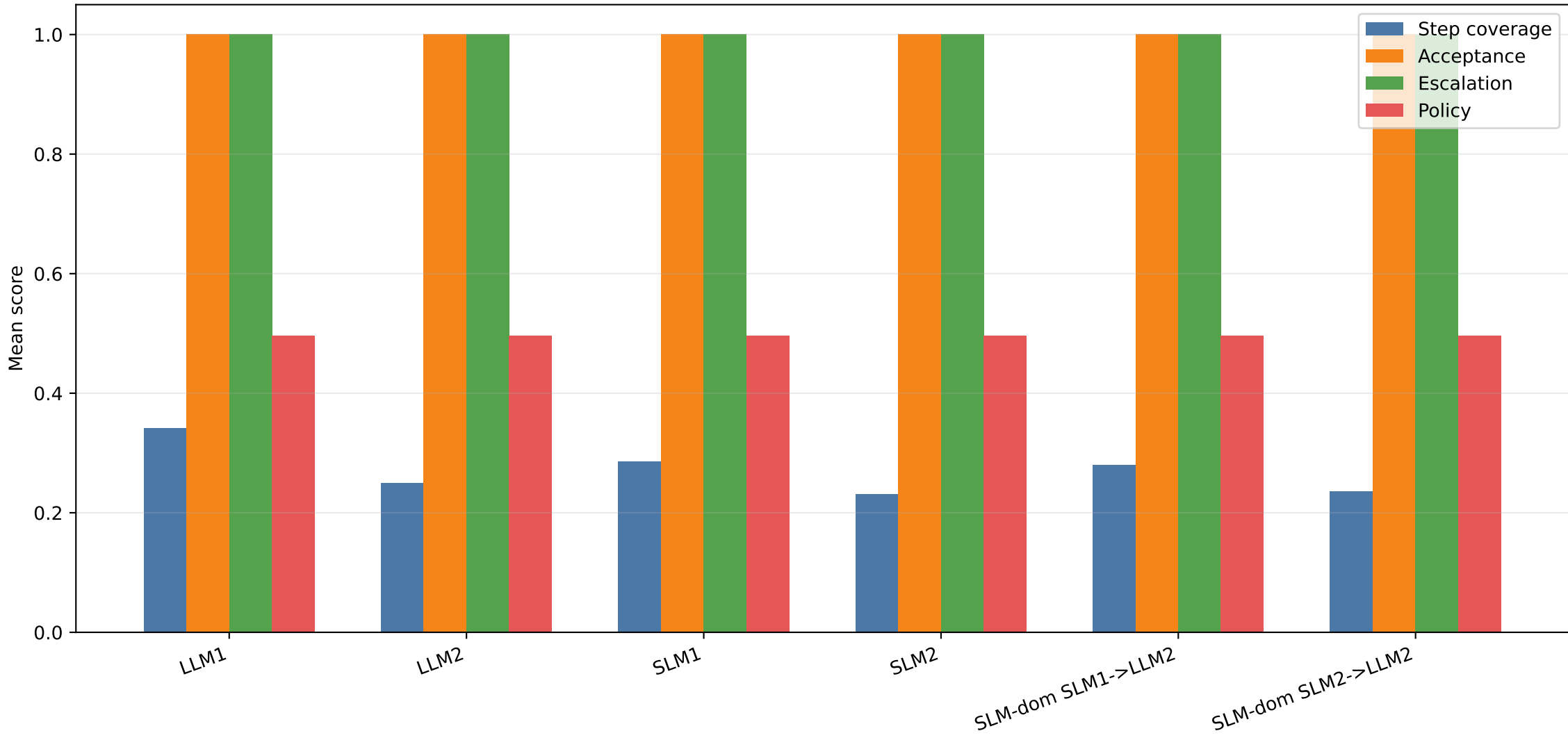
Gold Resolution Component Scores by Config
