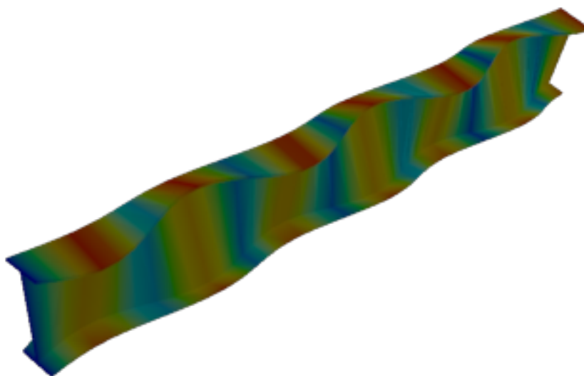
Figure 43: Code_Aster — mode 10, 160.681 Hz
