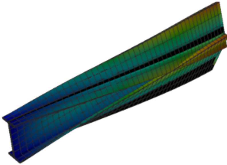
Figure 517: Code_Aster — mode 6, 130.809 Hz
