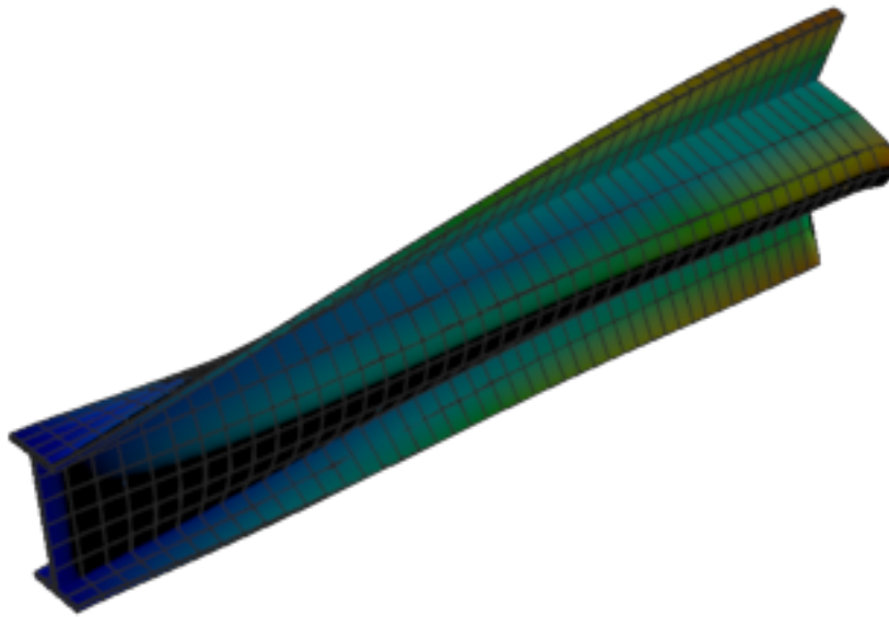
Figure 280: Calculix — mode 6, 125.257 Hz
