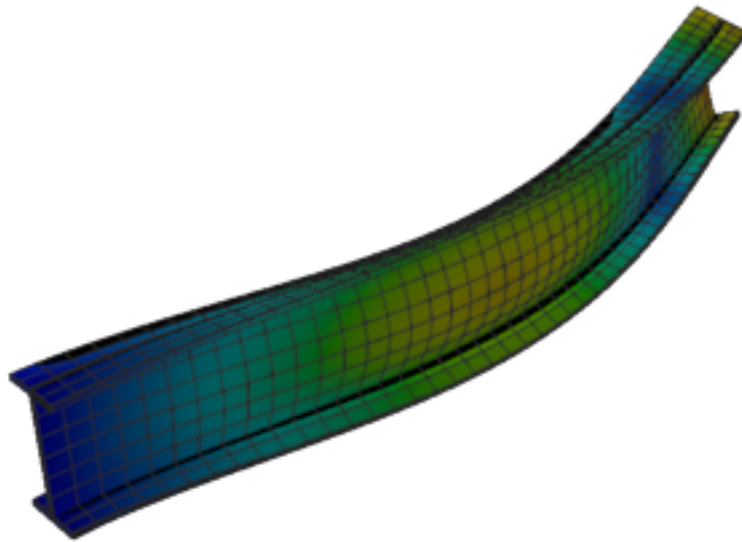
Figure 471: Sesam — mode 4, 76.747 Hz
