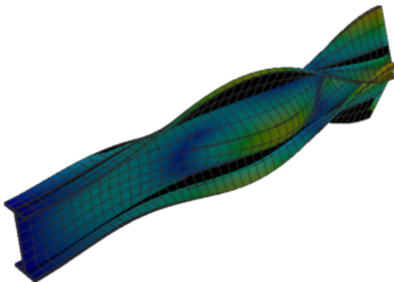
Figure 485: Calculix — mode 8, 173.925 Hz
