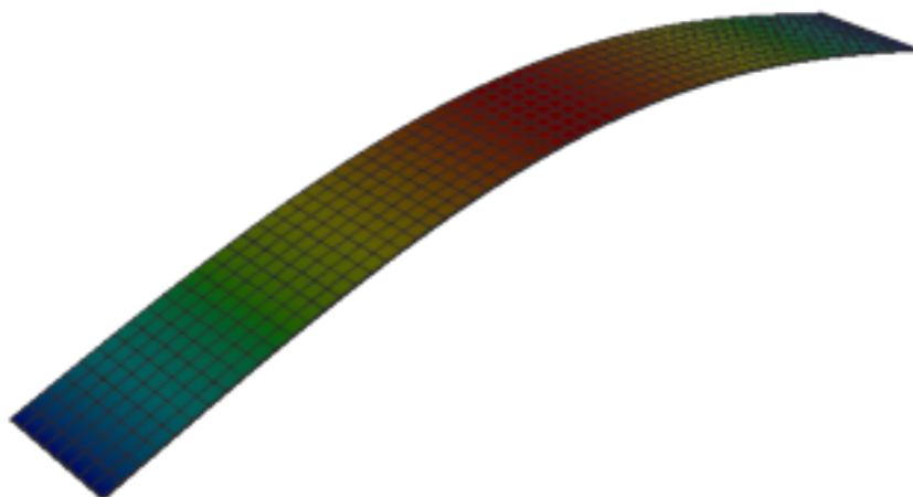
Figure 533: Abaqus — mode 1, 1.537 Hz
