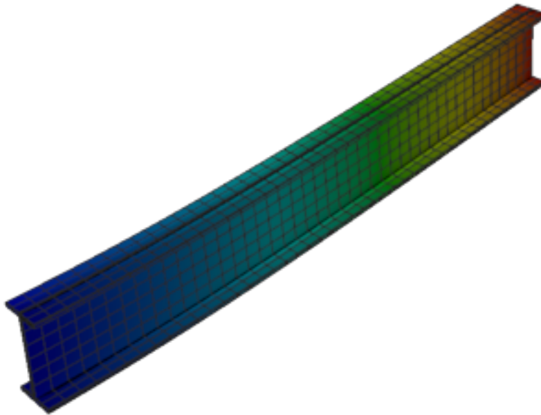
Figure 506: Abaqus — mode 3, 50.498 Hz
