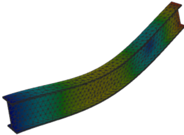
Figure 309: Code_Aster — mode 5, 261.806 Hz
