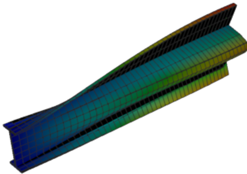
Figure 396: Code_Aster — mode 6, 147.139 Hz
