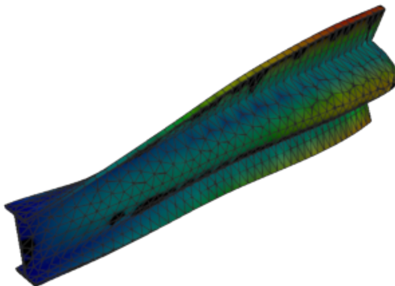
Figure 106: Calculix — mode 9, 304.464 Hz
