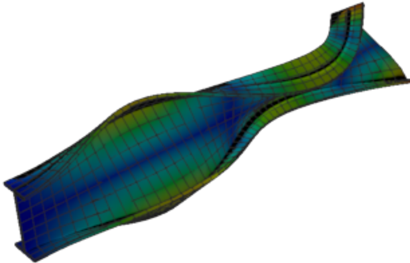
Figure 378: Sesam — mode 11, 256.050 Hz
