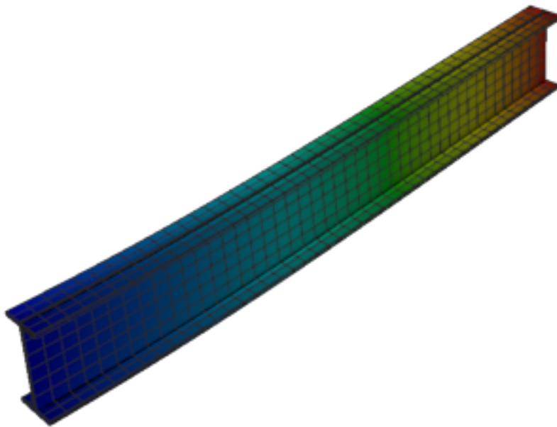
Figure 508: Code_Aster — mode 3, 50.498 Hz
