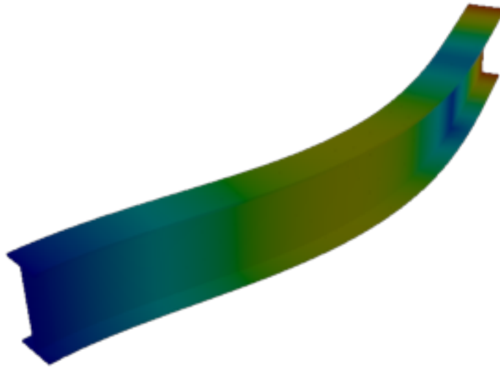
Figure 71: Sesam — mode 6, 65.327 Hz
