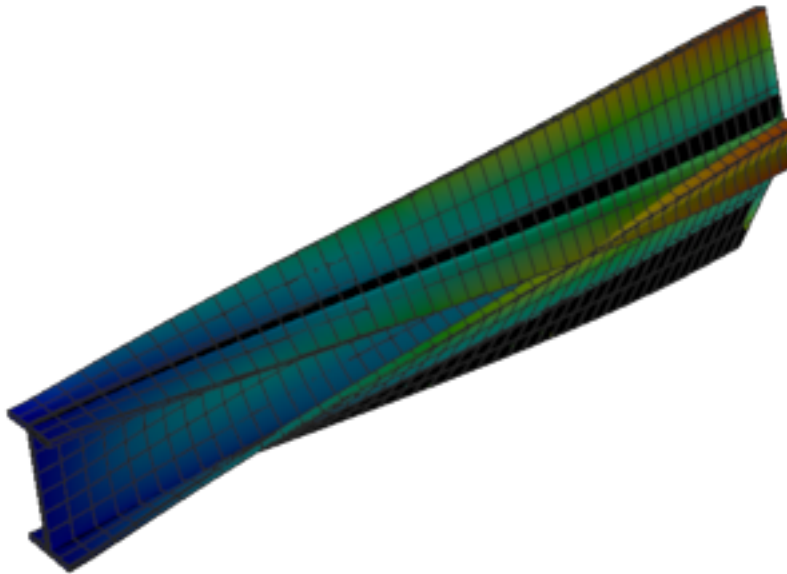
Figure 476: Abaqus — mode 6, 131.365 Hz
