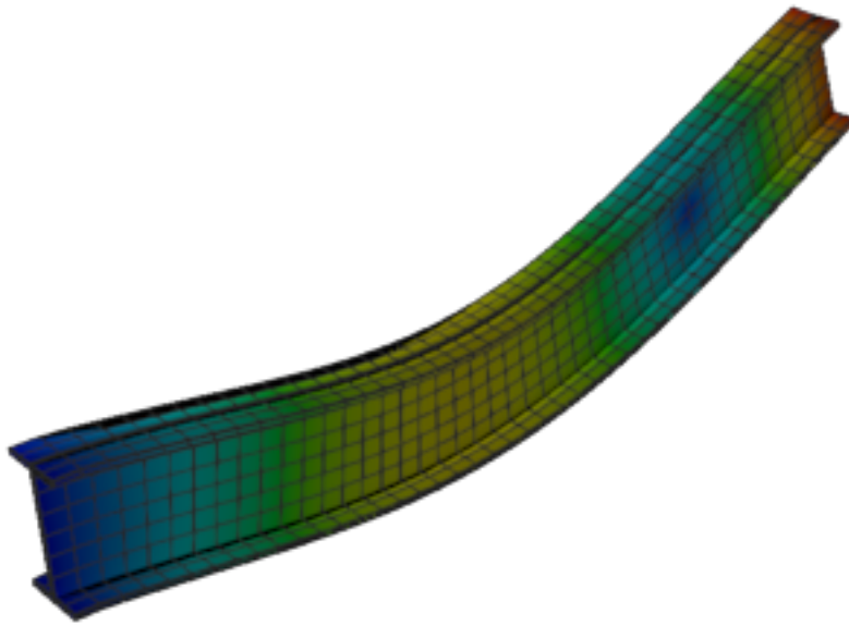
Figure 361: Code_Aster — mode 7, 255.872 Hz
