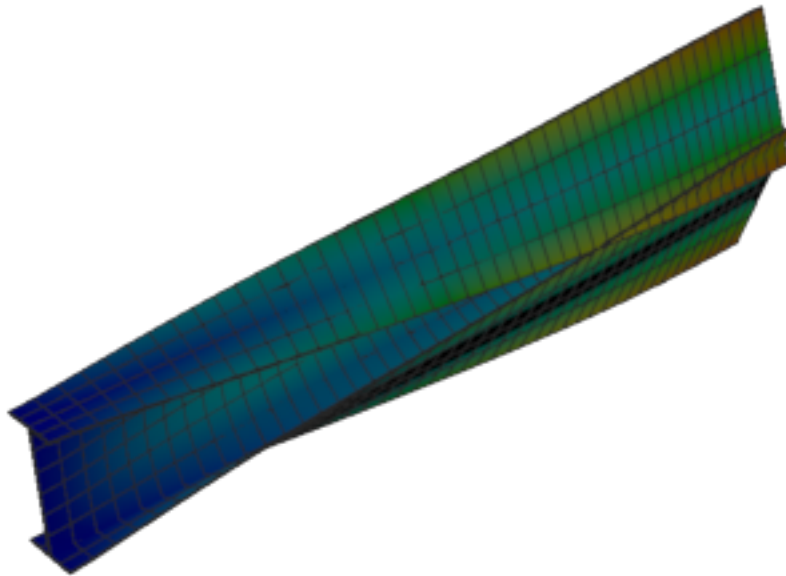
Figure 135: Abaqus — mode 6, 126.961 Hz
