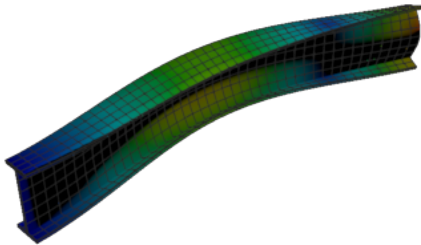
Figure 276: Calculix — mode 4, 75.140 Hz
