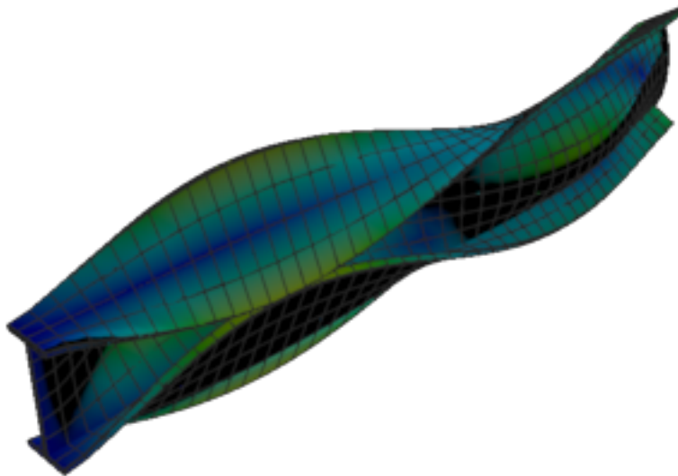
Figure 282: Calculix — mode 7, 142.497 Hz
