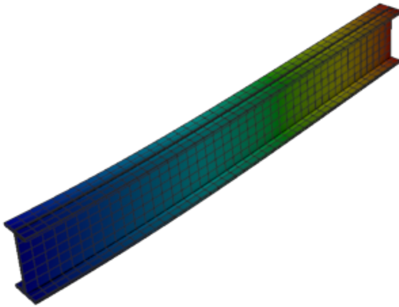
Figure 467: Sesam — mode 3, 50.534 Hz
