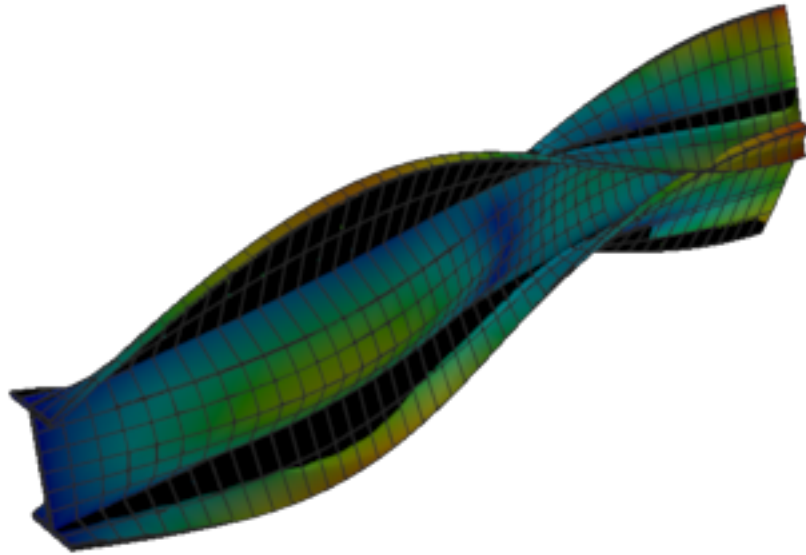
Figure 403: Abaqus — mode 9, 155.992 Hz
