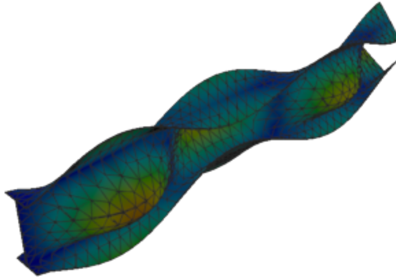
Figure 216: Sesam — mode 9, 193.308 Hz
