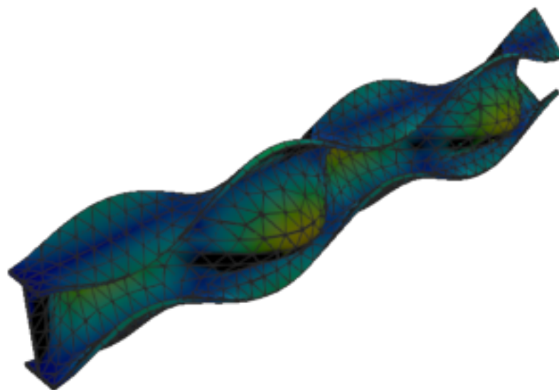
Figure 218: Calculix — mode 10, 236.042 Hz
