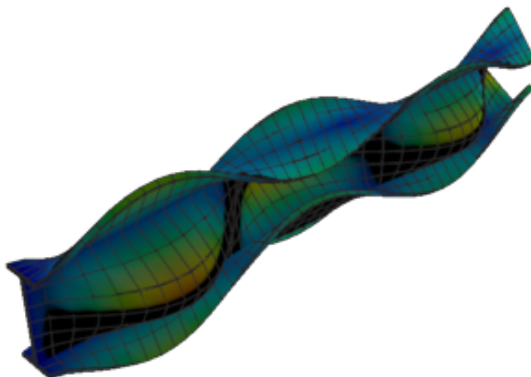
Figure 148: Calculix — mode 9, 200.495 Hz
