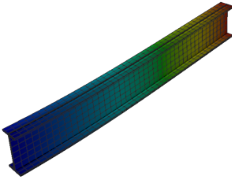
Figure 507: Calculix — mode 3, 50.498 Hz
