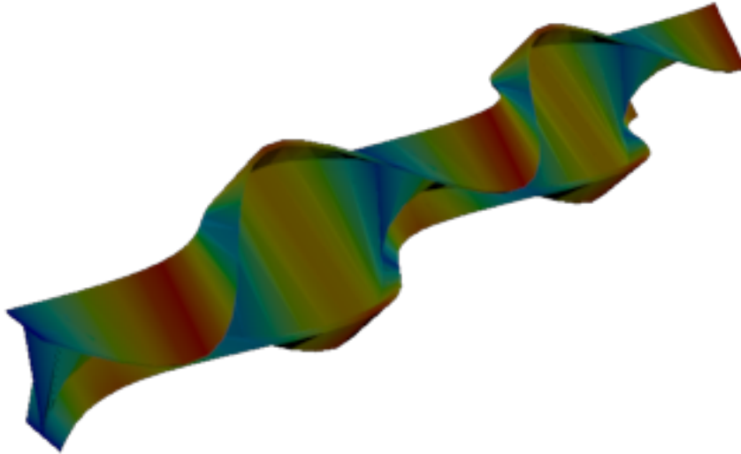
Figure 36: Sesam — mode 8, 110.699 Hz
