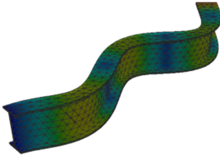
Figure 326: Sesam — mode 9, 503.862 Hz
