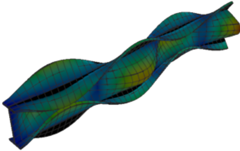
Figure 489: Calculix — mode 9, 205.292 Hz
