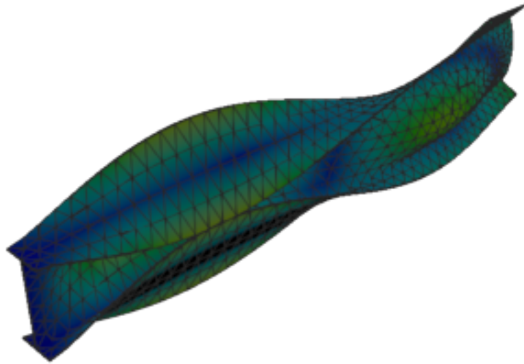
Figure 205: Abaqus — mode 7, 142.773 Hz
