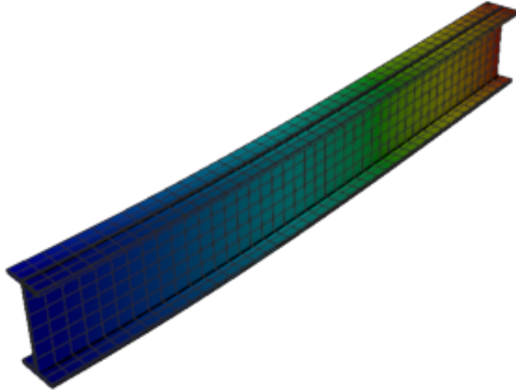
Figure 459: Sesam — mode 1, 12.954 Hz
