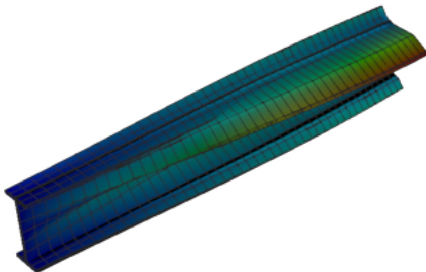
Figure 409: Abaqus — mode 11, 162.557 Hz
