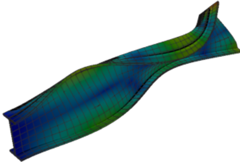
Figure 408: Code_Aster — mode 10, 282.888 Hz
