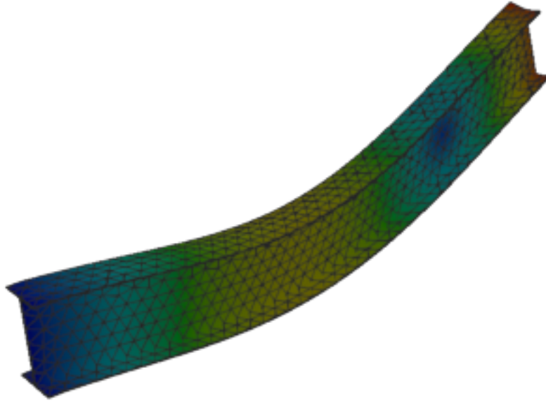
Figure 114: Sesam — mode 11, 257.362 Hz
