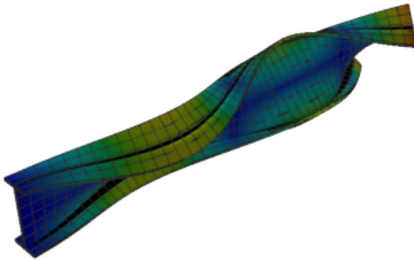
Figure 364: Calculix — mode 8, 266.519 Hz
