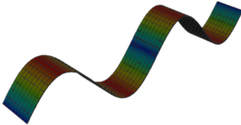
Figure 548: Sesam — mode 4, 24.586 Hz
