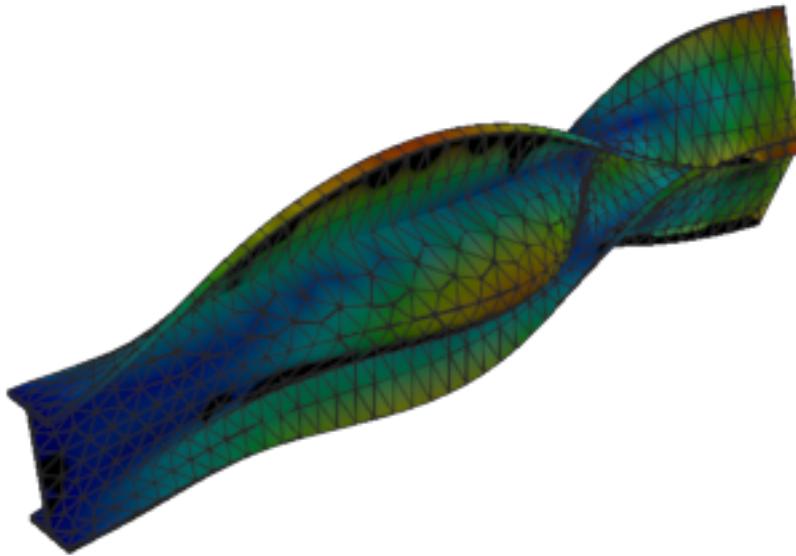
Figure 109: Calculix — mode 10, 365.943 Hz
