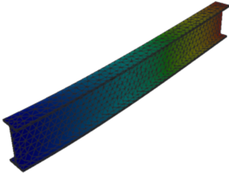
Figure 293: Code_Aster — mode 1, 15.928 Hz
