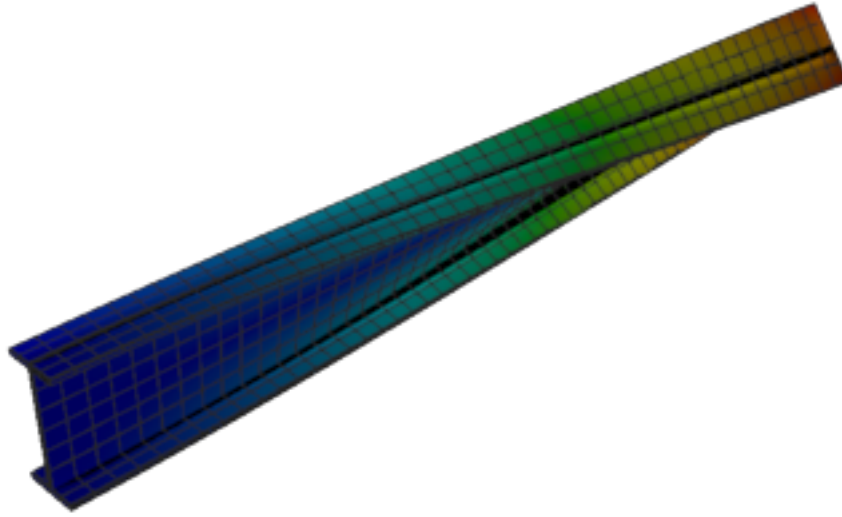
Figure 461: Calculix — mode 2, 20.150 Hz
