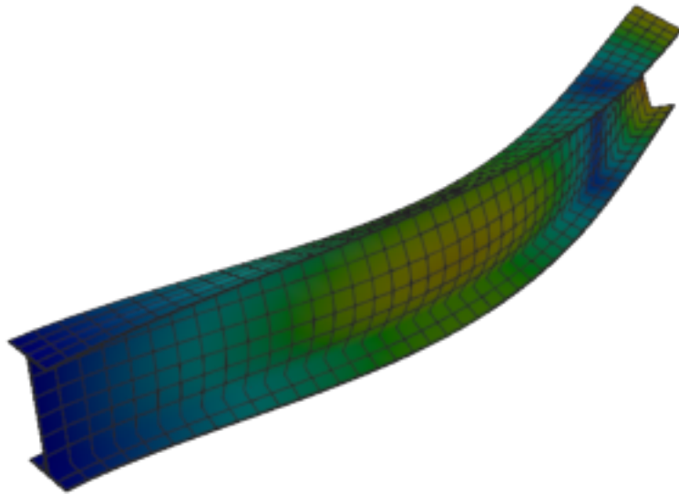
Figure 237: Abaqus — mode 4, 75.149 Hz
