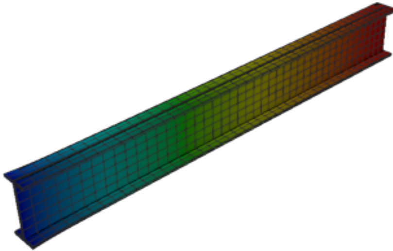
Figure 401: Calculix — mode 8, 431.955 Hz
