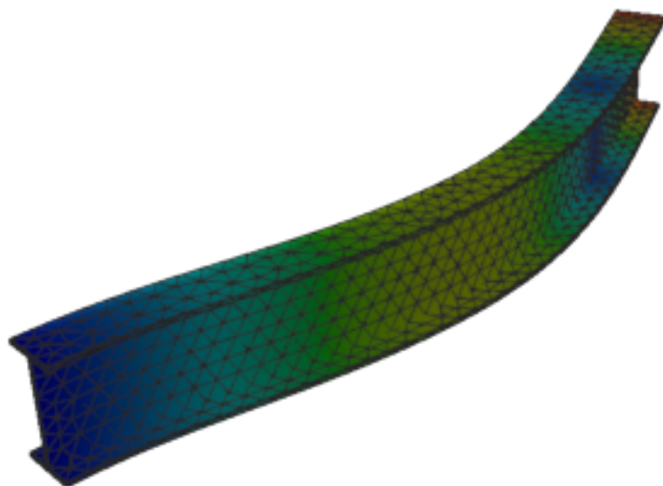
Figure 299: Abaqus — mode 3, 97.588 Hz
