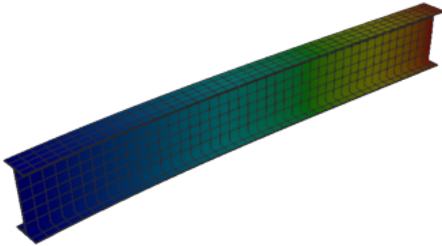
Figure 228: Sesam — mode 1, 12.755 Hz
