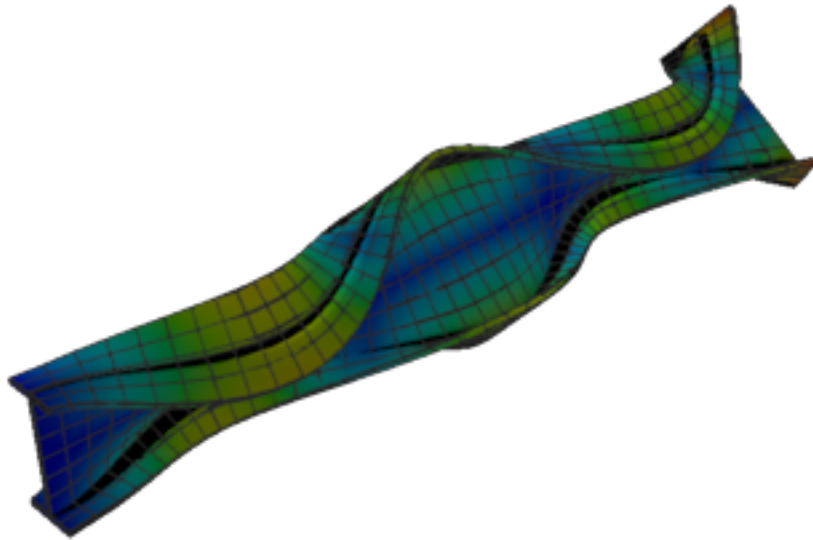
Figure 375: Abaqus — mode 11, 486.965 Hz
