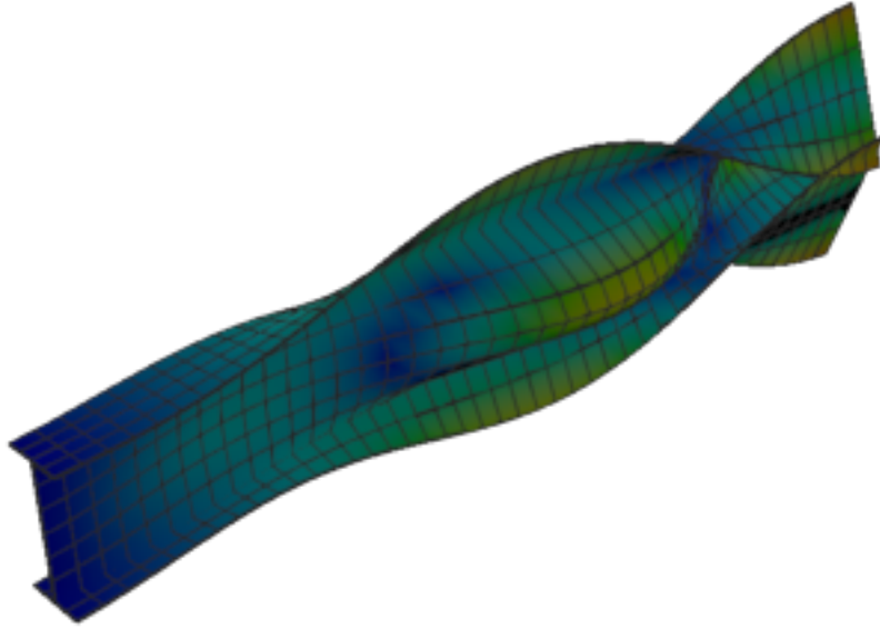
Figure 146: Sesam — mode 8, 165.030 Hz
