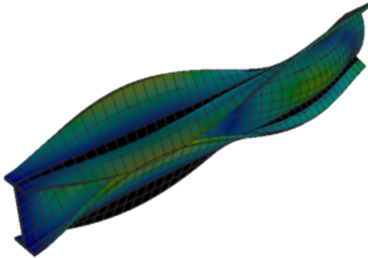
Figure 519: Calculix — mode 7, 148.478 Hz
