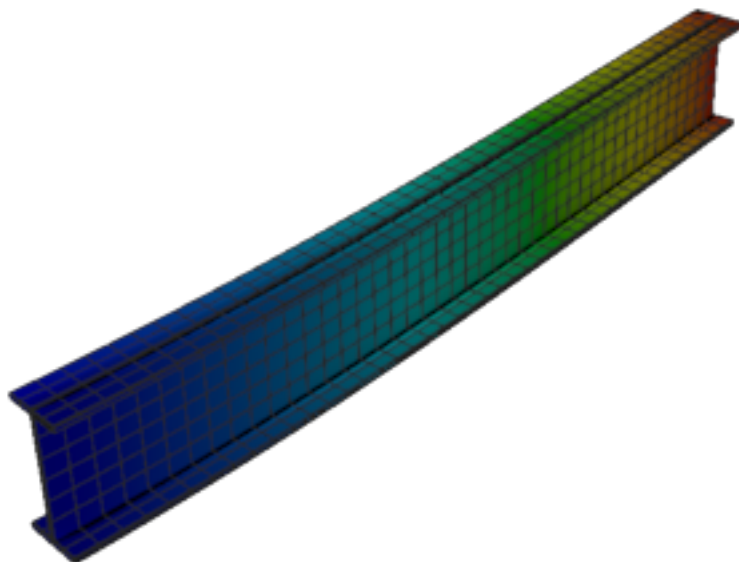
Figure 457: Calculix — mode 1, 12.955 Hz
