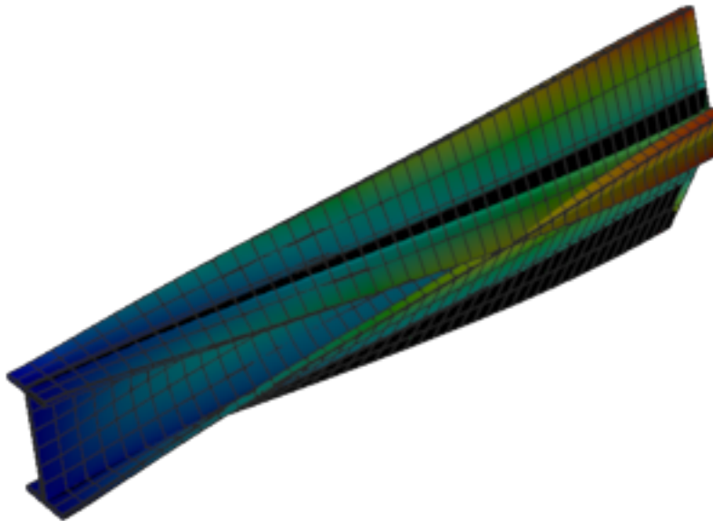
Figure 358: Sesam — mode 6, 133.016 Hz
