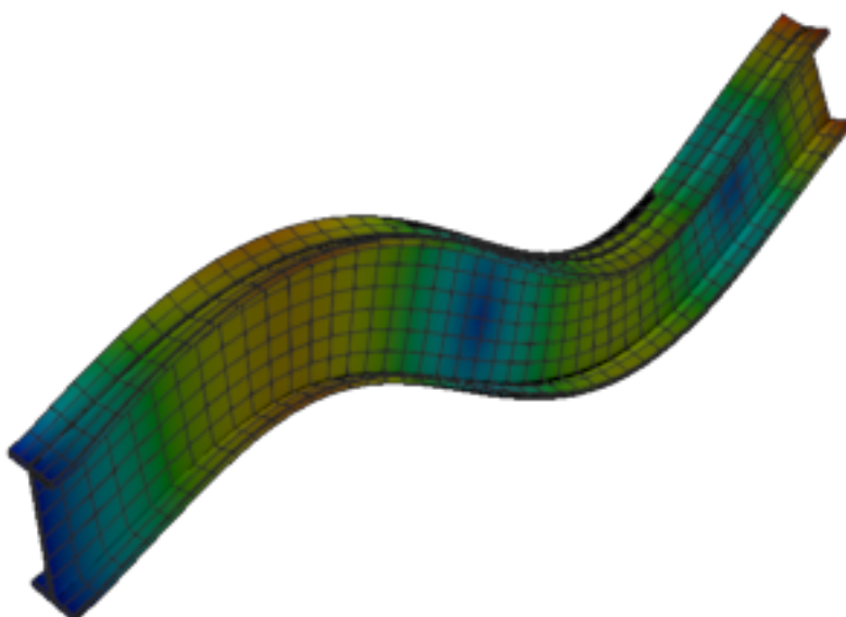
Figure 410: Calculix — mode 11, 582.562 Hz
