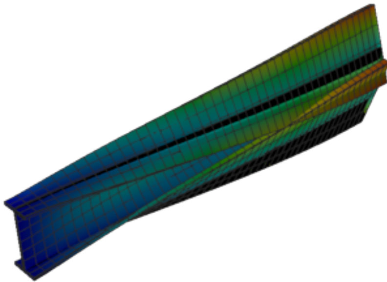
Figure 478: Code_Aster — mode 6, 131.365 Hz
