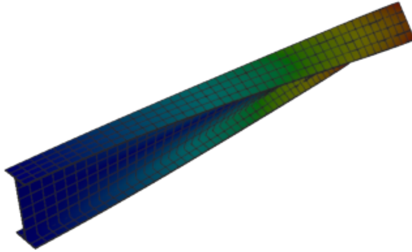
Figure 122: Sesam — mode 2, 19.394 Hz
