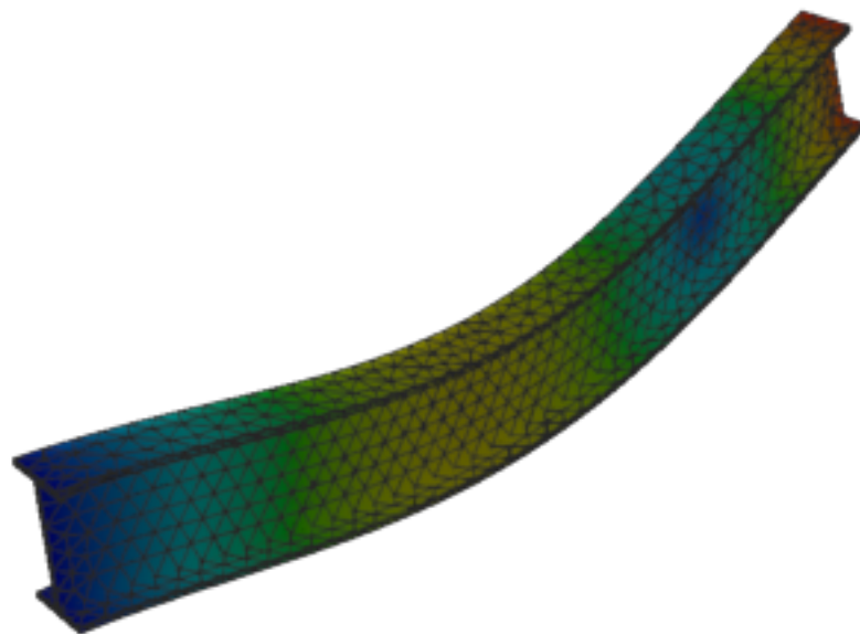
Figure 310: Sesam — mode 5, 260.887 Hz
