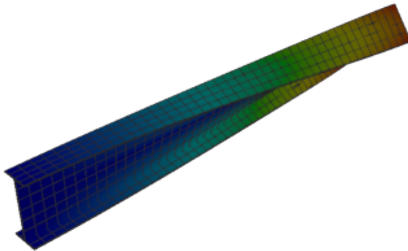
Figure 121: Code_Aster — mode 2, 19.972 Hz
