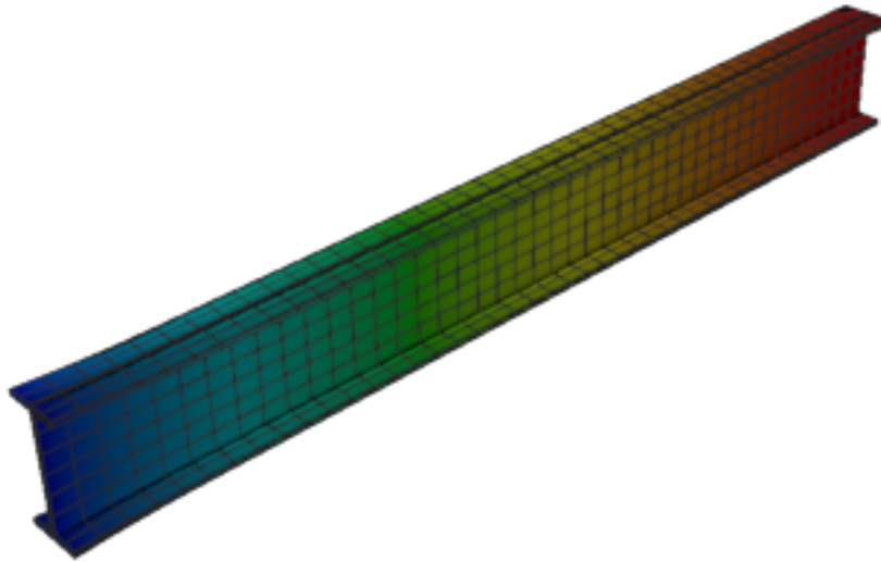
Figure 373: Code_Aster — mode 10, 432.207 Hz
