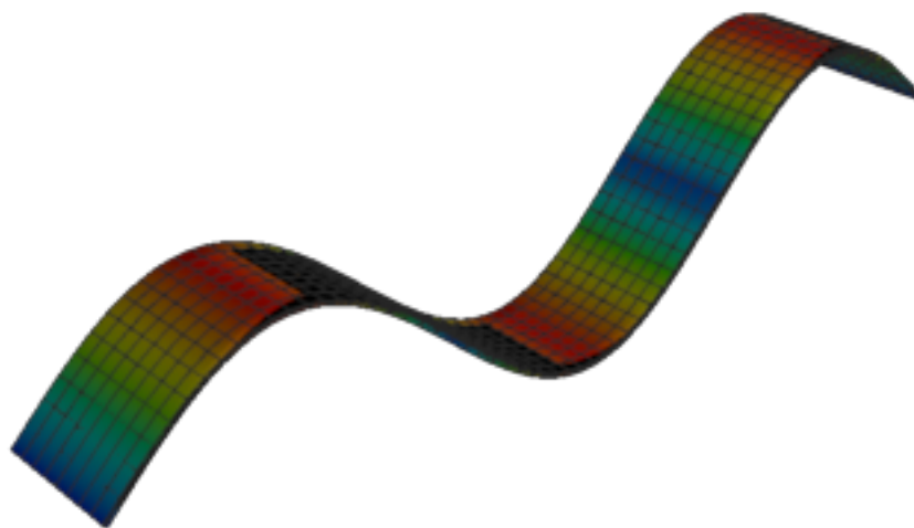
Figure 542: Calculix — mode 3, 13.840 Hz
