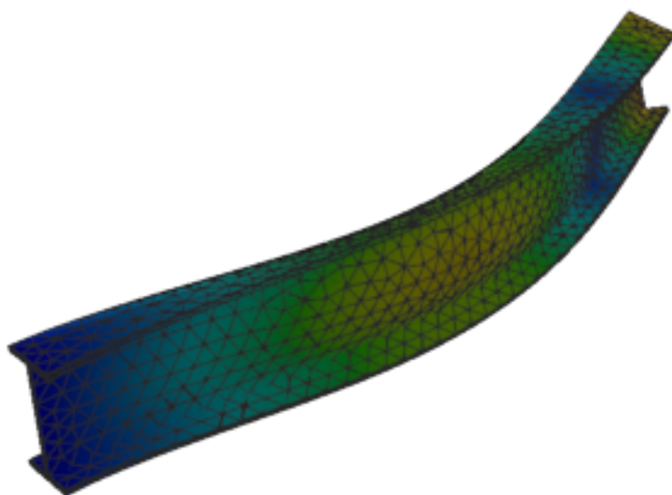
Figure 426: Code_Aster — mode 4, 77.230 Hz
