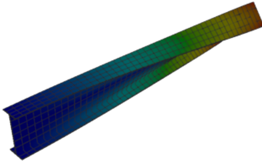
Figure 119: Abaqus — mode 2, 19.593 Hz
