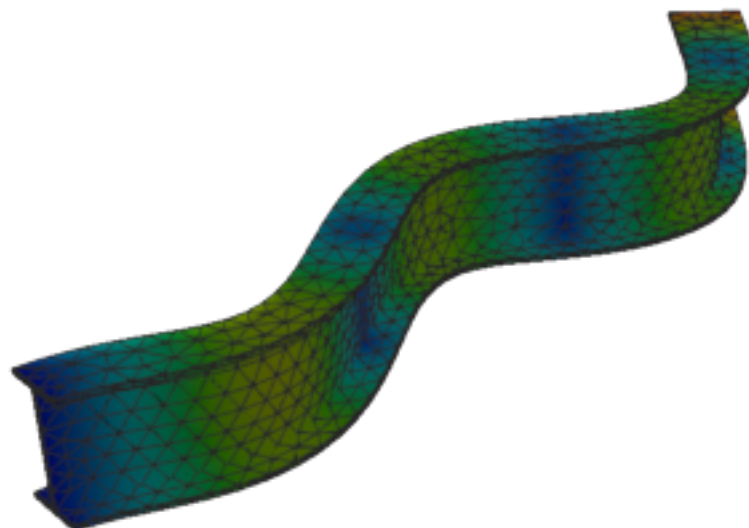
Figure 324: Calculix — mode 9, 529.297 Hz
