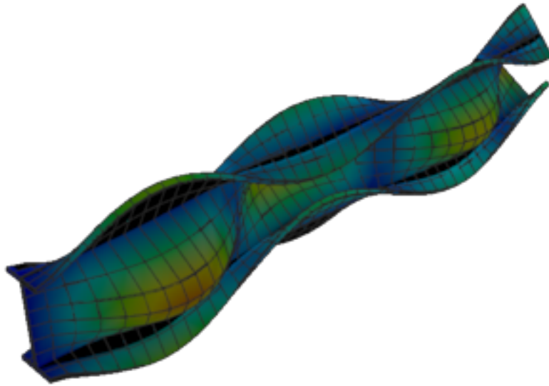
Figure 524: Abaqus — mode 9, 201.839 Hz
