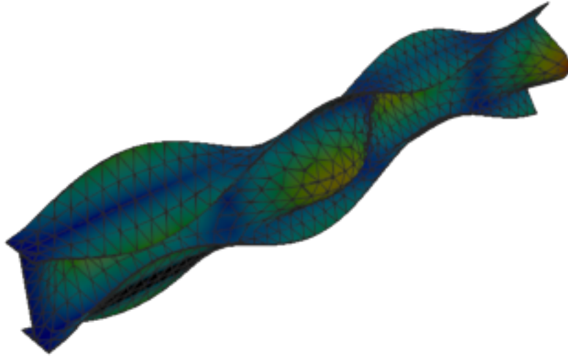
Figure 215: Code_Aster — mode 9, 192.406 Hz
