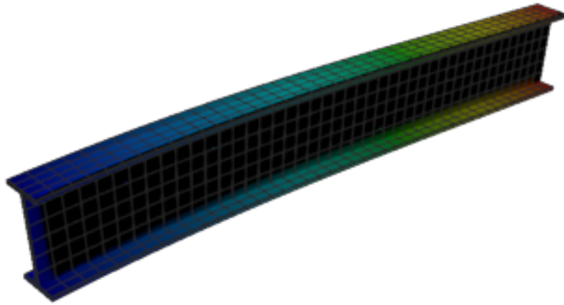
Figure 124: Calculix — mode 3, 52.000 Hz
