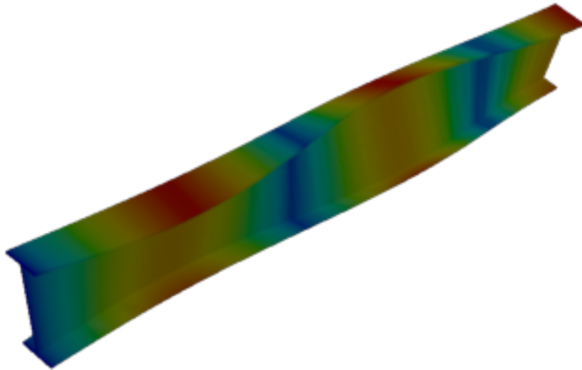
Figure 21: Abaqus — mode 5, 53.855 Hz
