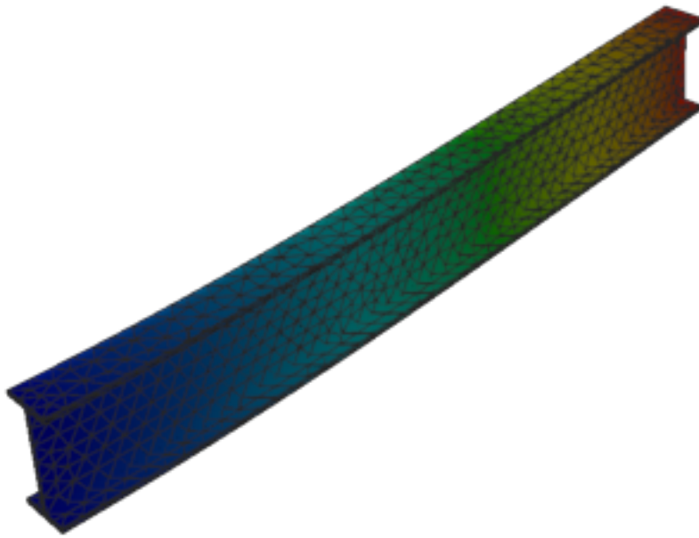
Figure 297: Code_Aster — mode 2, 51.587 Hz
