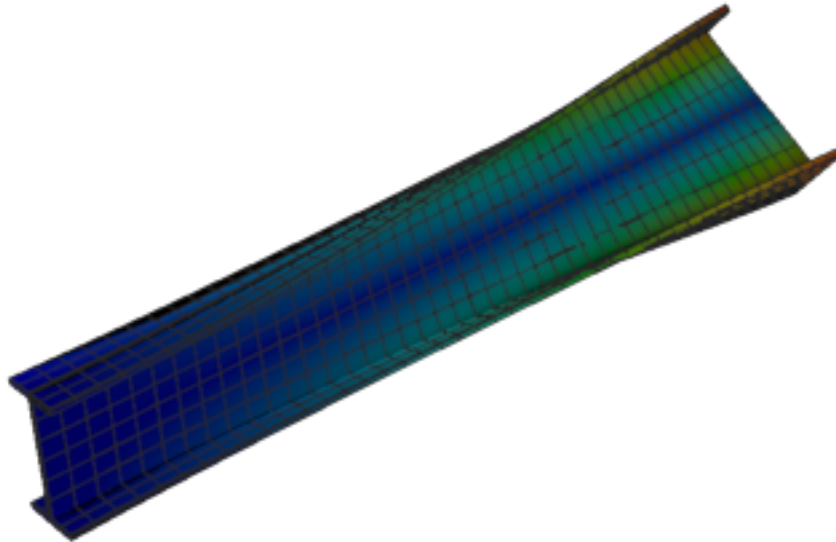
Figure 460: Abaqus — mode 2, 20.150 Hz
