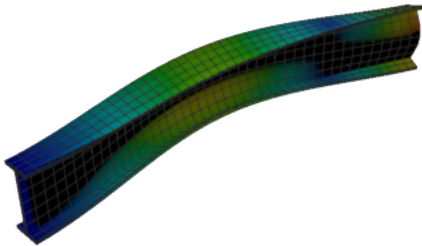
Figure 238: Calculix — mode 4, 75.269 Hz
