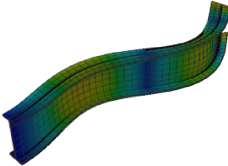
Figure 357: Code_Aster — mode 6, 227.250 Hz
