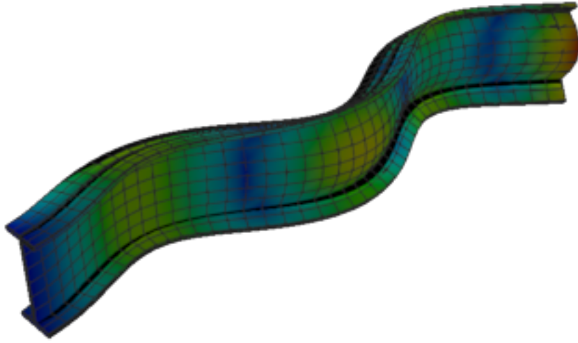
Figure 407: Calculix — mode 10, 456.762 Hz
