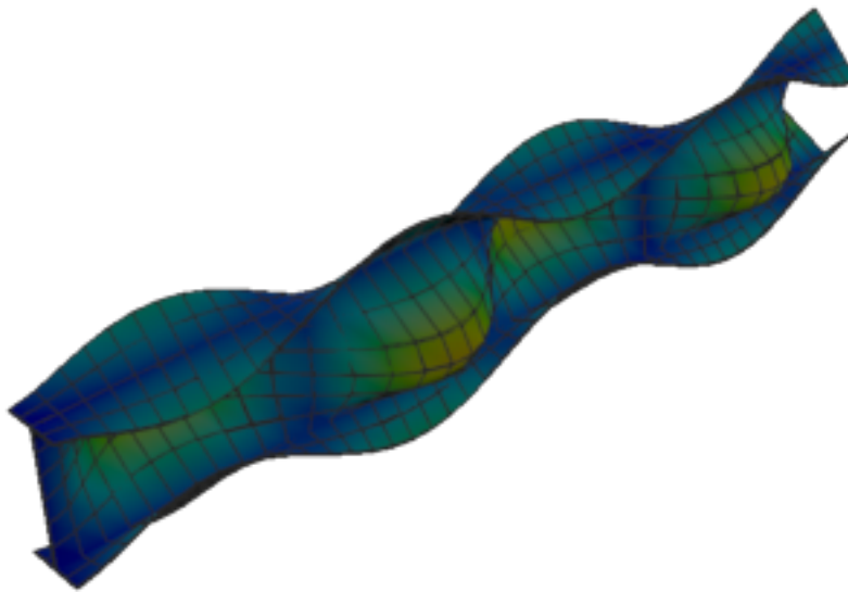
Figure 153: Code_Aster — mode 10, 233.817 Hz
