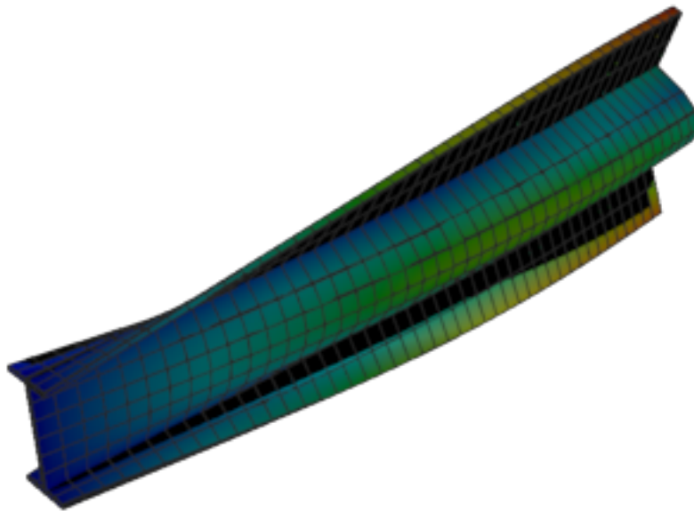
Figure 388: Abaqus — mode 4, 55.271 Hz
