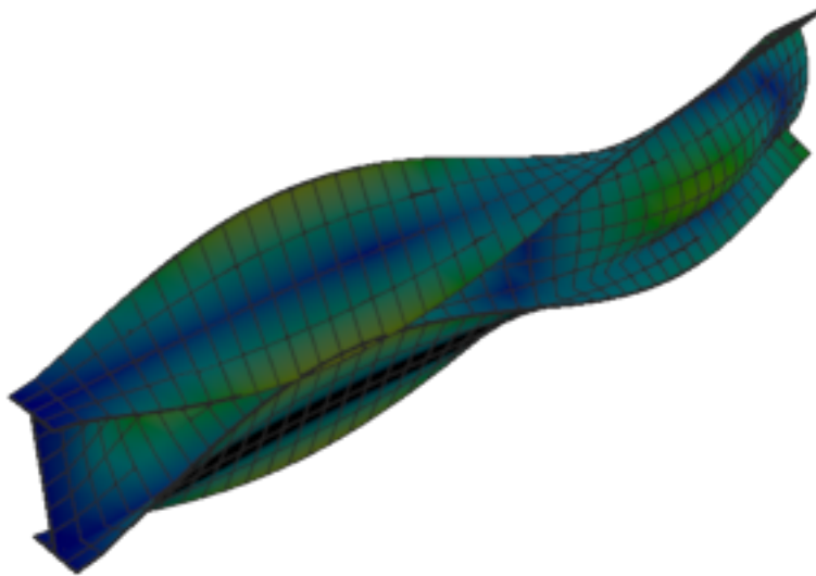
Figure 139: Abaqus — mode 7, 145.566 Hz
