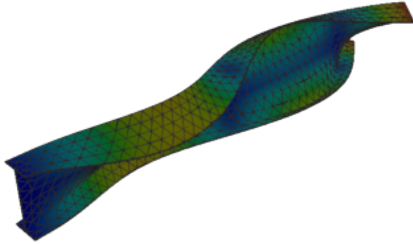
Figure 223: Code_Aster — mode 11, 250.175 Hz
