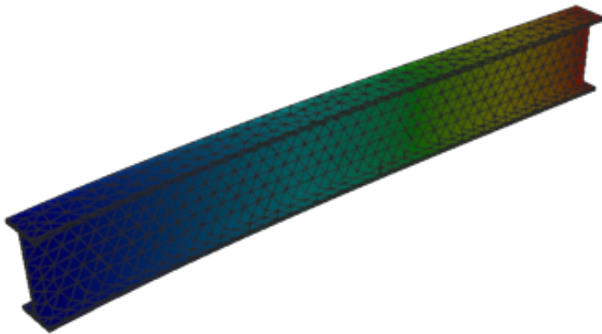
Figure 294: Sesam — mode 1, 15.793 Hz
