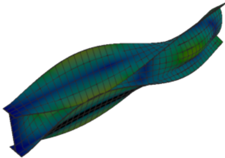
Figure 171: Abaqus — mode 7, 144.579 Hz
