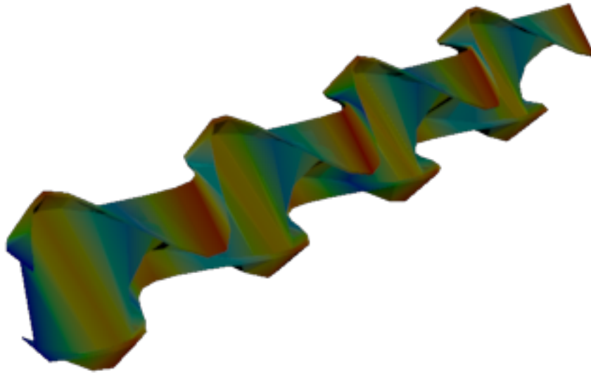
Figure 81: Sesam — mode 11, 149.217 Hz
