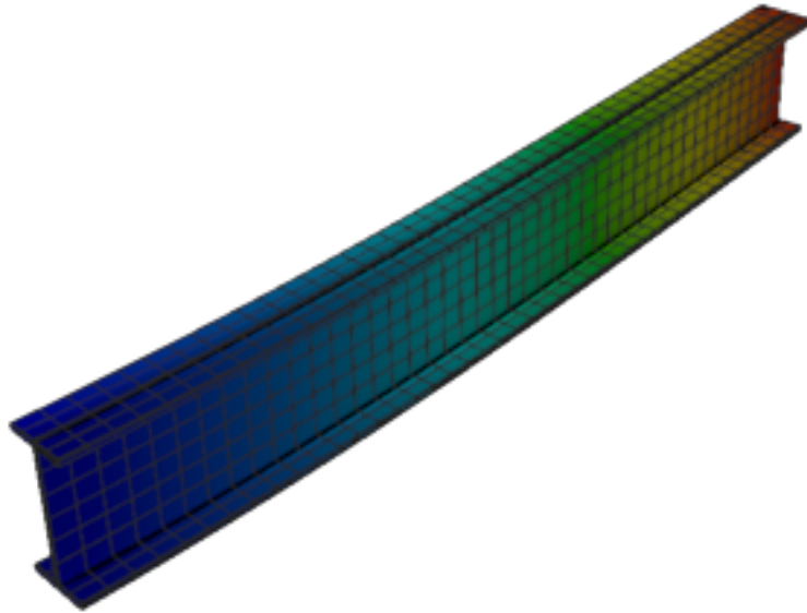
Figure 501: Calculix — mode 1, 12.943 Hz
