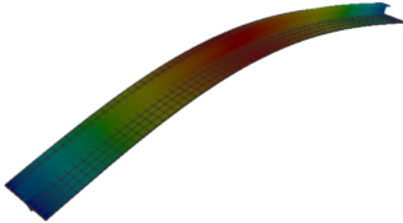
Figure 557: Abaqus — mode 1, 21.242 Hz
