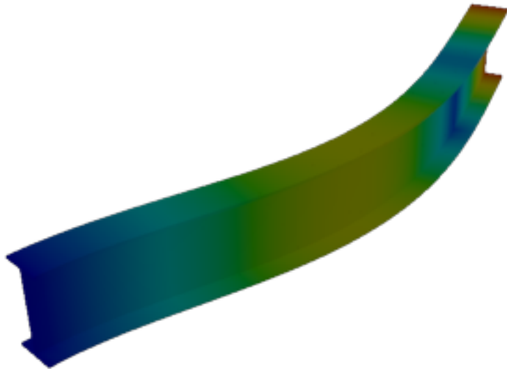
Figure 27: Code_Aster — mode 6, 81.340 Hz
