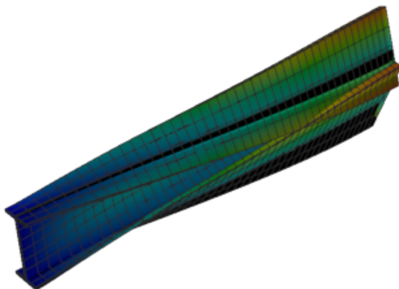
Figure 515: Abaqus — mode 6, 130.809 Hz
