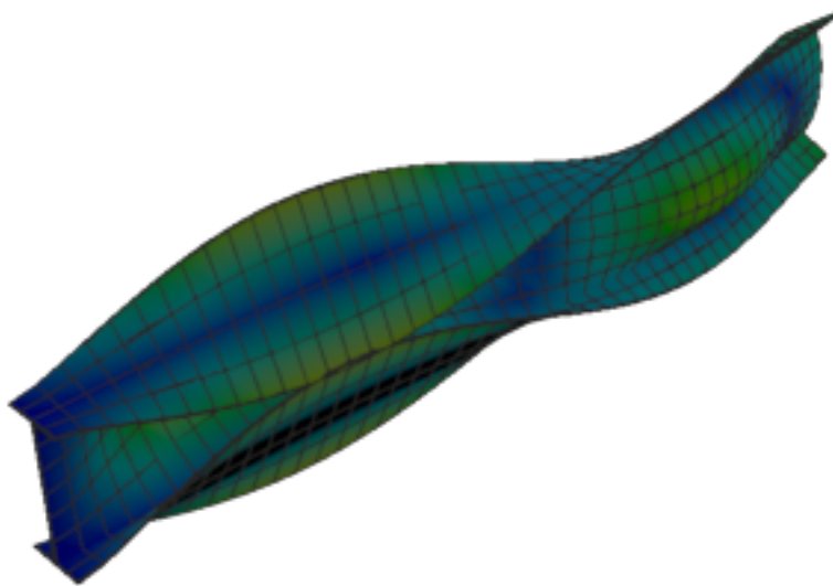
Figure 141: Code_Aster — mode 7, 143.864 Hz
