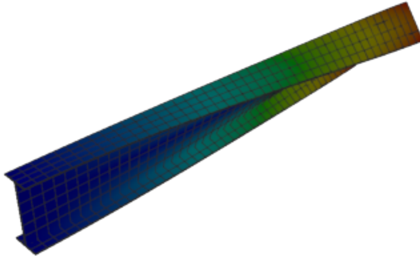
Figure 229: Abaqus — mode 2, 19.486 Hz
