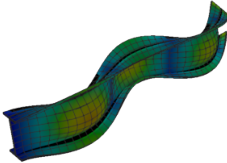
Figure 369: Code_Aster — mode 9, 407.869 Hz
