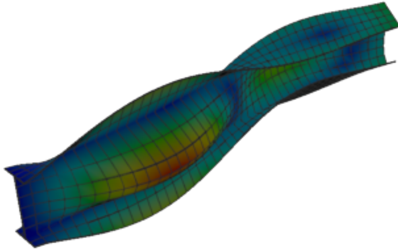
Figure 251: Code_Aster — mode 7, 142.233 Hz
