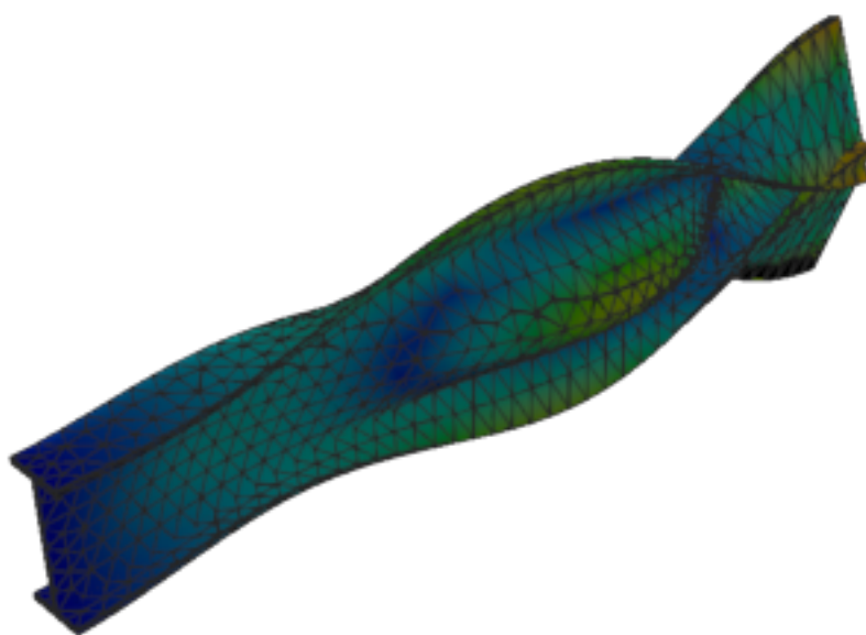
Figure 442: Code_Aster — mode 8, 181.026 Hz
