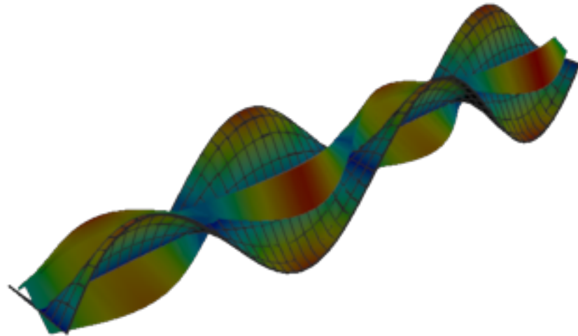
Figure 574: Sesam — mode 6, 134.472 Hz
