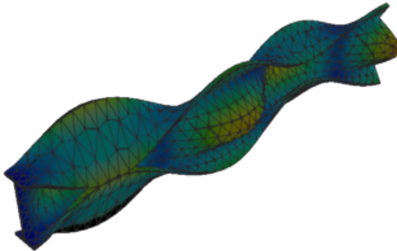
Figure 444: Abaqus — mode 9, 215.822 Hz
