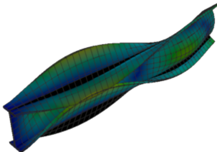
Figure 482: Code_Aster — mode 7, 149.958 Hz
