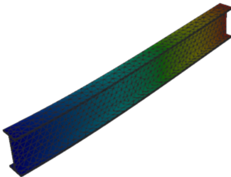
Figure 421: Calculix — mode 3, 50.540 Hz
