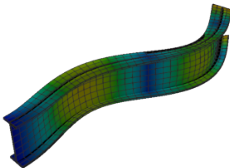
Figure 356: Calculix — mode 6, 227.250 Hz
