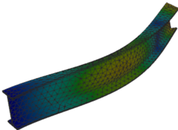
Figure 425: Calculix — mode 4, 77.230 Hz
