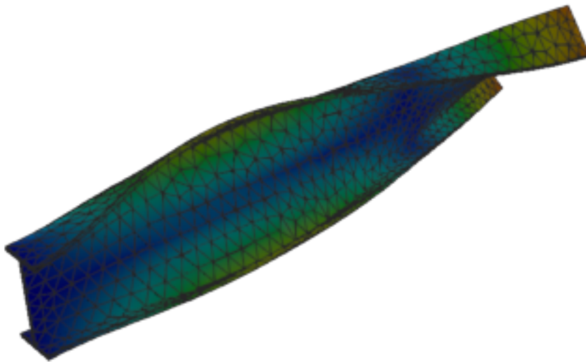
Figure 316: Calculix — mode 7, 357.062 Hz
