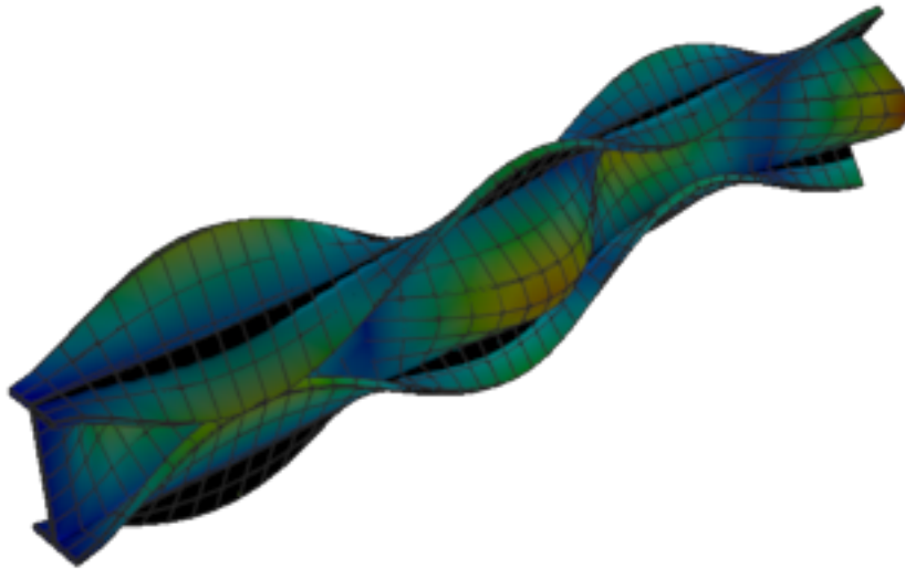
Figure 370: Sesam — mode 9, 214.689 Hz
