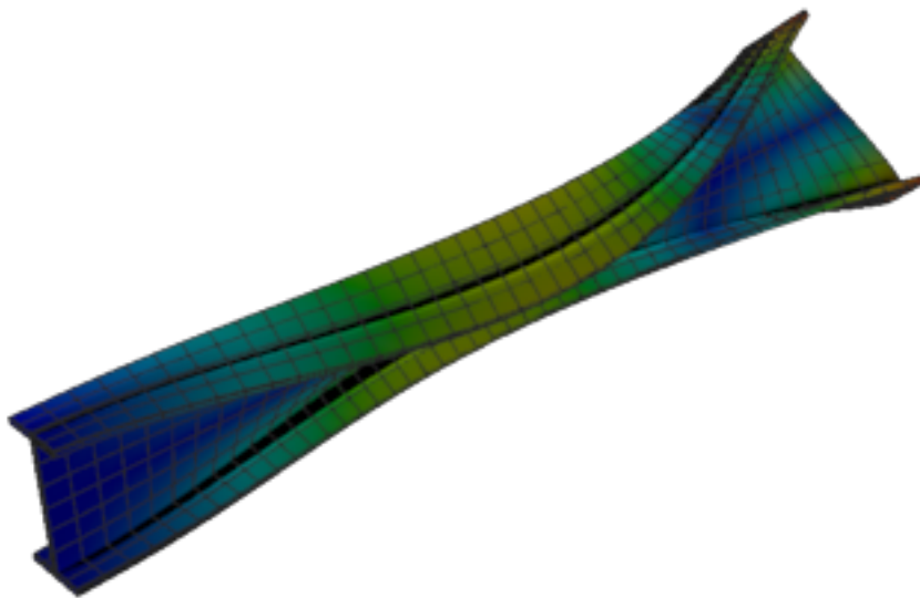
Figure 472: Abaqus — mode 5, 97.594 Hz
