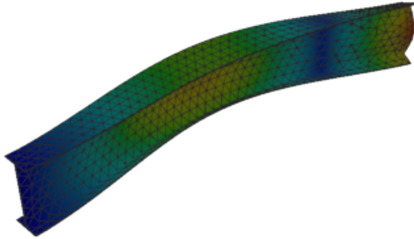
Figure 195: Code_Aster — mode 4, 75.144 Hz
