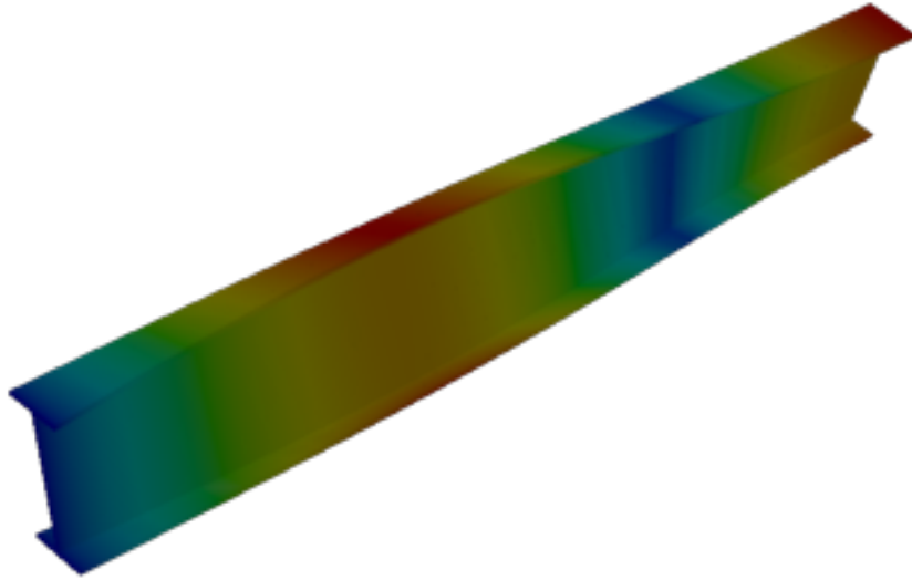
Figure 64: Abaqus — mode 3, 32.358 Hz
