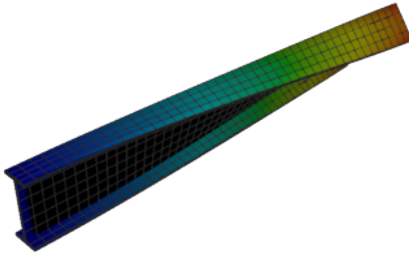
Figure 272: Calculix — mode 2, 19.502 Hz
