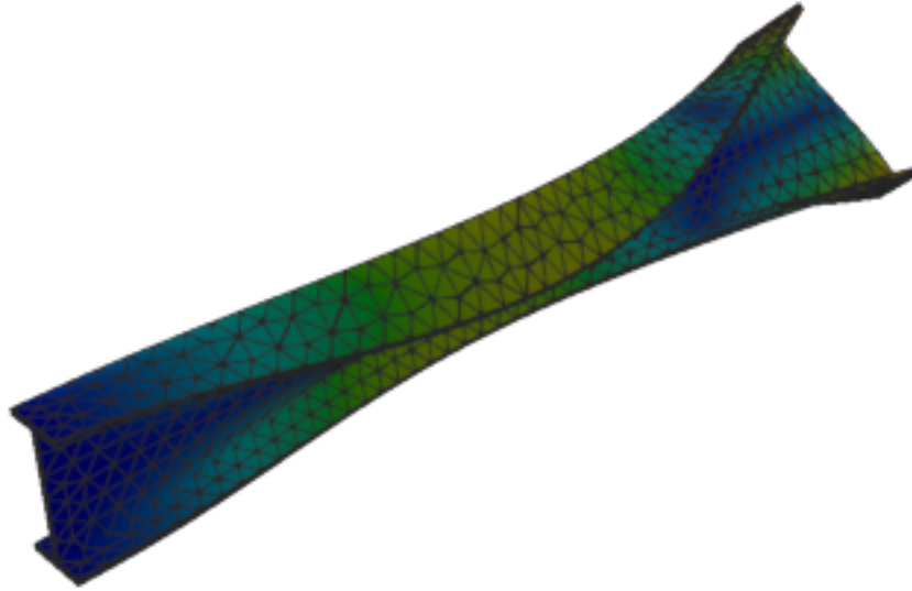
Figure 431: Sesam — mode 5, 97.830 Hz
