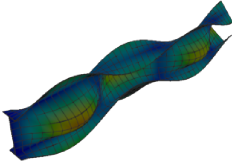
Figure 259: Code_Aster — mode 9, 191.998 Hz
