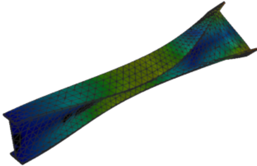
Figure 94: Calculix — mode 5, 132.927 Hz
