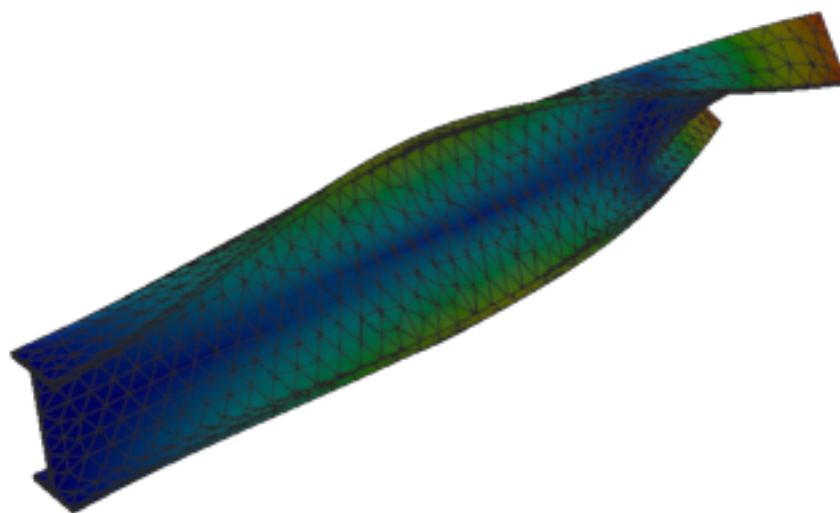
Figure 429: Calculix — mode 5, 97.851 Hz
