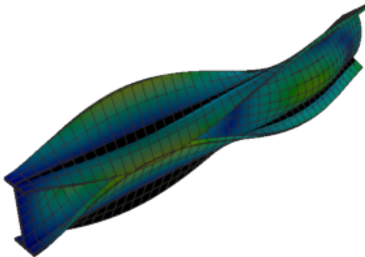
Figure 520: Code_Aster — mode 7, 148.474 Hz
