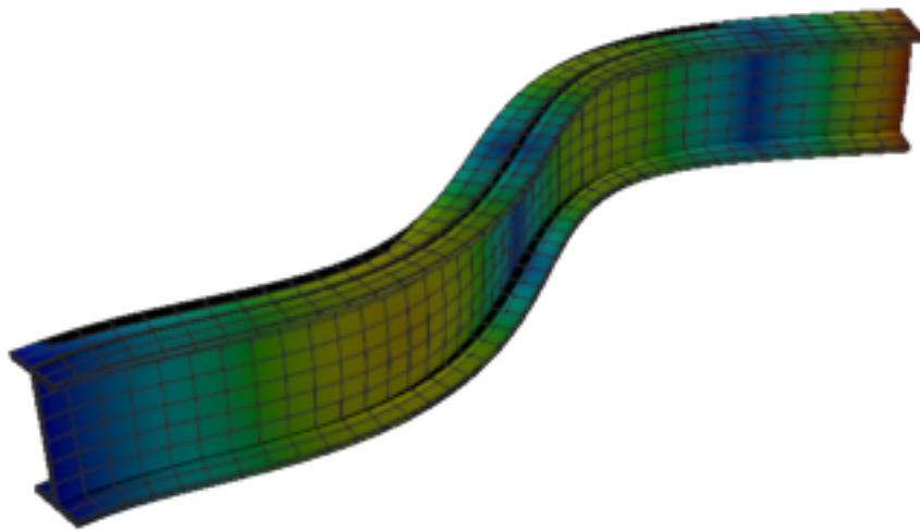
Figure 392: Calculix — mode 5, 240.766 Hz
