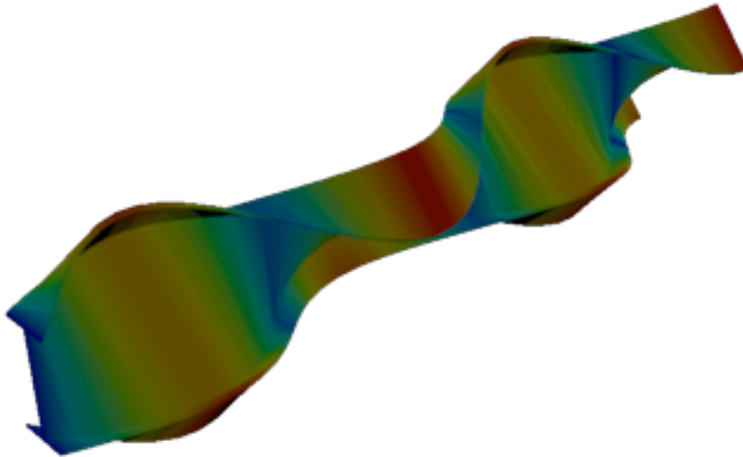
Figure 73: Sesam — mode 7, 70.143 Hz
