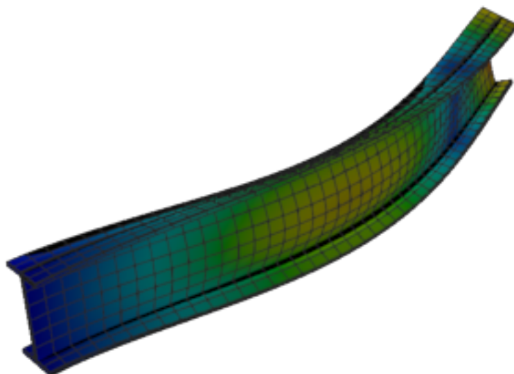
Figure 509: Abaqus — mode 4, 76.687 Hz
