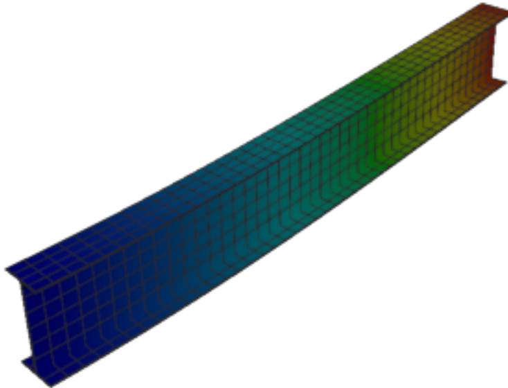
Figure 115: Abaqus — mode 1, 12.780 Hz
