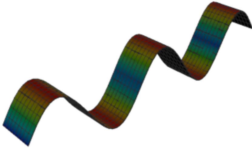
Figure 551: Code_Aster — mode 5, 38.415 Hz
