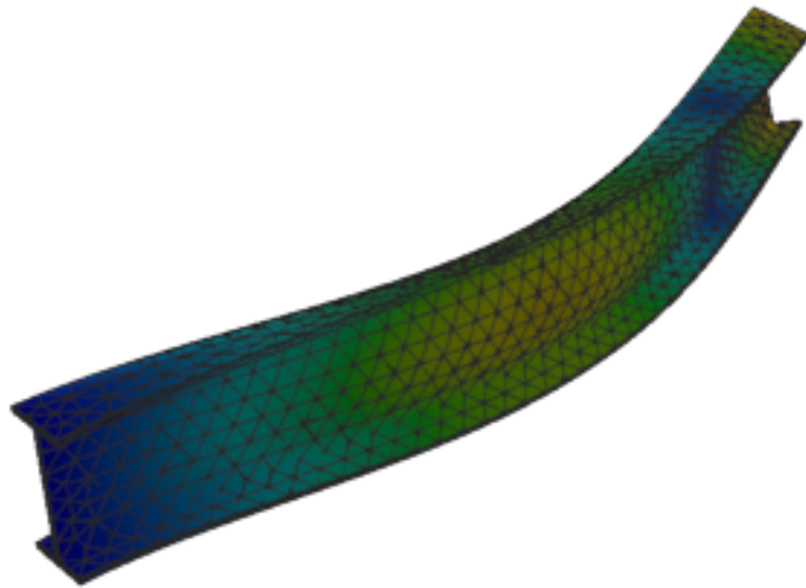
Figure 427: Sesam — mode 4, 77.128 Hz
