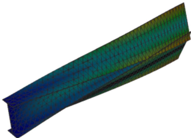
Figure 201: Abaqus — mode 6, 125.207 Hz
