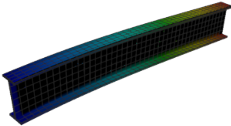
Figure 274: Calculix — mode 3, 51.974 Hz
