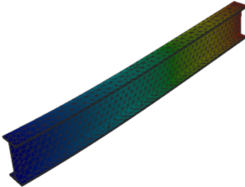
Figure 420: Abaqus — mode 3, 50.540 Hz
