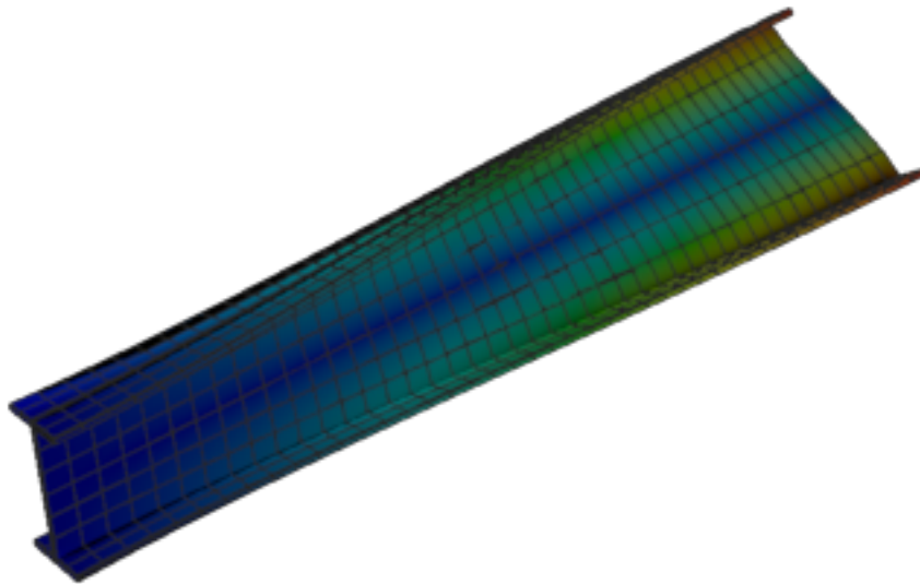
Figure 382: Abaqus — mode 2, 34.157 Hz
