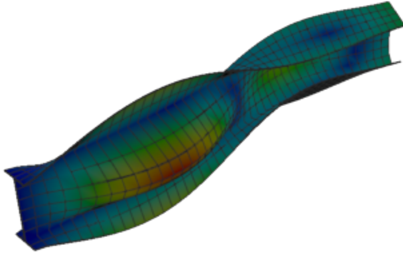
Figure 142: Sesam — mode 7, 141.556 Hz
