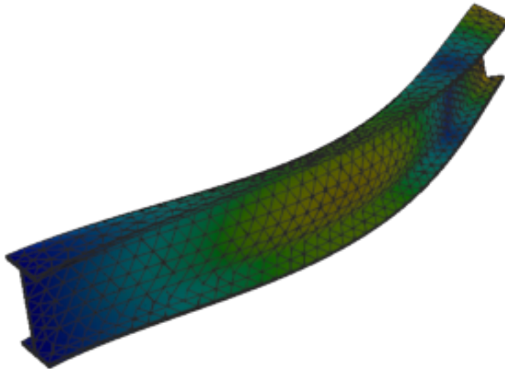
Figure 424: Abaqus — mode 4, 77.128 Hz
