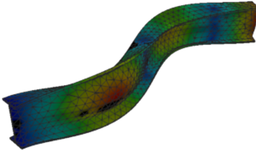
Figure 97: Calculix — mode 6, 218.167 Hz
