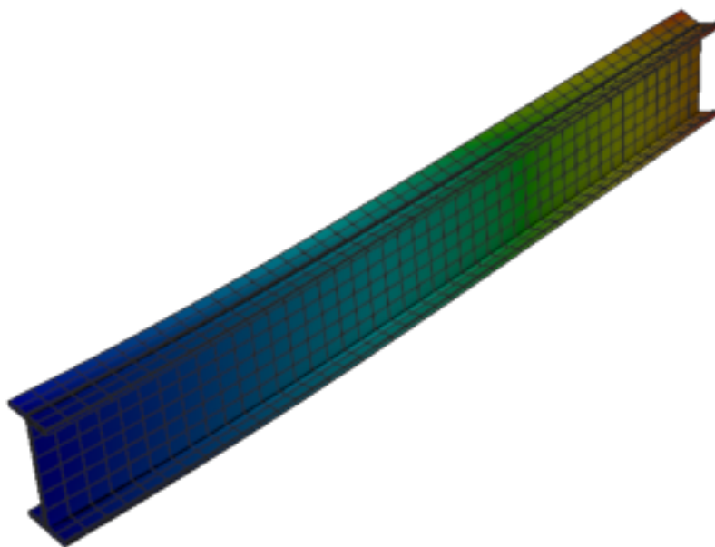
Figure 385: Abaqus — mode 3, 49.598 Hz
