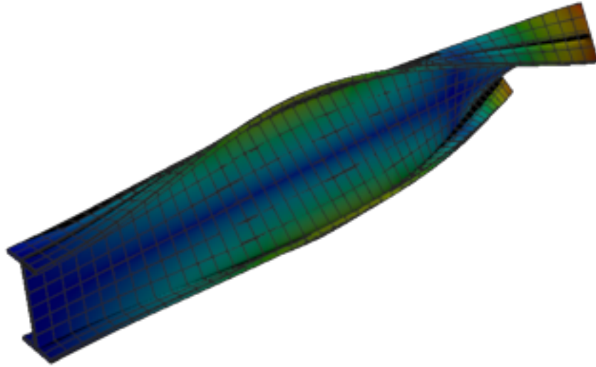
Figure 353: Code_Aster — mode 5, 102.334 Hz
