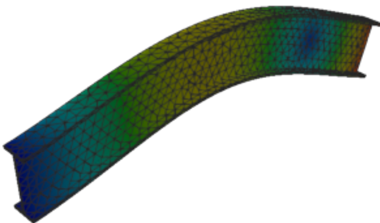
Figure 308: Calculix — mode 5, 261.877 Hz
