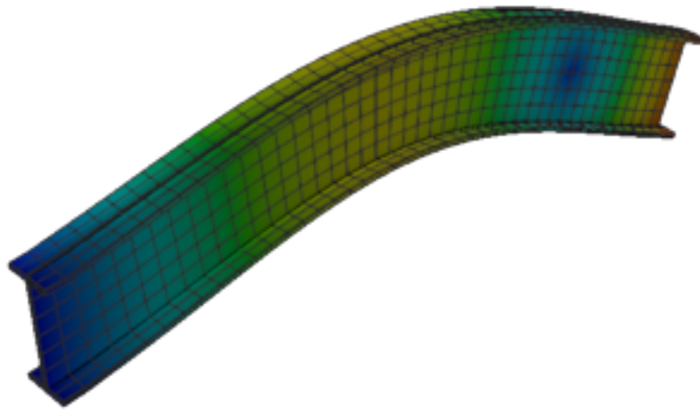
Figure 499: Sesam — mode 11, 252.742 Hz
