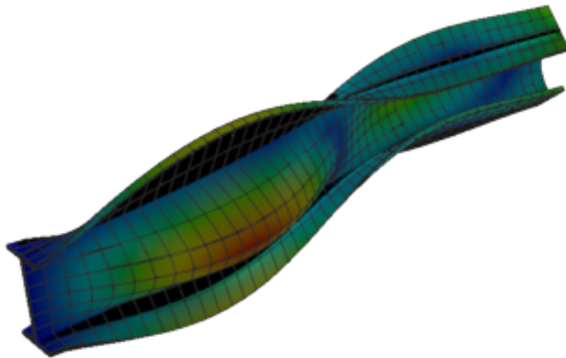
Figure 362: Sesam — mode 7, 153.833 Hz
