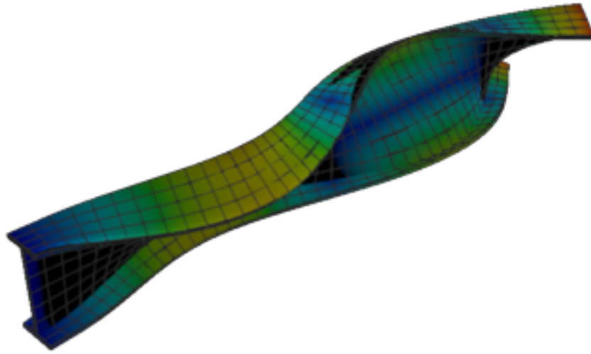
Figure 156: Calculix — mode 11, 251.554 Hz
