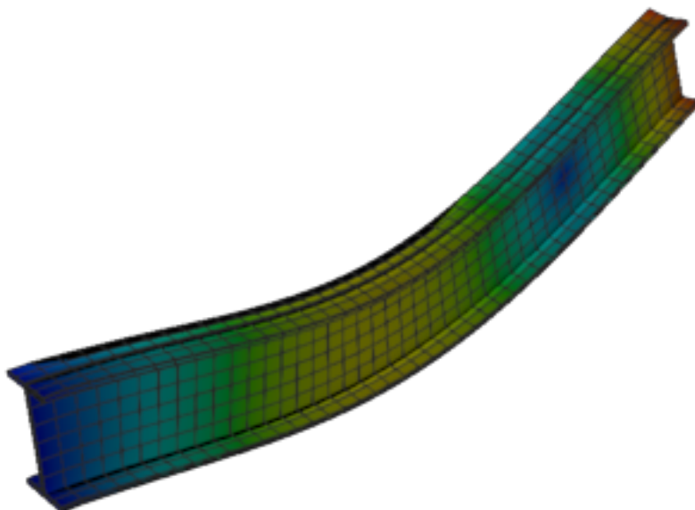
Figure 532: Code_Aster — mode 11, 252.573 Hz
