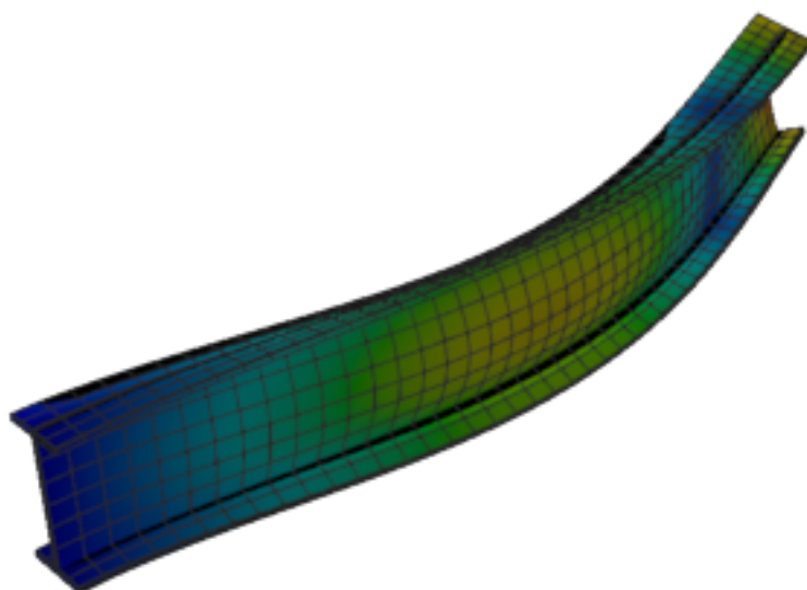
Figure 510: Calculix — mode 4, 76.688 Hz
