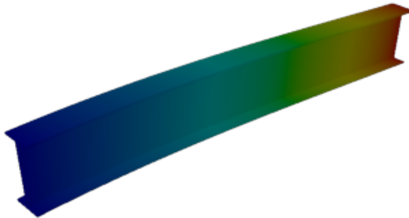
Figure 67: Sesam — mode 4, 41.236 Hz
