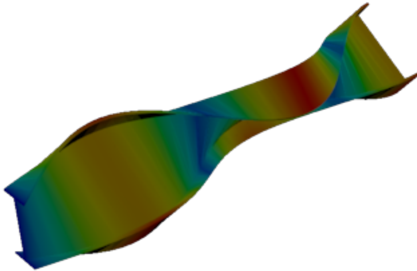
Figure 69: Sesam — mode 5, 50.149 Hz
