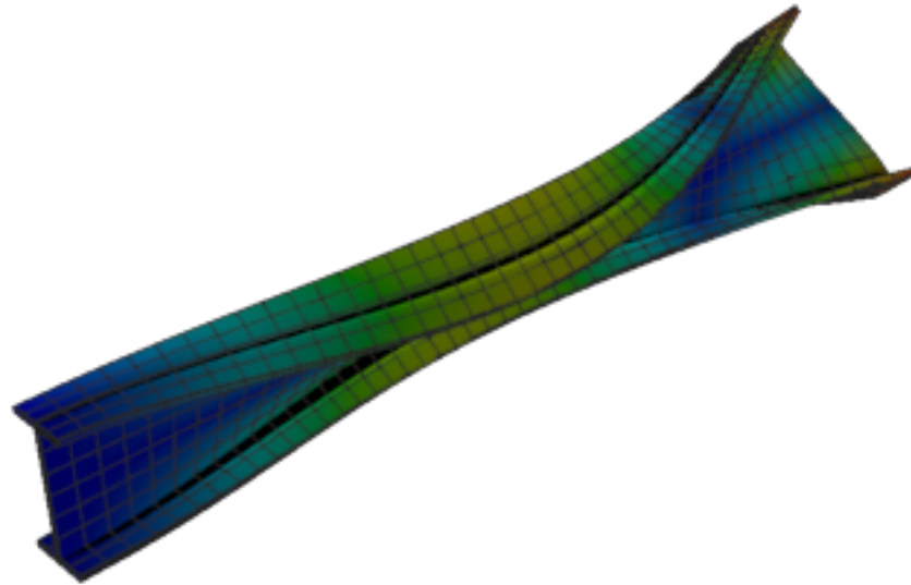
Figure 354: Sesam — mode 5, 98.119 Hz
