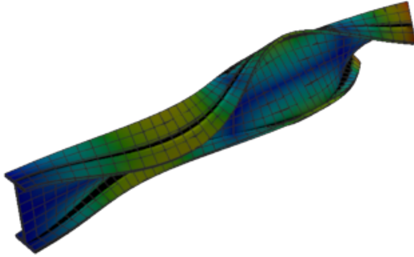
Figure 365: Code_Aster — mode 8, 266.519 Hz
