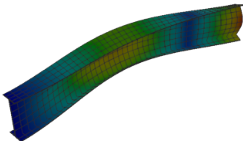
Figure 129: Code_Aster — mode 4, 77.236 Hz
