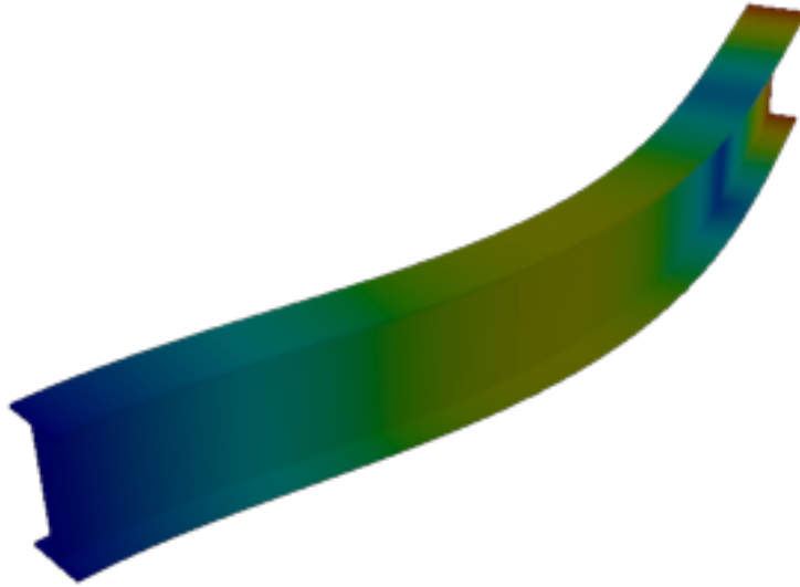
Figure 72: Abaqus — mode 7, 79.684 Hz
