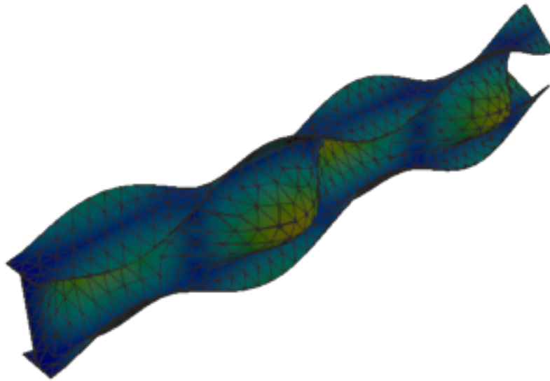
Figure 219: Code_Aster — mode 10, 233.389 Hz
