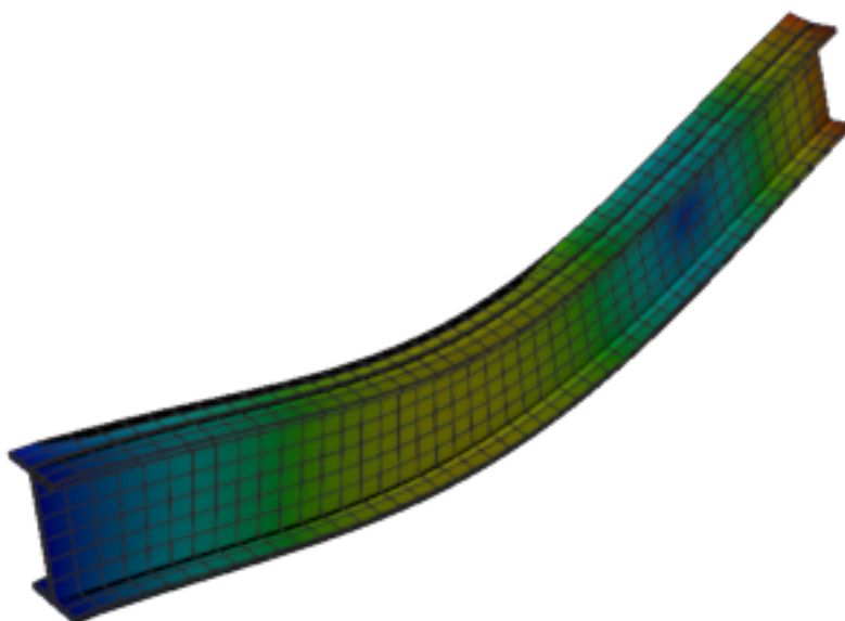
Figure 498: Code_Aster — mode 11, 252.917 Hz
