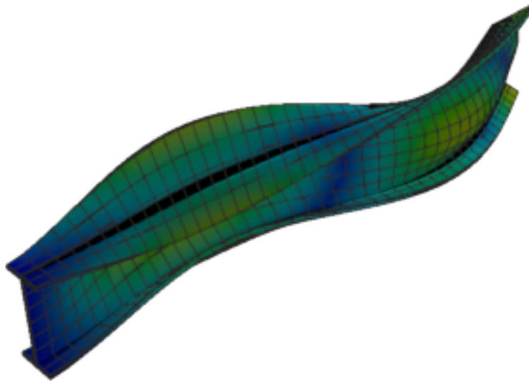
Figure 399: Code_Aster — mode 7, 205.267 Hz
