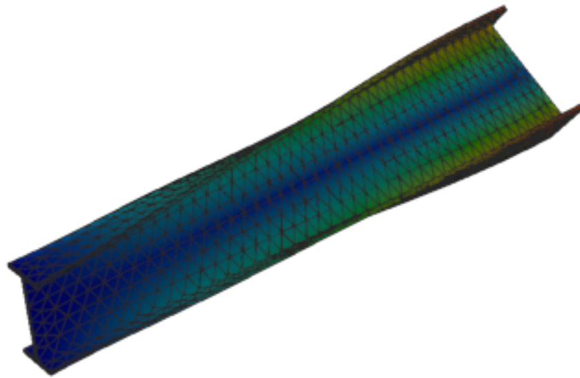
Figure 306: Sesam — mode 4, 105.691 Hz
