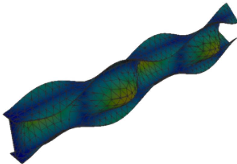
Figure 217: Abaqus — mode 10, 233.355 Hz
