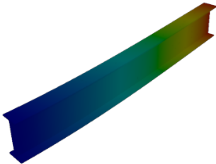
Figure 9: Abaqus — mode 2, 12.928 Hz
