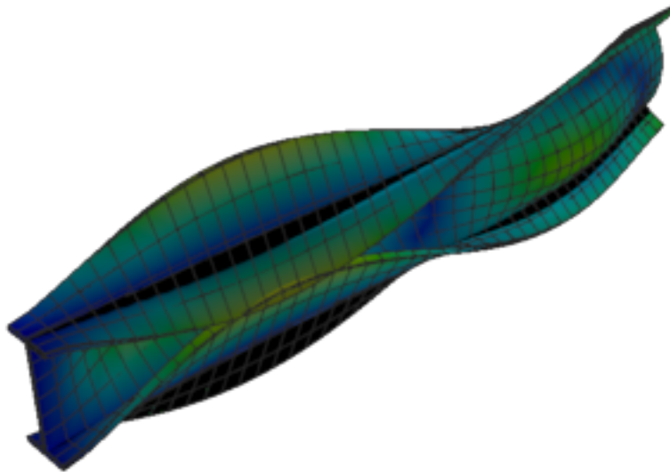
Figure 480: Abaqus — mode 7, 149.958 Hz
