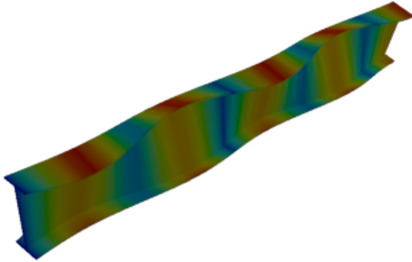
Figure 74: Abaqus — mode 8, 97.074 Hz
