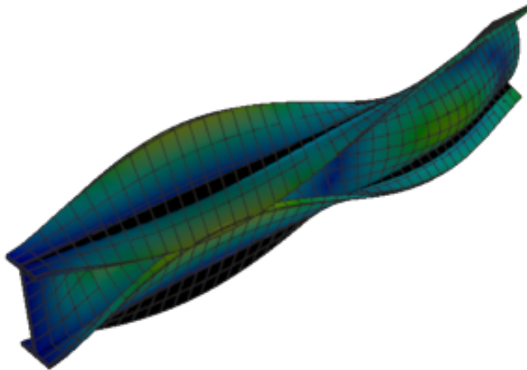
Figure 518: Abaqus — mode 7, 148.474 Hz
