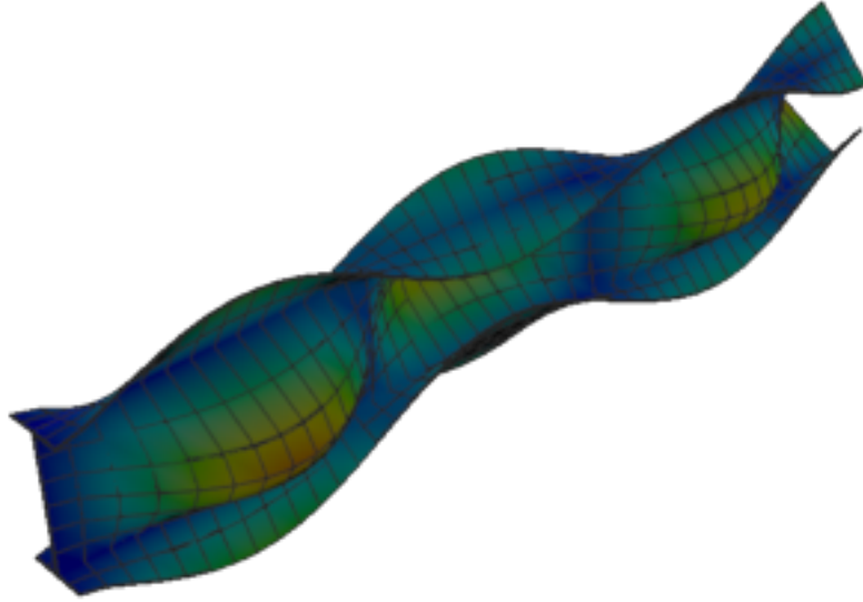
Figure 150: Sesam — mode 9, 190.099 Hz
