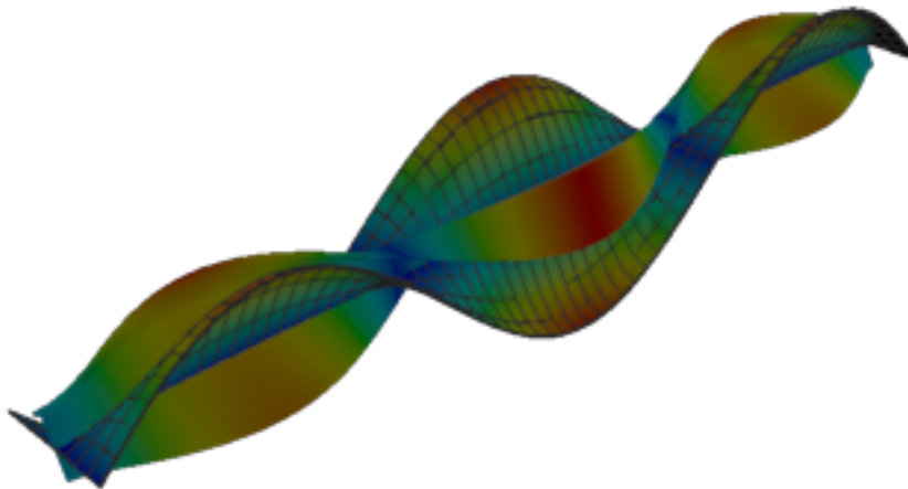
Figure 570: Code_Aster — mode 5, 112.038 Hz
