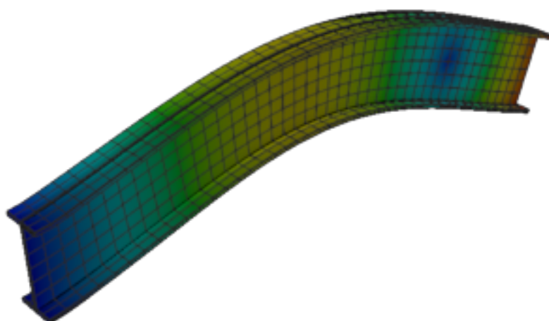
Figure 360: Calculix — mode 7, 255.872 Hz
