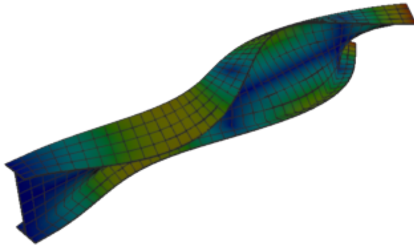
Figure 158: Sesam — mode 11, 250.786 Hz
