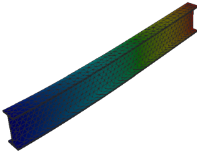
Figure 295: Abaqus — mode 2, 51.532 Hz
