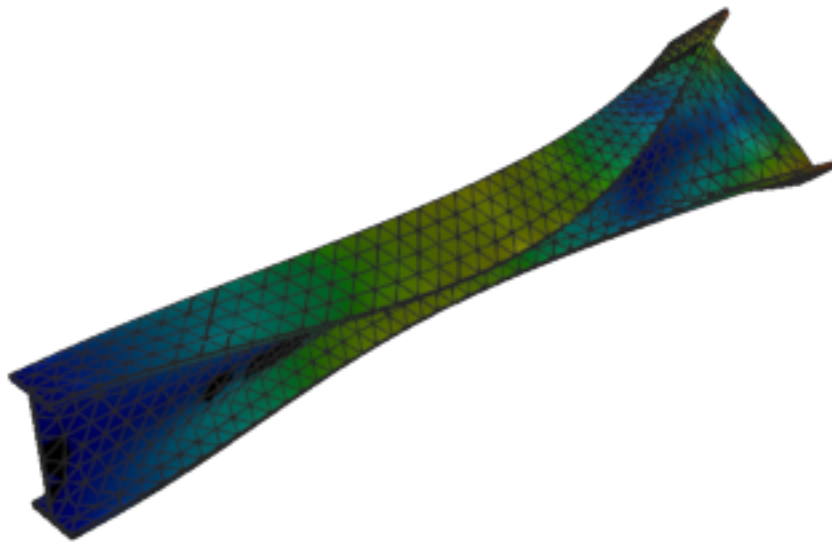
Figure 198: Calculix — mode 5, 95.971 Hz
