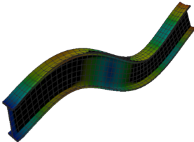
Figure 180: Calculix — mode 11, 589.240 Hz
