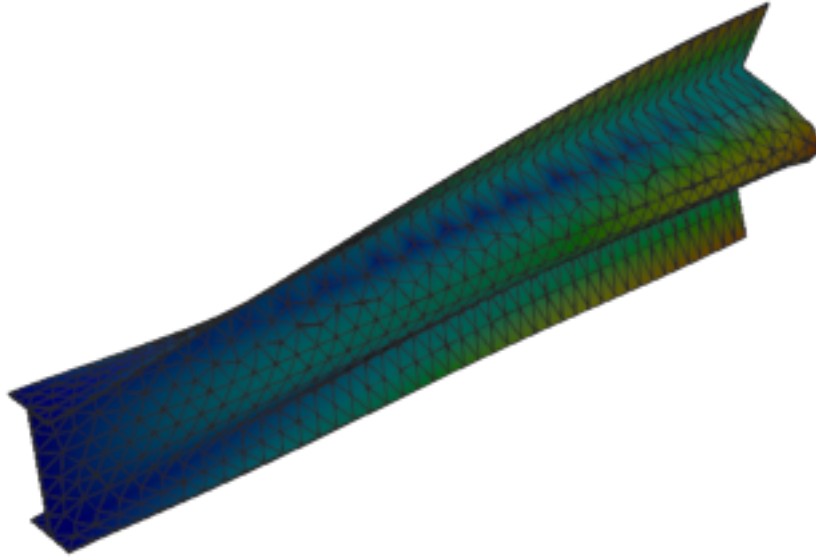
Figure 98: Code_Aster — mode 6, 125.459 Hz
