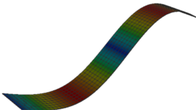
Figure 539: Code_Aster — mode 2, 6.146 Hz
