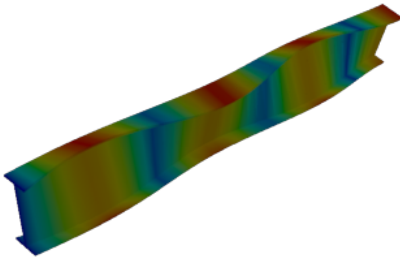
Figure 31: Code_Aster — mode 7, 85.947 Hz
