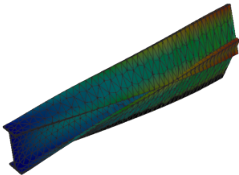
Figure 434: Code_Aster — mode 6, 133.014 Hz
