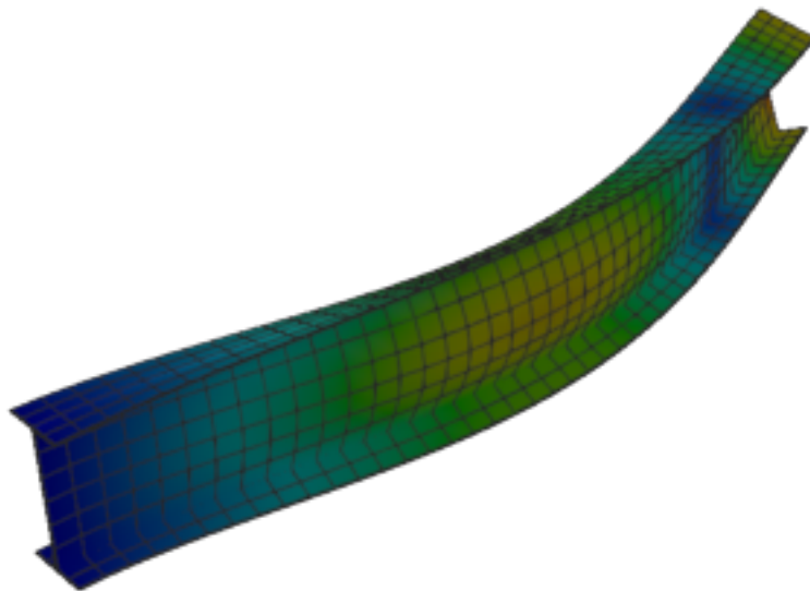
Figure 240: Sesam — mode 4, 75.125 Hz
