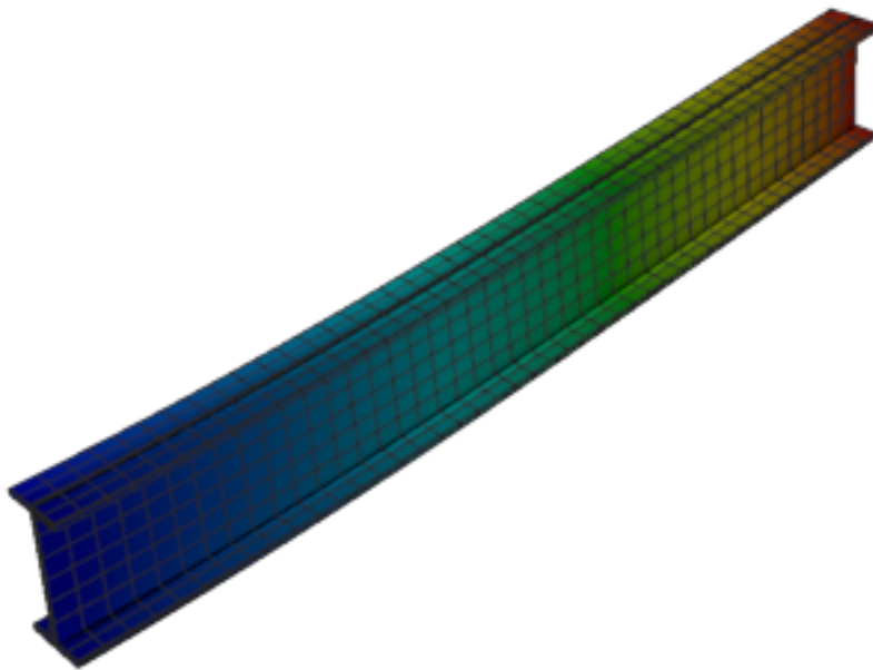
Figure 344: Calculix — mode 3, 50.825 Hz
