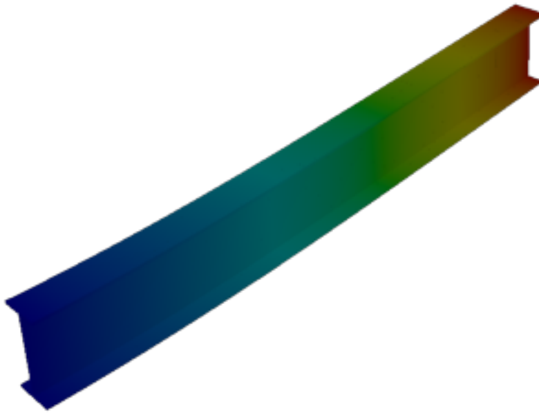
Figure 66: Abaqus — mode 4, 50.557 Hz
