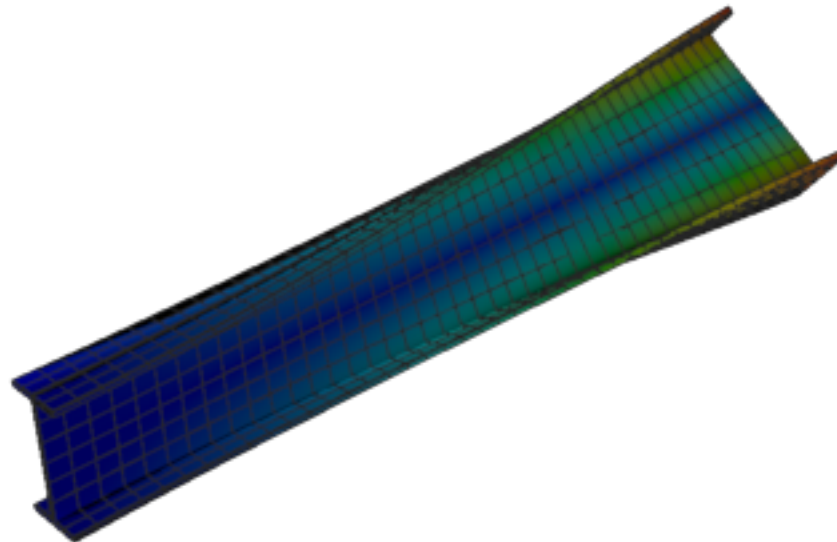
Figure 342: Sesam — mode 2, 20.302 Hz
