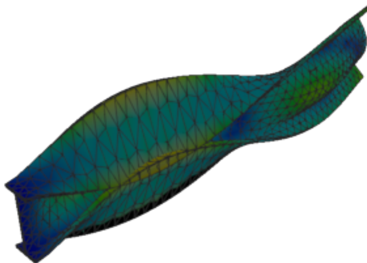
Figure 437: Calculix — mode 7, 154.803 Hz
