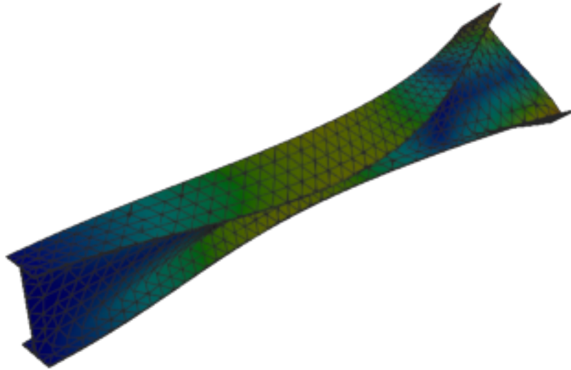
Figure 200: Sesam — mode 5, 95.934 Hz
