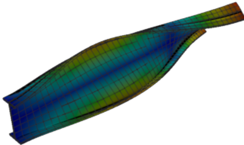
Figure 398: Calculix — mode 7, 351.823 Hz
