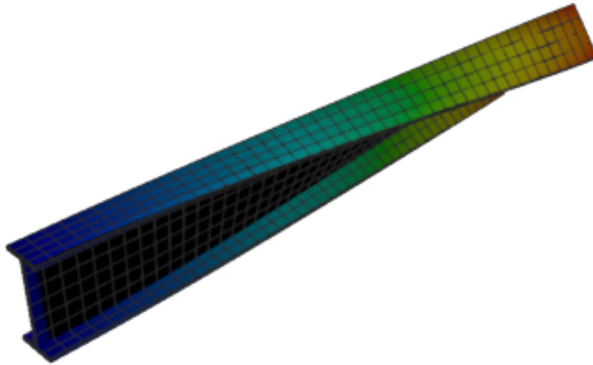
Figure 120: Calculix — mode 2, 19.630 Hz
