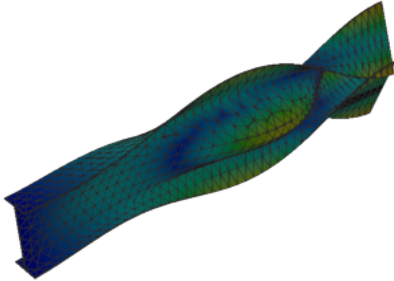
Figure 211: Code_Aster — mode 8, 165.790 Hz
