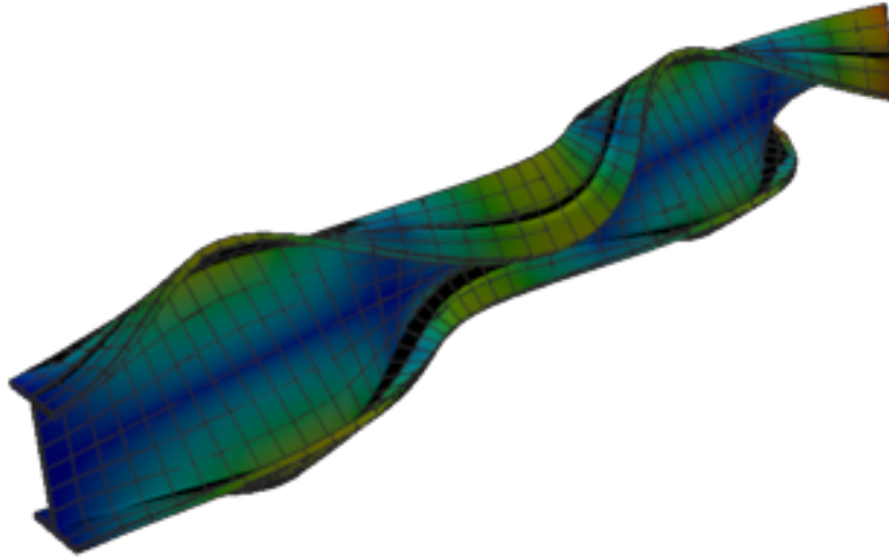
Figure 377: Code_Aster — mode 11, 500.931 Hz
