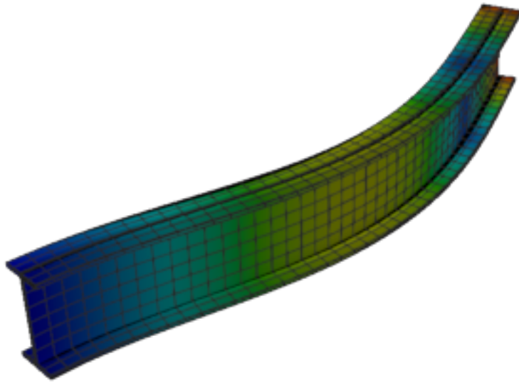
Figure 347: Abaqus — mode 4, 82.799 Hz
