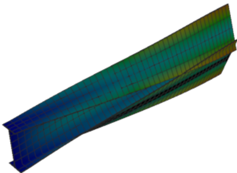
Figure 137: Code_Aster — mode 6, 125.442 Hz
