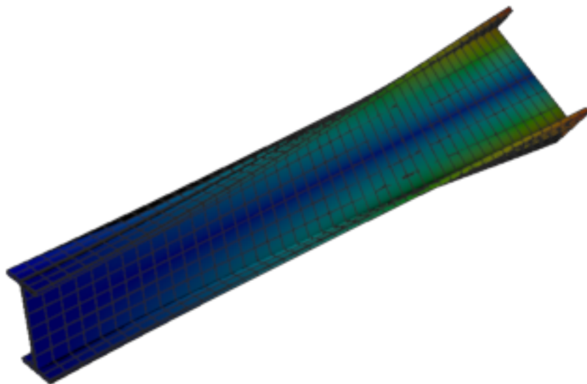
Figure 340: Calculix — mode 2, 21.069 Hz
