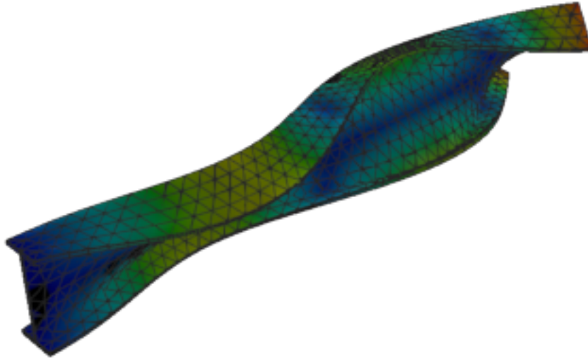
Figure 103: Calculix — mode 8, 297.856 Hz
