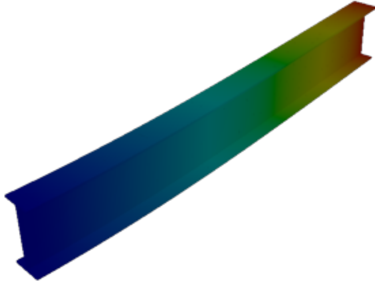
Figure 12: Sesam — mode 2, 12.943 Hz
