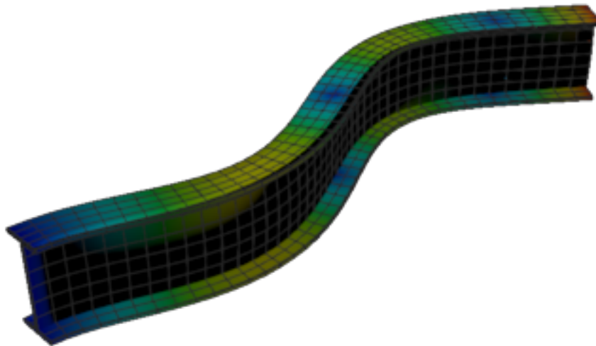
Figure 168: Calculix — mode 5, 239.804 Hz
