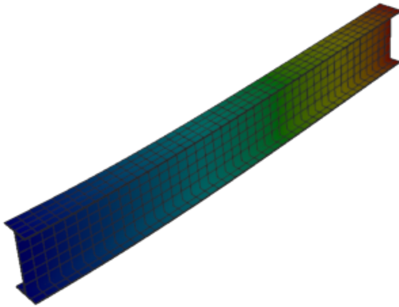
Figure 163: Abaqus — mode 3, 51.849 Hz
