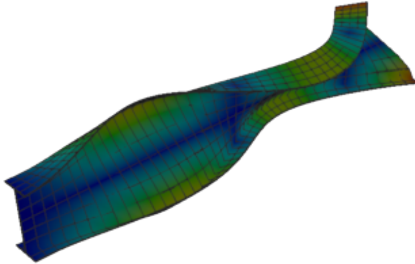
Figure 289: Abaqus — mode 11, 250.173 Hz
