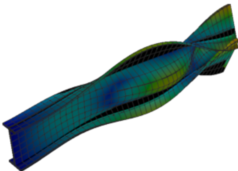
Figure 486: Code_Aster — mode 8, 173.925 Hz
