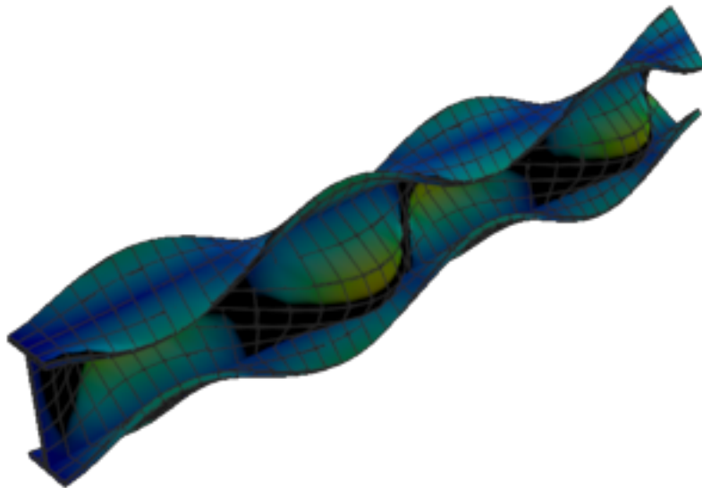
Figure 288: Calculix — mode 10, 234.347 Hz
