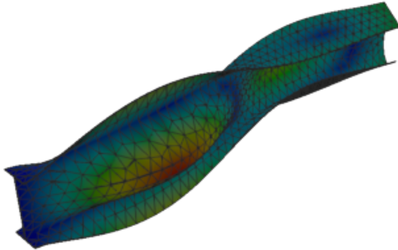
Figure 208: Sesam — mode 7, 142.768 Hz
