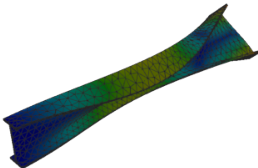
Figure 430: Code_Aster — mode 5, 97.851 Hz
