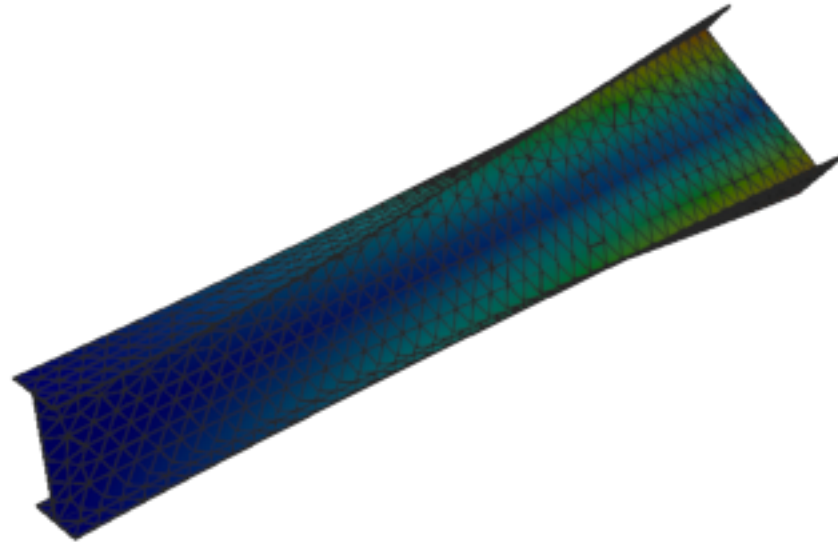
Figure 188: Sesam — mode 2, 19.505 Hz
