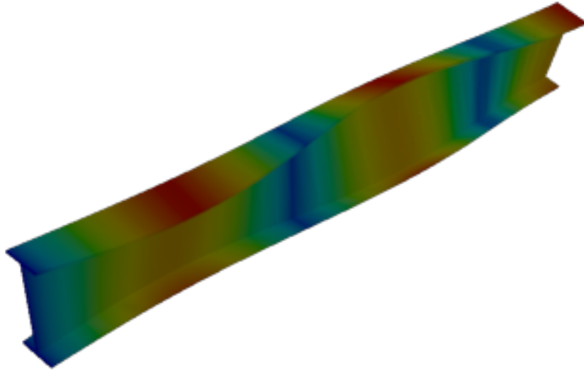
Figure 68: Abaqus — mode 5, 53.930 Hz
