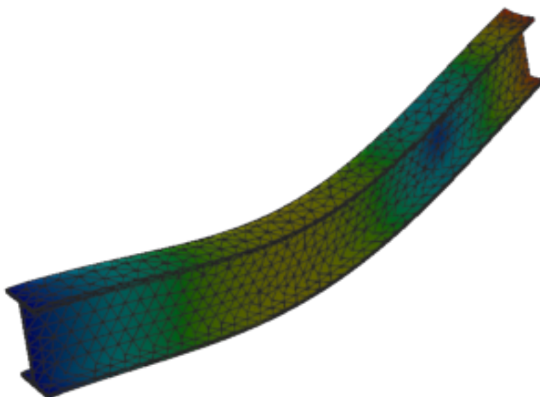
Figure 450: Code_Aster — mode 10, 253.193 Hz
