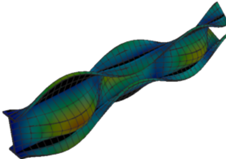
Figure 488: Abaqus — mode 9, 205.292 Hz
