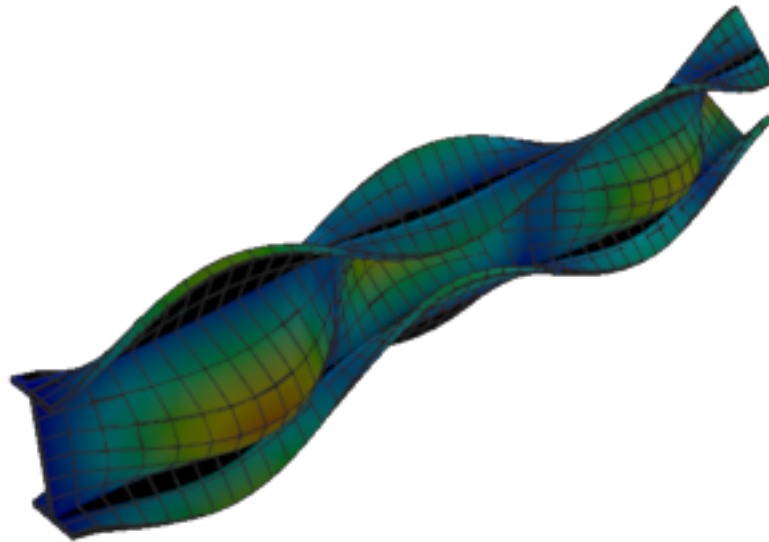
Figure 526: Code_Aster — mode 9, 201.839 Hz
