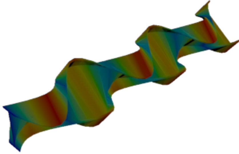
Figure 40: Sesam — mode 9, 135.600 Hz
