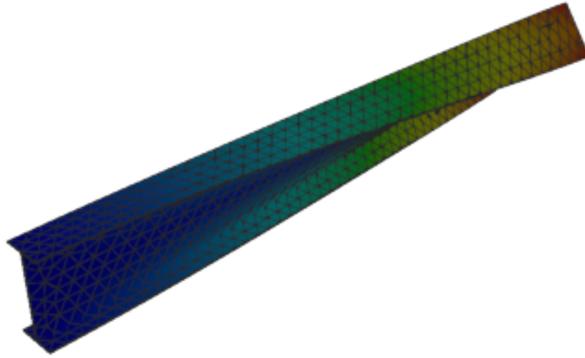
Figure 187: Code_Aster — mode 2, 19.451 Hz
