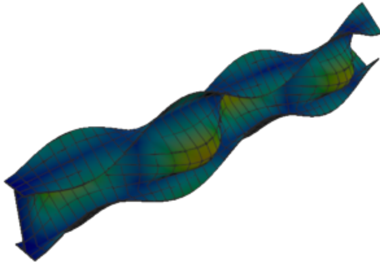
Figure 177: Abaqus — mode 10, 241.275 Hz
