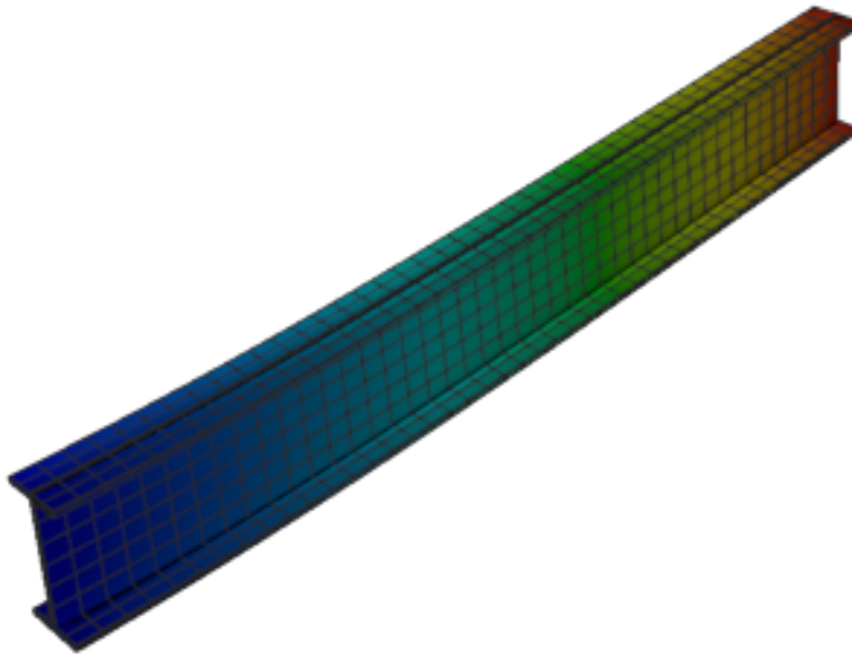
Figure 464: Abaqus — mode 3, 50.541 Hz
