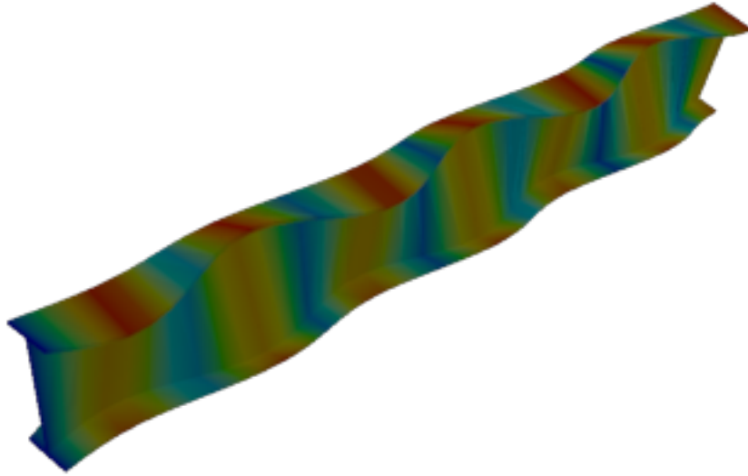
Figure 78: Abaqus — mode 10, 140.222 Hz
