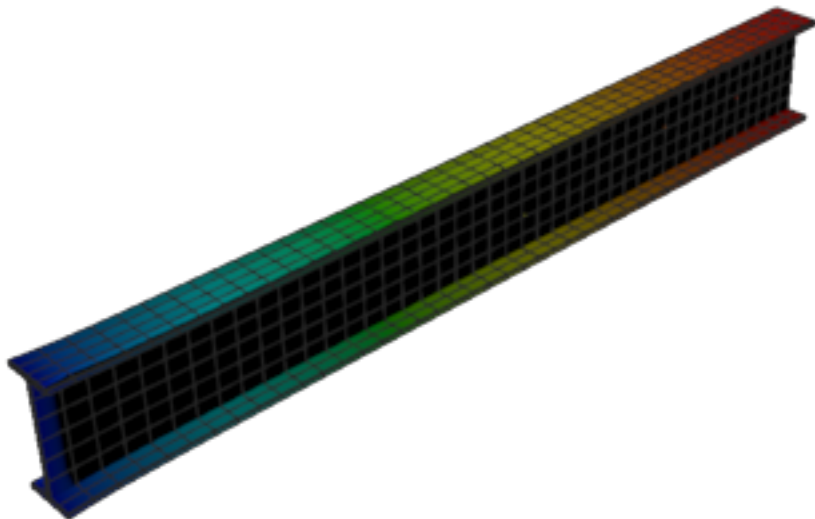
Figure 174: Calculix — mode 8, 431.774 Hz
