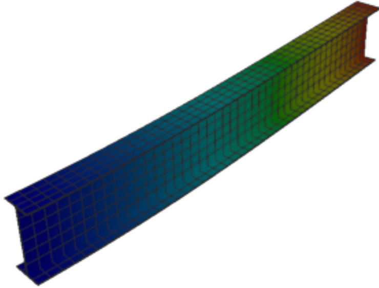
Figure 227: Code_Aster — mode 1, 12.756 Hz
