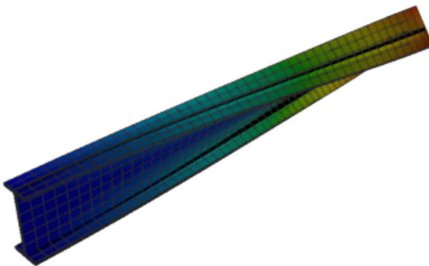
Figure 504: Calculix — mode 2, 20.029 Hz
