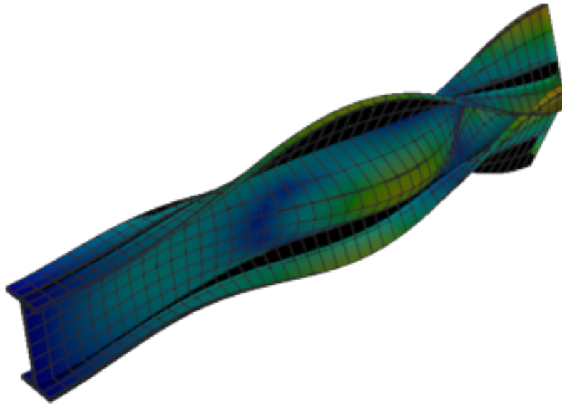
Figure 484: Abaqus — mode 8, 173.925 Hz
