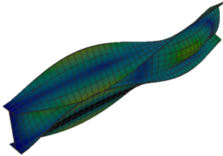
Figure 252: Sesam — mode 7, 142.234 Hz
