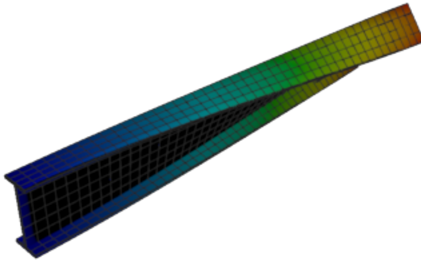
Figure 230: Calculix — mode 2, 19.564 Hz
