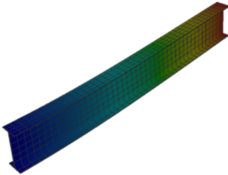
Figure 233: Abaqus — mode 3, 51.998 Hz
