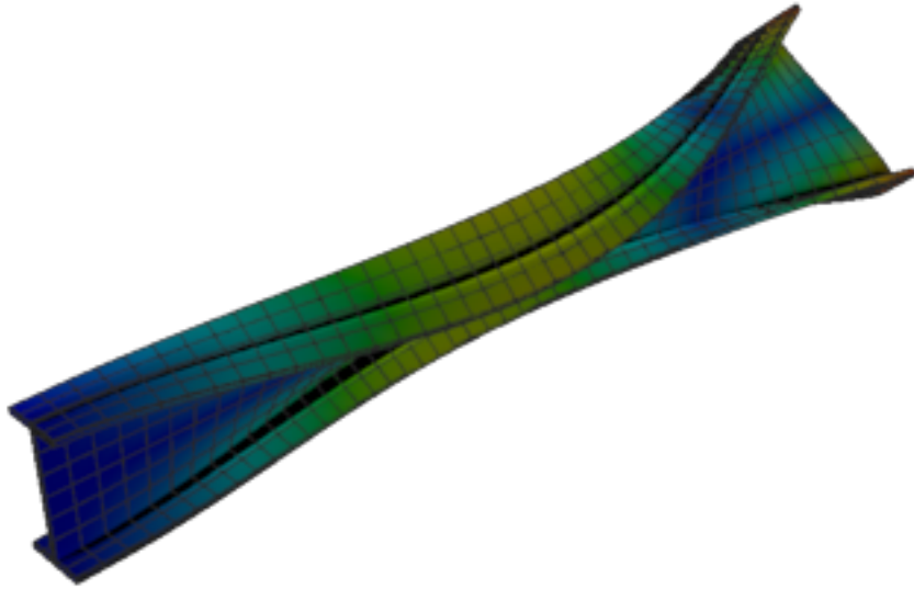
Figure 473: Calculix — mode 5, 97.594 Hz
