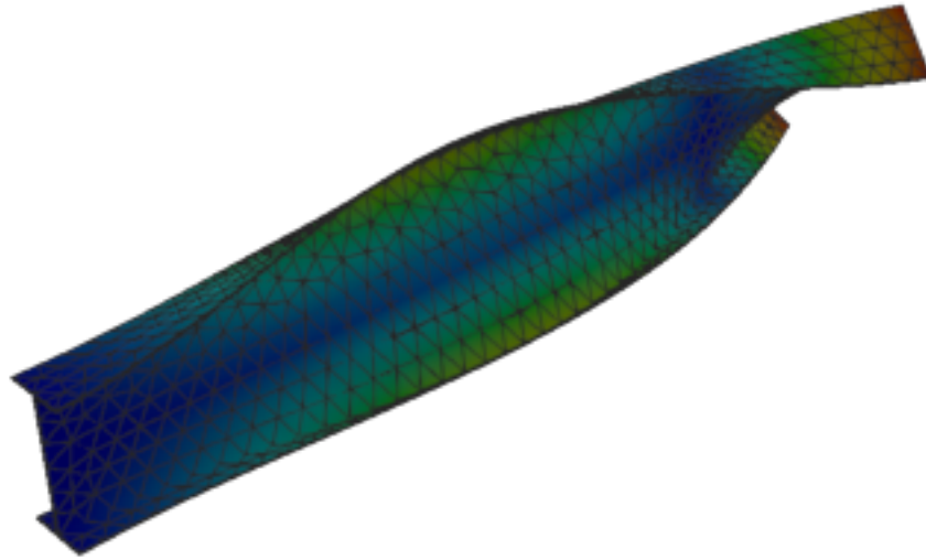
Figure 199: Code_Aster — mode 5, 95.871 Hz
