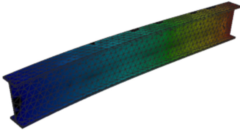
Figure 88: Calculix — mode 3, 52.249 Hz
