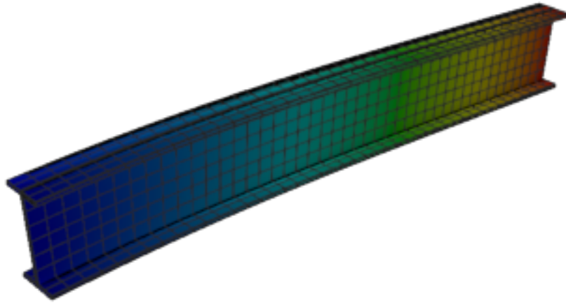
Figure 383: Calculix — mode 2, 51.665 Hz
