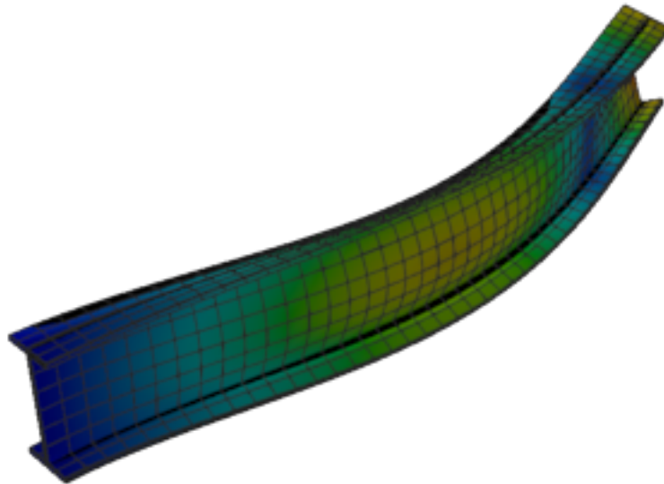
Figure 468: Abaqus — mode 4, 76.890 Hz
