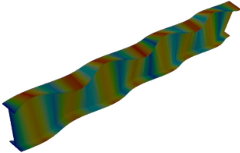
Figure 47: Code_Aster — mode 11, 185.976 Hz
