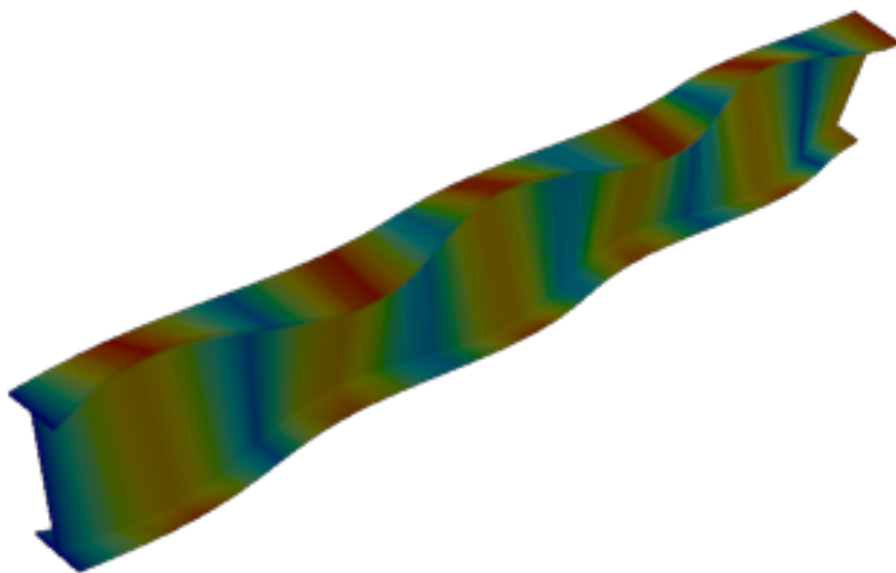
Figure 39: Code_Aster — mode 9, 135.600 Hz
