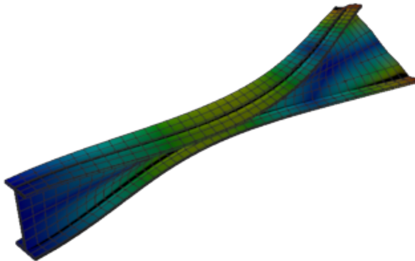
Figure 400: Abaqus — mode 8, 124.578 Hz
