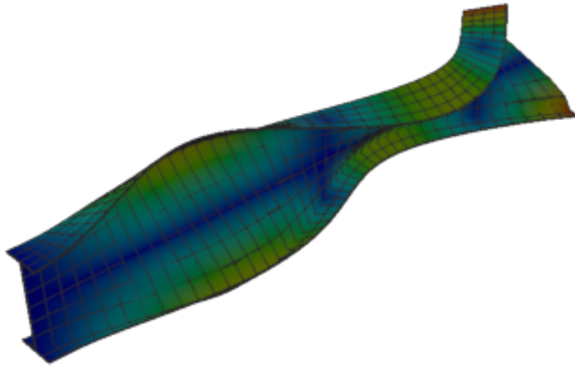
Figure 265: Abaqus — mode 11, 250.173 Hz
