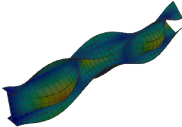
Figure 285: Abaqus — mode 9, 192.184 Hz
