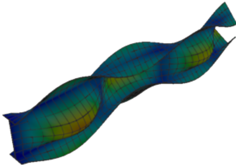
Figure 260: Sesam — mode 9, 191.999 Hz
