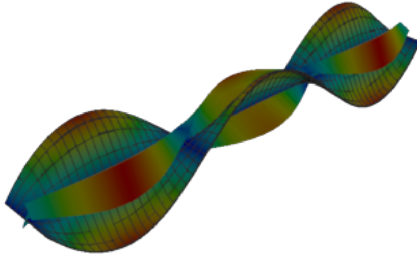
Figure 571: Sesam — mode 5, 114.982 Hz
