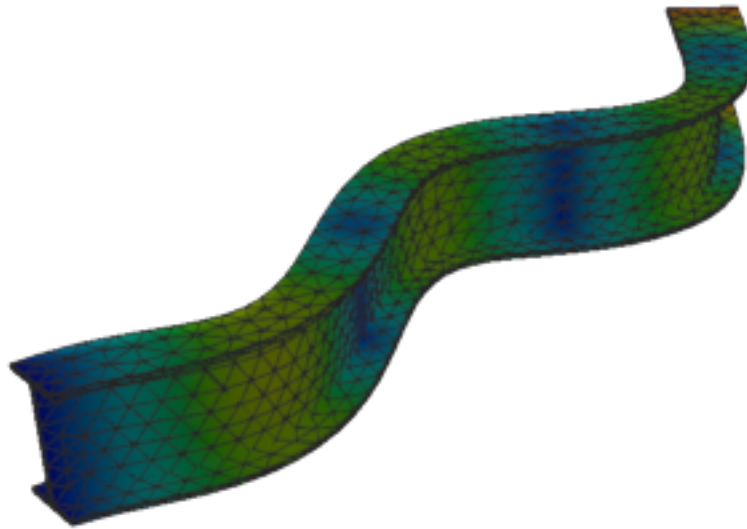
Figure 325: Code_Aster — mode 9, 528.489 Hz
