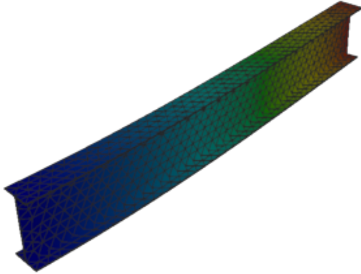
Figure 183: Code_Aster — mode 1, 12.757 Hz
