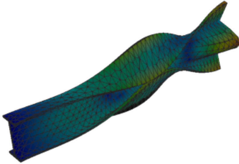
Figure 443: Sesam — mode 8, 178.114 Hz
