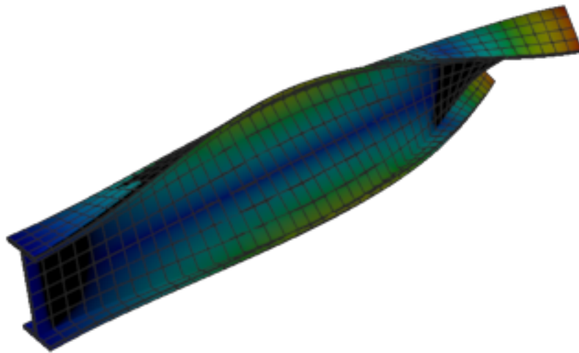
Figure 242: Calculix — mode 5, 96.037 Hz
