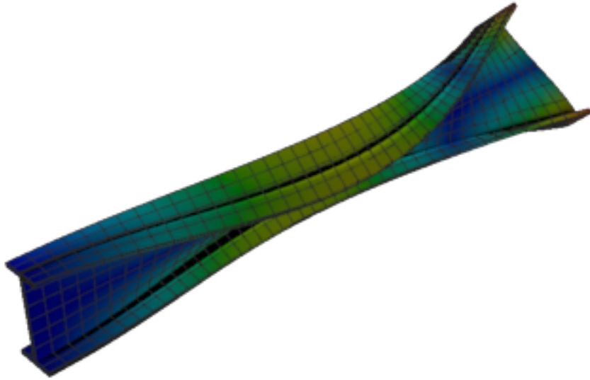
Figure 513: Calculix — mode 5, 97.391 Hz
