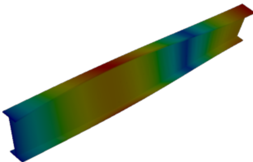
Figure 15: Code_Aster — mode 3, 36.752 Hz
