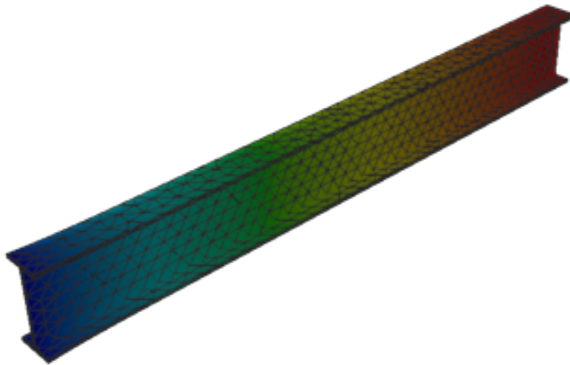
Figure 322: Sesam — mode 8, 432.347 Hz
