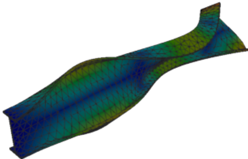
Figure 452: Abaqus — mode 11, 254.466 Hz
