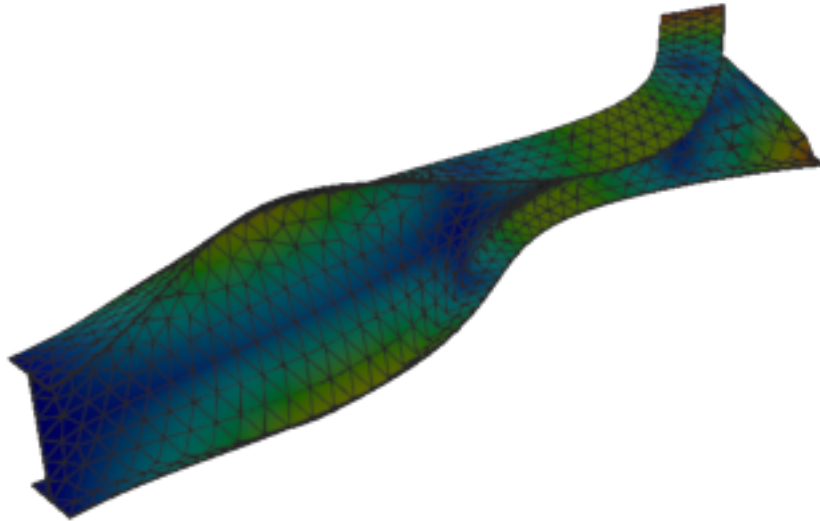
Figure 224: Sesam — mode 11, 250.240 Hz
