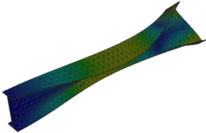
Figure 197: Abaqus — mode 5, 96.001 Hz
