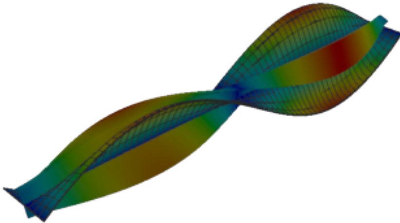
Figure 567: Code_Aster — mode 4, 100.176 Hz
