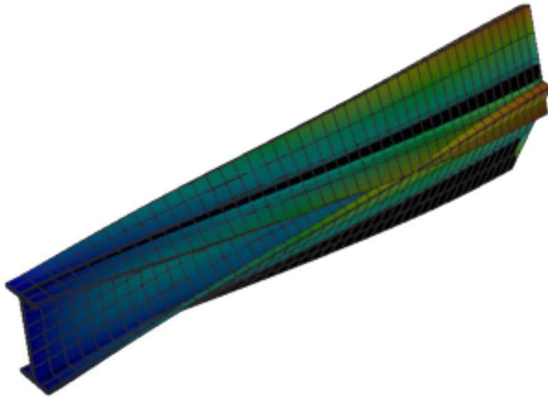
Figure 479: Sesam — mode 6, 130.865 Hz
