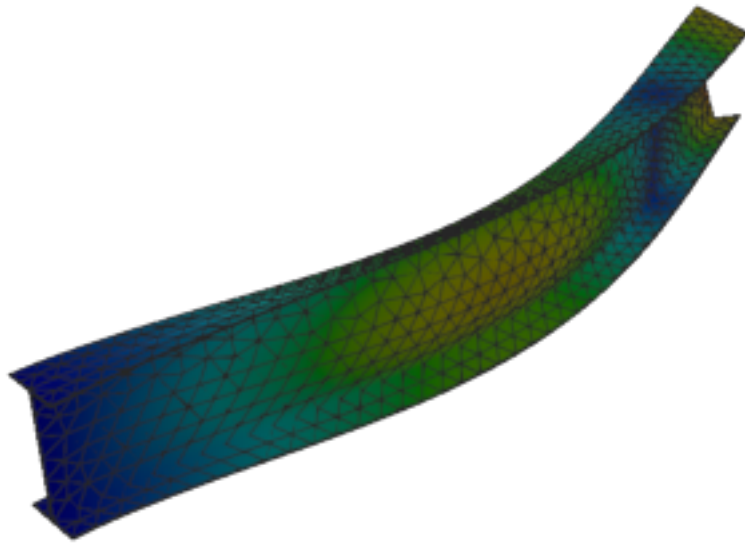
Figure 193: Abaqus — mode 4, 75.145 Hz
