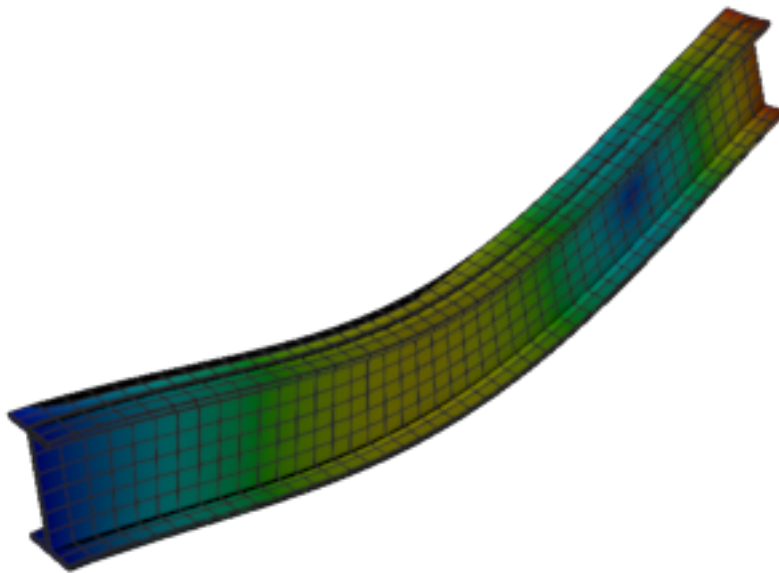
Figure 395: Calculix — mode 6, 258.286 Hz
