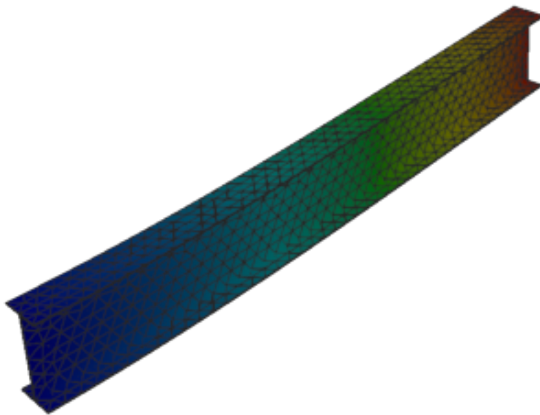
Figure 89: Code_Aster — mode 3, 52.193 Hz
