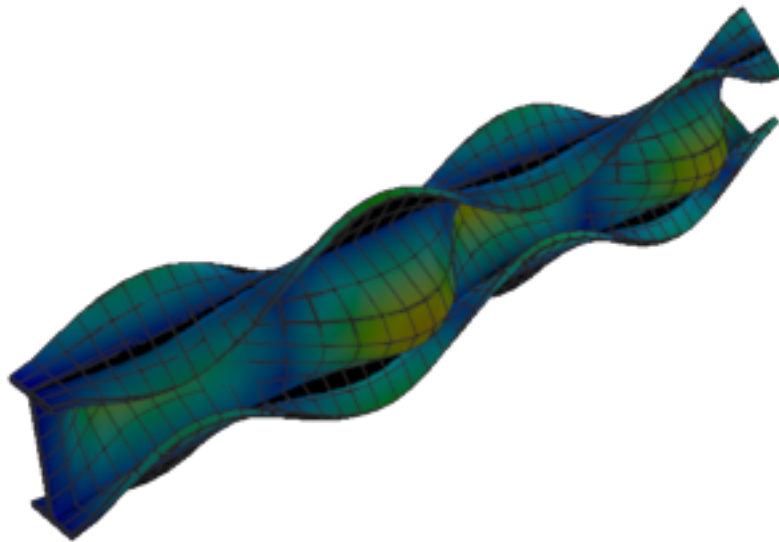
Figure 494: Code_Aster — mode 10, 251.347 Hz
