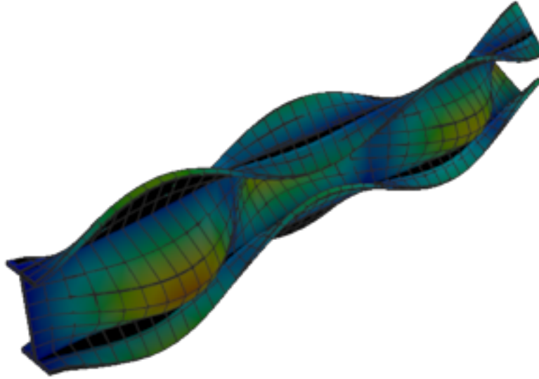
Figure 491: Sesam — mode 9, 201.904 Hz
