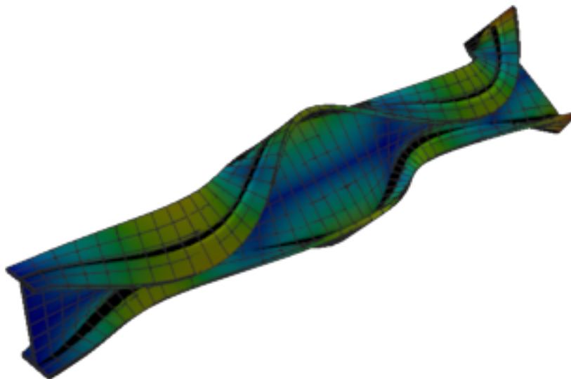
Figure 376: Calculix — mode 11, 500.931 Hz
