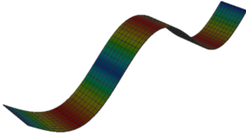
Figure 543: Code_Aster — mode 3, 13.829 Hz
