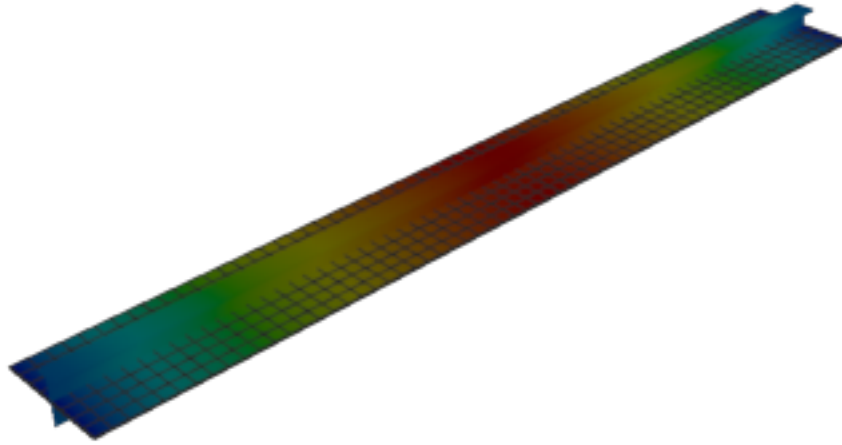
Figure 580: Code_Aster — displacement
