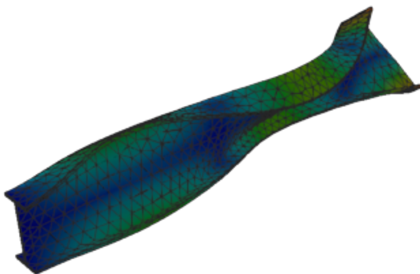
Figure 332: Calculix — mode 11, 617.646 Hz
