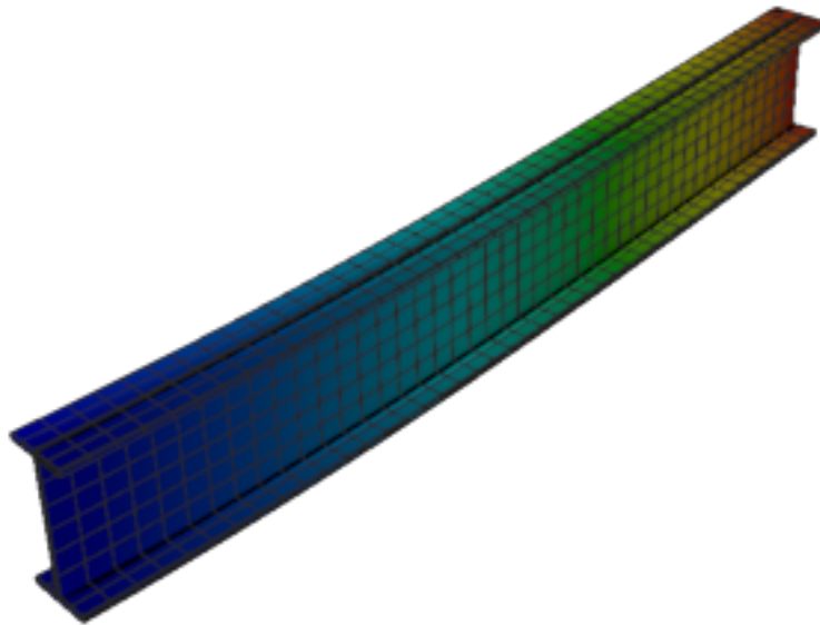
Figure 500: Abaqus — mode 1, 12.943 Hz
