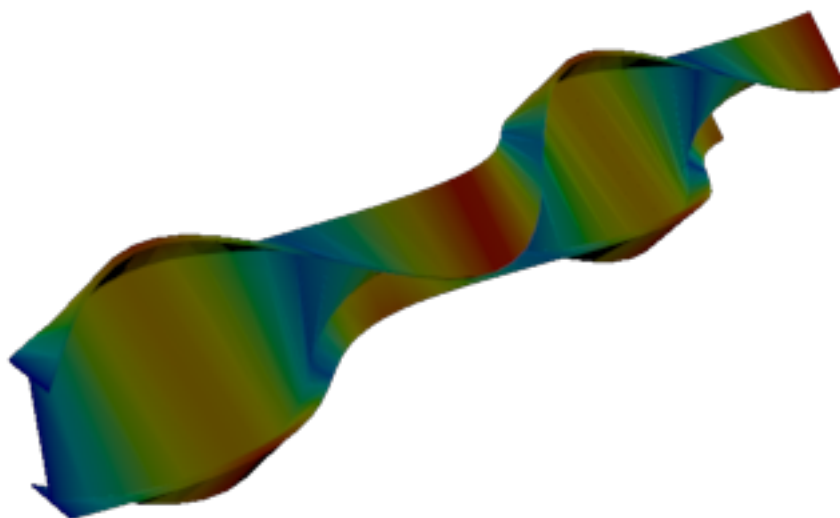
Figure 32: Sesam — mode 7, 85.947 Hz
