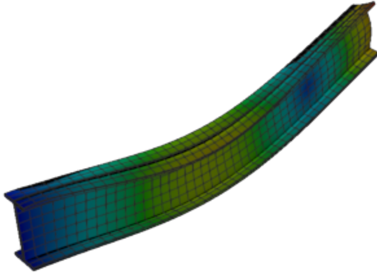
Figure 405: Code_Aster — mode 9, 254.838 Hz
