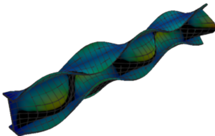
Figure 262: Calculix — mode 10, 238.389 Hz
