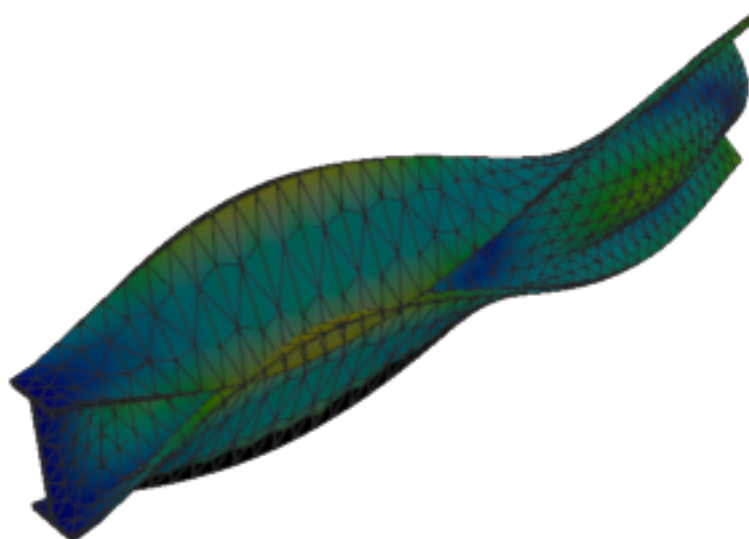
Figure 438: Code_Aster — mode 7, 154.802 Hz
