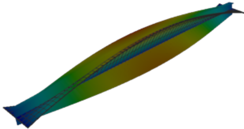
Figure 565: Sesam — mode 3, 92.540 Hz
