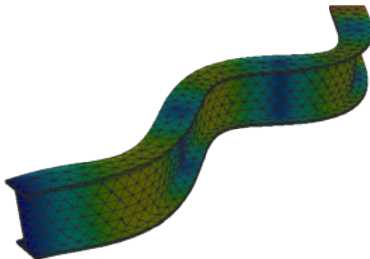
Figure 323: Abaqus — mode 9, 500.864 Hz
