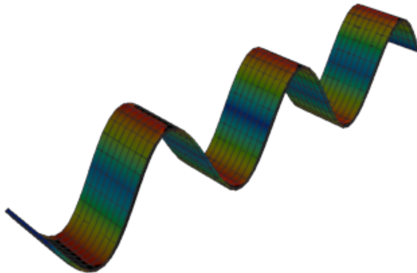
Figure 554: Calculix — mode 6, 55.494 Hz
