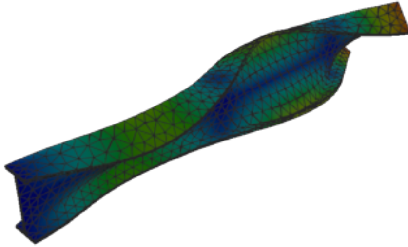
Figure 327: Abaqus — mode 10, 534.263 Hz
