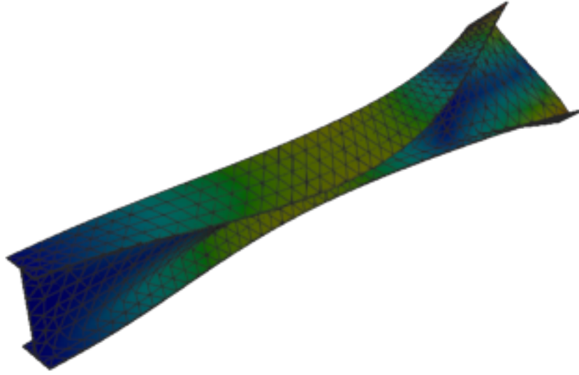
Figure 96: Sesam — mode 5, 101.756 Hz
