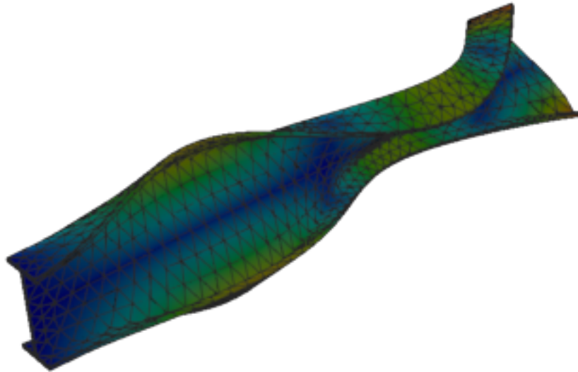
Figure 455: Sesam — mode 11, 254.466 Hz
