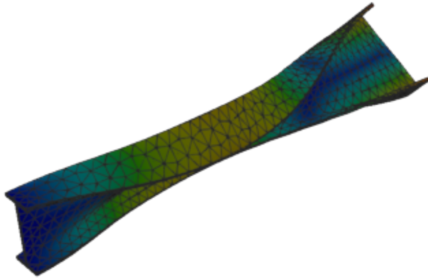
Figure 315: Abaqus — mode 7, 285.051 Hz
