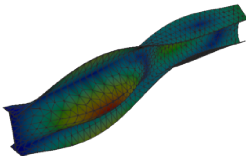
Figure 101: Code_Aster — mode 7, 144.895 Hz
