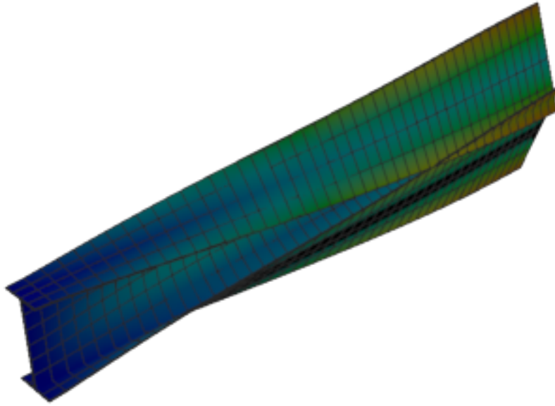
Figure 247: Code_Aster — mode 6, 124.987 Hz
