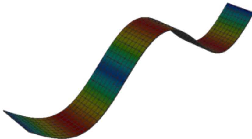
Figure 541: Abaqus — mode 3, 13.866 Hz
