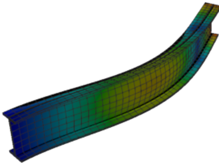
Figure 390: Code_Aster — mode 4, 82.296 Hz
