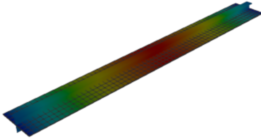
Figure 581: Sesam — displacement
