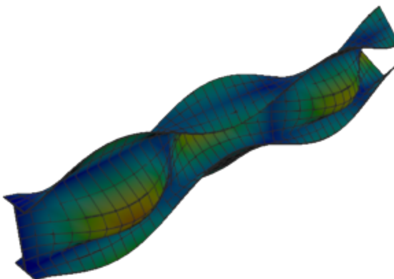
Figure 149: Code_Aster — mode 9, 193.960 Hz
