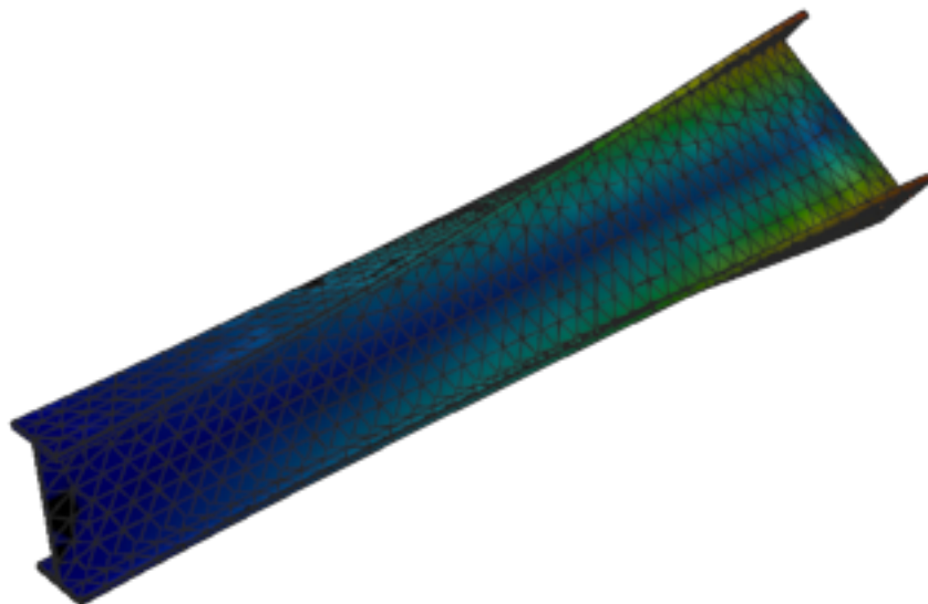
Figure 186: Calculix — mode 2, 19.525 Hz
