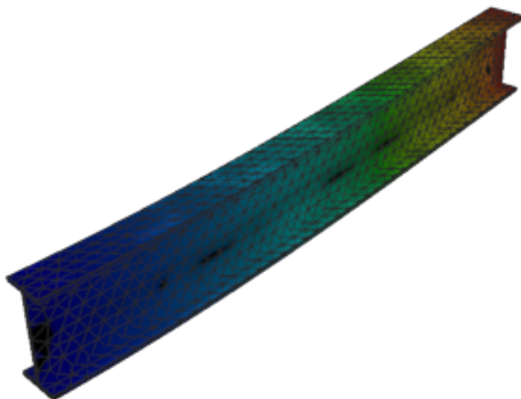
Figure 82: Calculix — mode 1, 13.725 Hz
