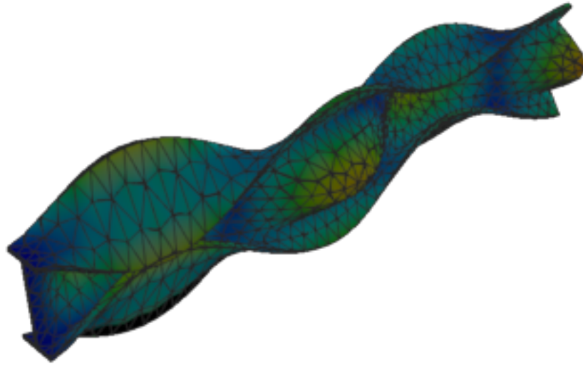
Figure 445: Calculix — mode 9, 219.501 Hz
