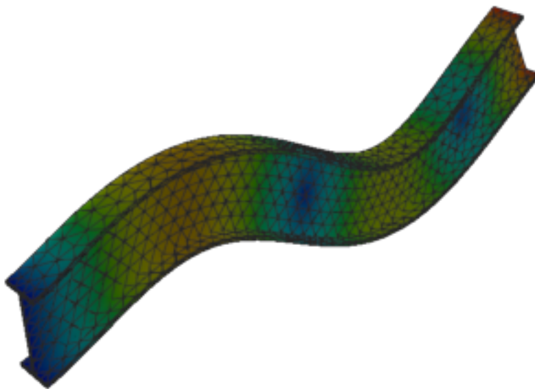
Figure 331: Abaqus — mode 11, 596.780 Hz
