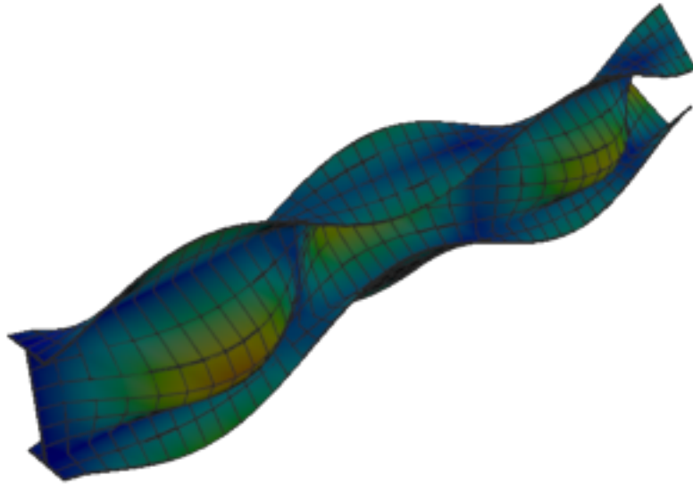
Figure 257: Abaqus — mode 9, 192.184 Hz
