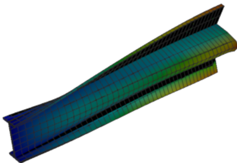
Figure 516: Calculix — mode 6, 130.814 Hz
