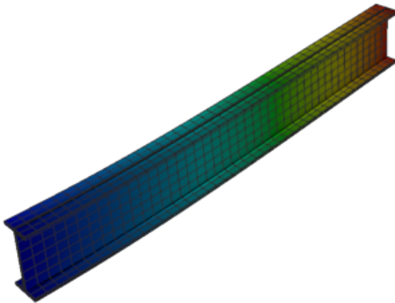
Figure 346: Sesam — mode 3, 50.618 Hz
