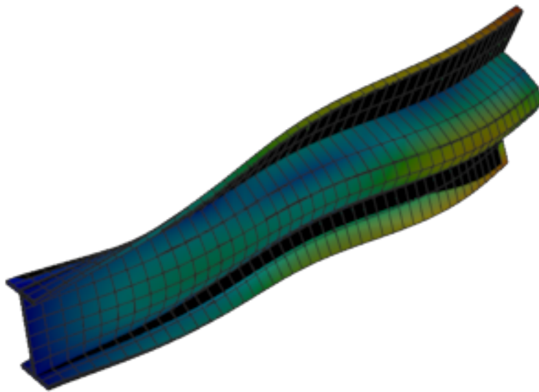
Figure 404: Calculix — mode 9, 439.038 Hz
