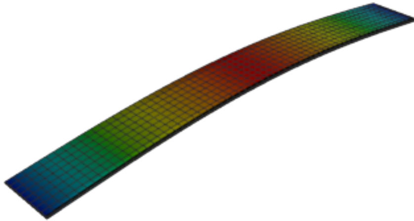
Figure 576: Calculix — displacement
