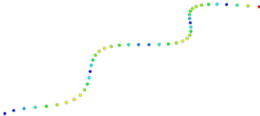
Figure 38: Calculix — mode 9, 728.596 Hz
