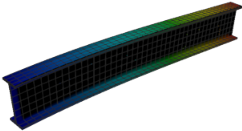
Figure 234: Calculix — mode 3, 51.980 Hz
