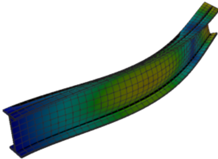
Figure 511: Code_Aster — mode 4, 76.687 Hz
