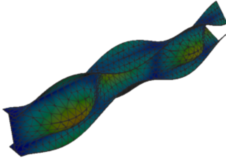
Figure 108: Sesam — mode 9, 191.533 Hz
