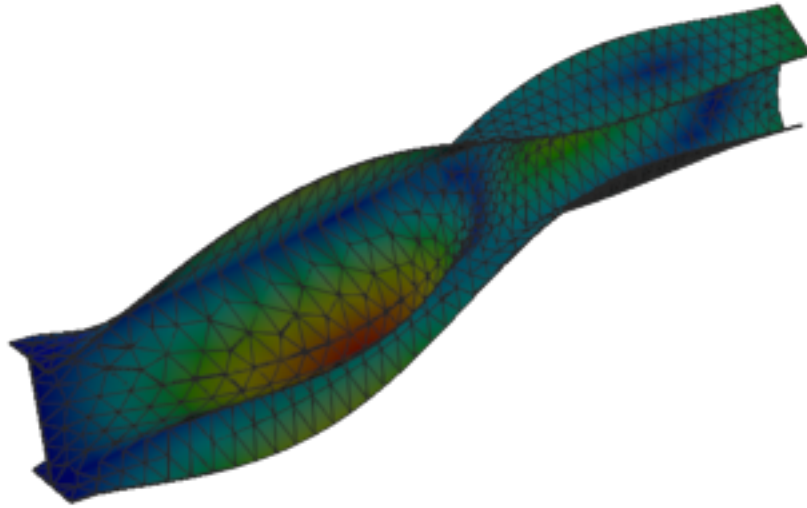
Figure 207: Code_Aster — mode 7, 142.359 Hz
