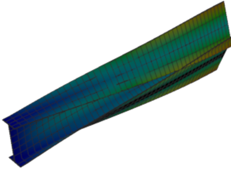
Figure 279: Abaqus — mode 6, 125.001 Hz
