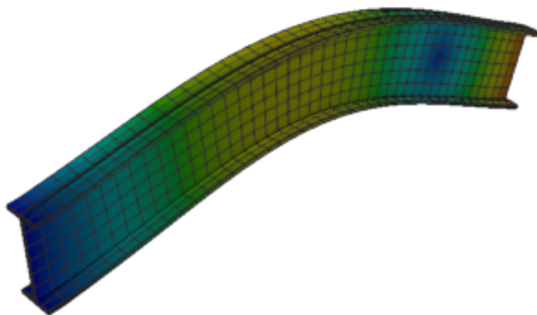
Figure 497: Calculix — mode 11, 252.917 Hz
