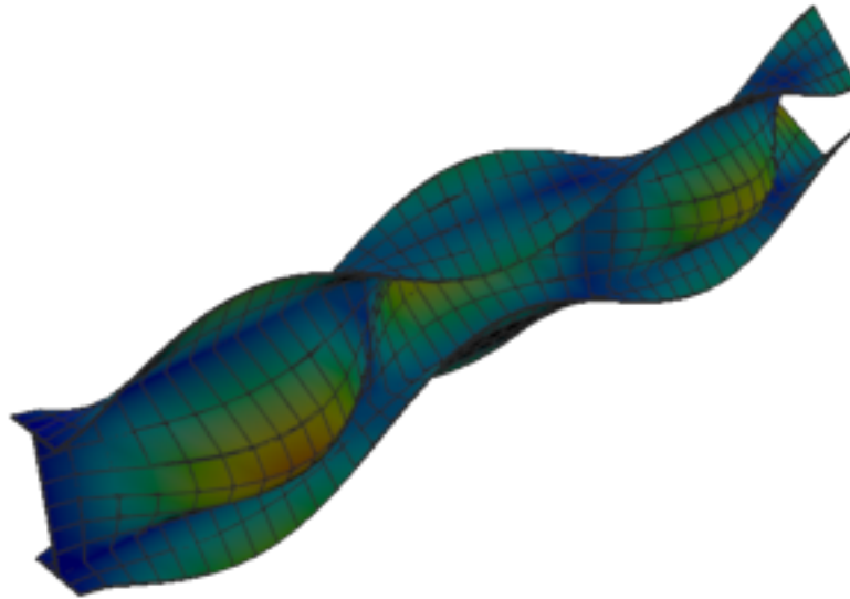
Figure 147: Abaqus — mode 9, 198.748 Hz
