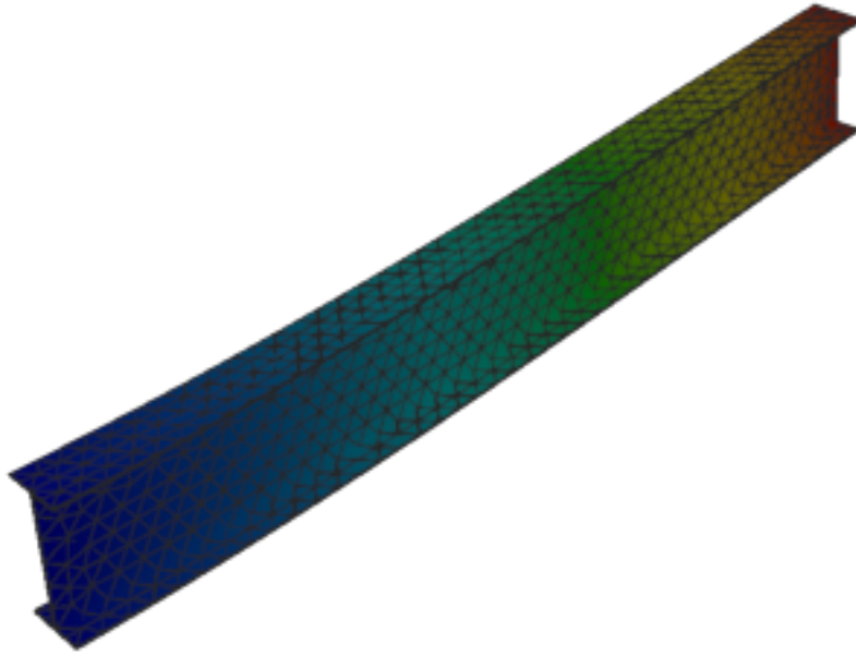
Figure 191: Code_Aster — mode 3, 51.970 Hz
