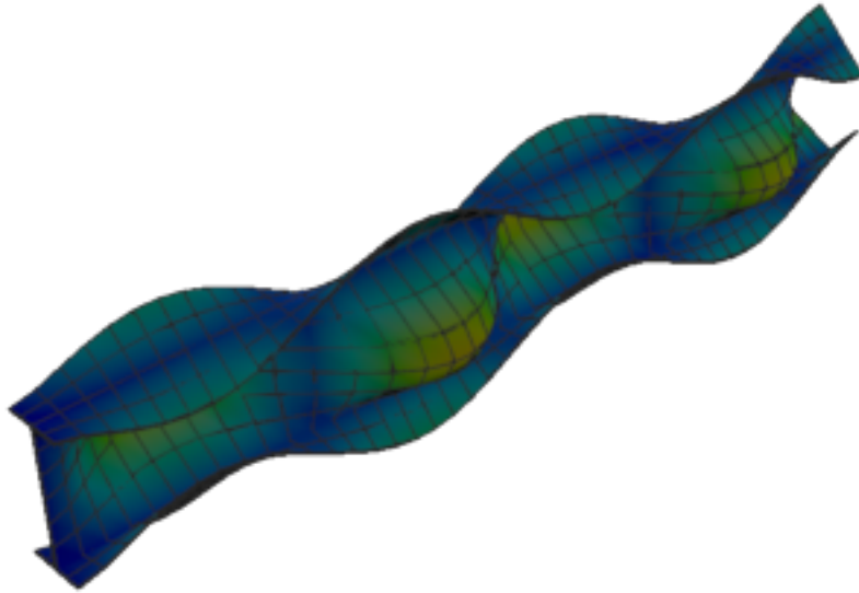
Figure 263: Code_Aster — mode 10, 232.628 Hz
