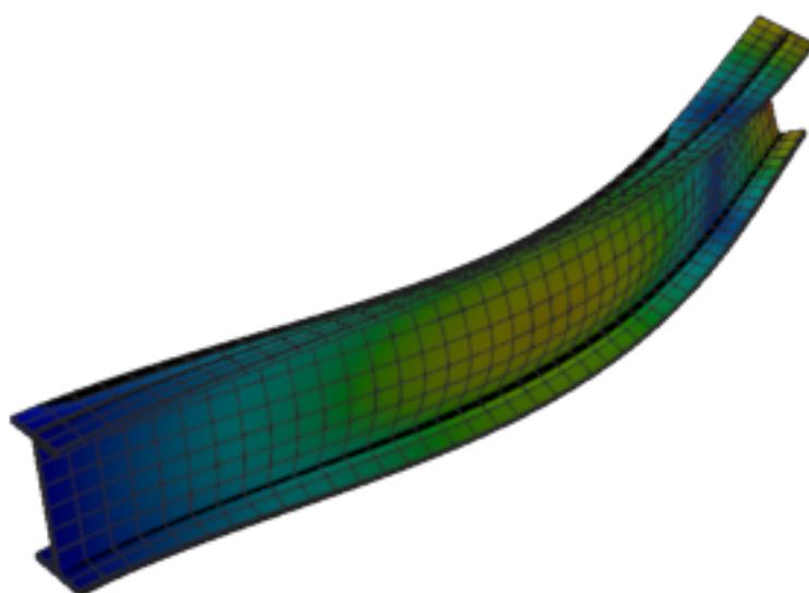
Figure 470: Code_Aster — mode 4, 76.890 Hz
