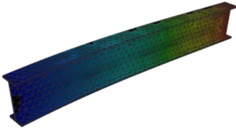
Figure 190: Calculix — mode 3, 51.974 Hz
