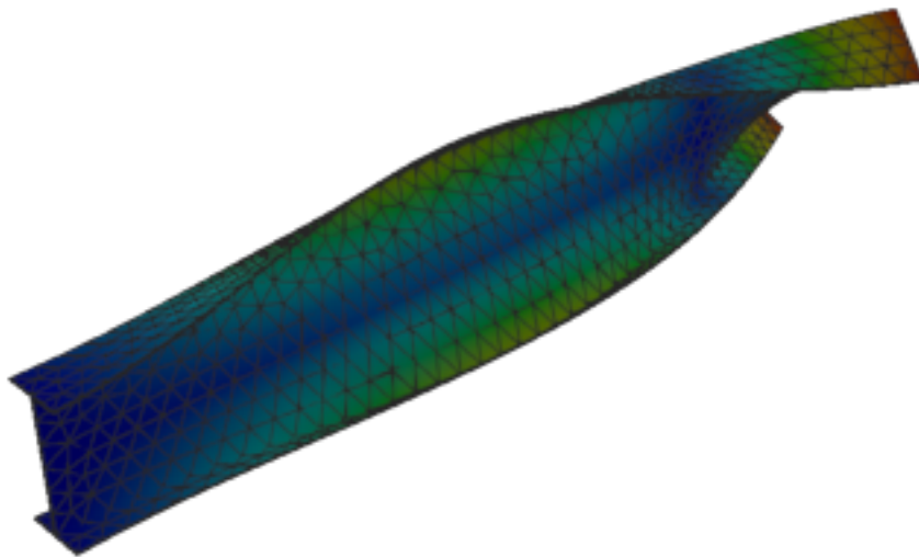
Figure 95: Code_Aster — mode 5, 102.010 Hz
