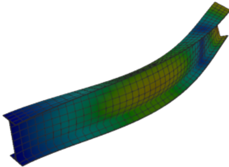
Figure 275: Abaqus — mode 4, 75.149 Hz
