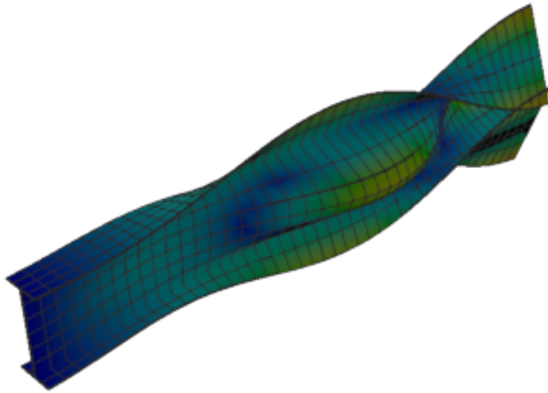
Figure 253: Abaqus — mode 8, 165.849 Hz
