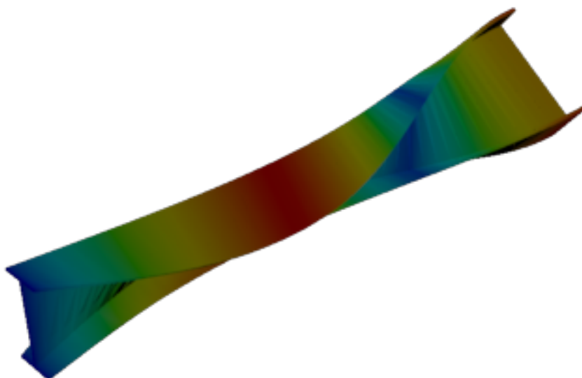
Figure 16: Sesam — mode 3, 36.752 Hz
