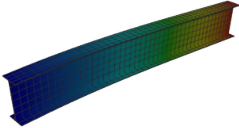
Figure 126: Sesam — mode 3, 51.991 Hz
