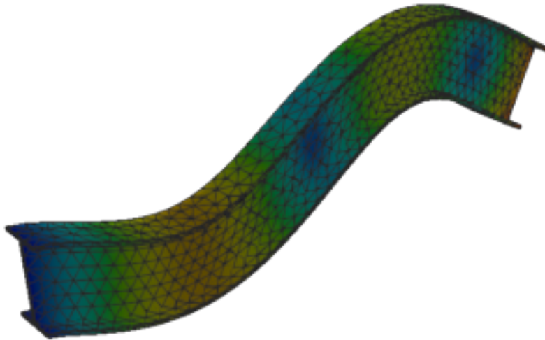
Figure 328: Calculix — mode 10, 601.943 Hz
