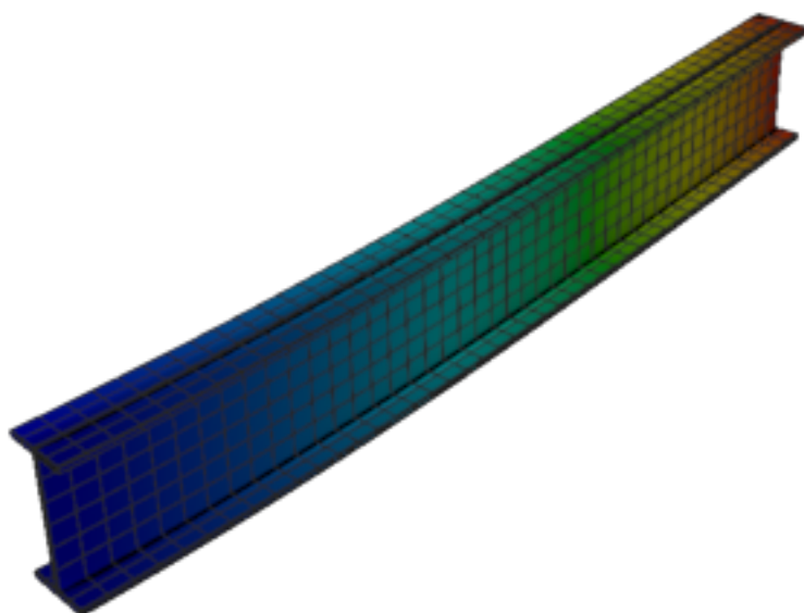
Figure 458: Code_Aster — mode 1, 12.955 Hz
