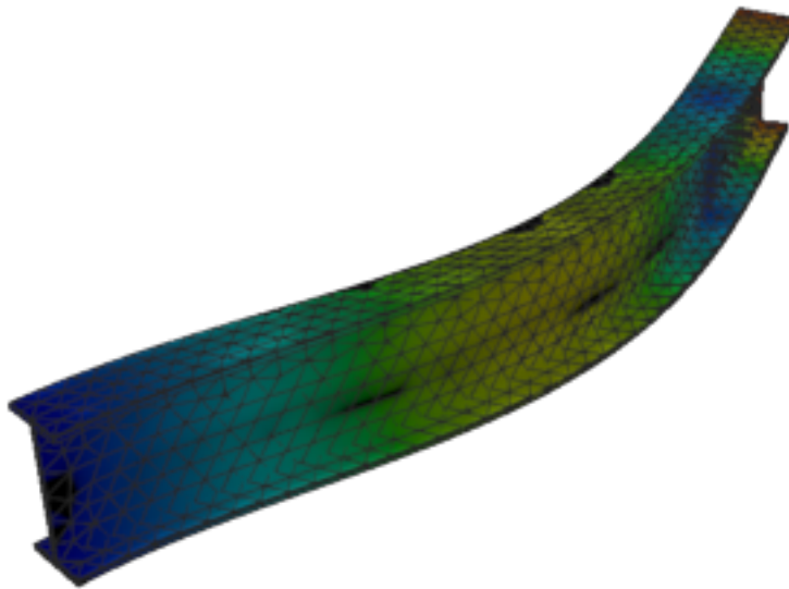
Figure 91: Calculix — mode 4, 83.709 Hz
