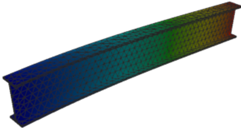
Figure 298: Sesam — mode 2, 51.542 Hz
