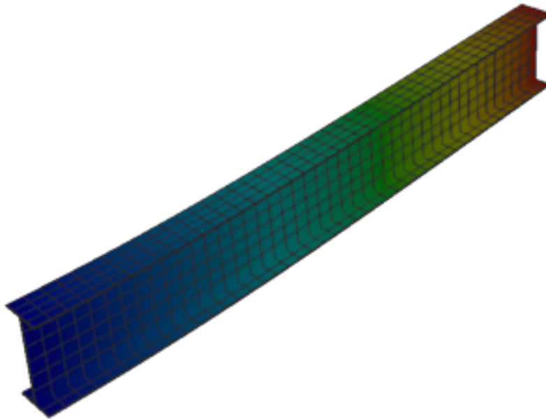
Figure 123: Abaqus — mode 3, 51.998 Hz
