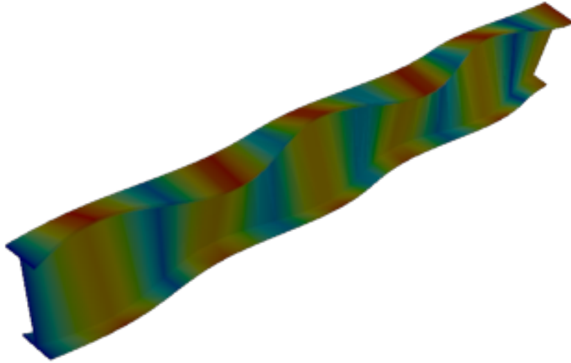
Figure 76: Abaqus — mode 9, 118.648 Hz
