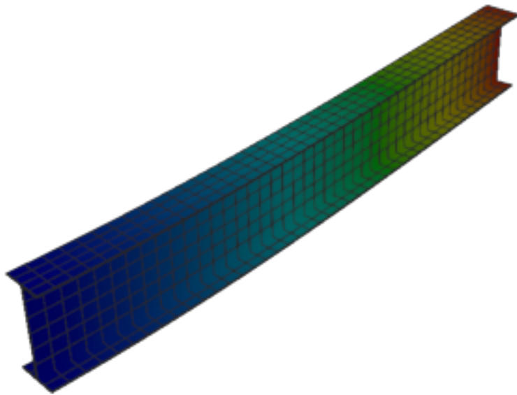
Figure 225: Abaqus — mode 1, 12.758 Hz
