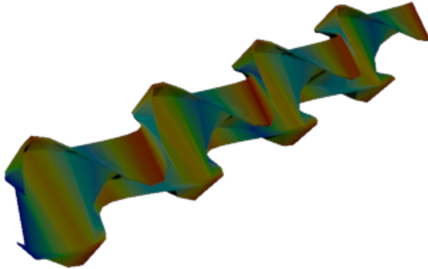
Figure 48: Sesam — mode 11, 185.976 Hz
