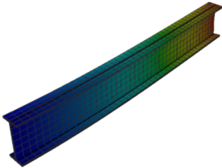
Figure 379: Abaqus — mode 1, 12.514 Hz
