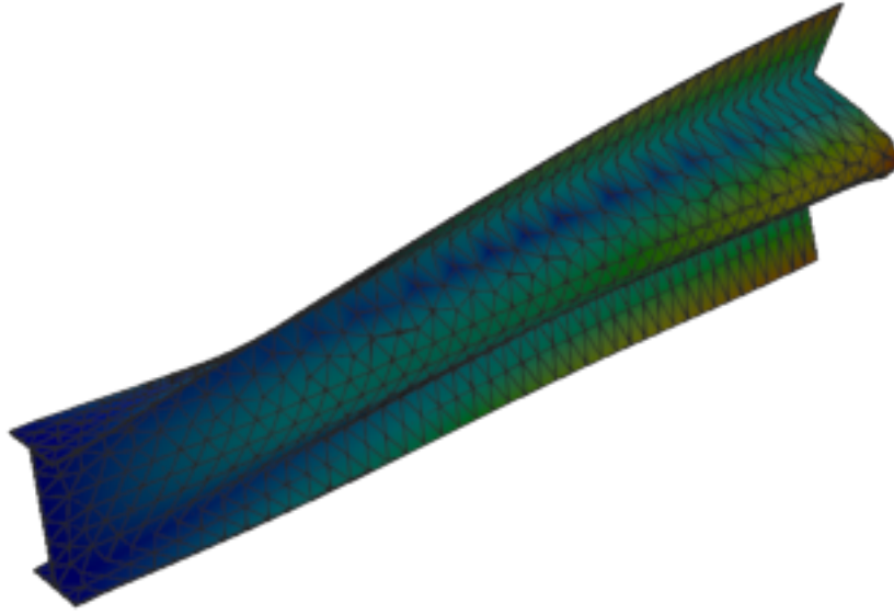
Figure 203: Code_Aster — mode 6, 125.087 Hz
