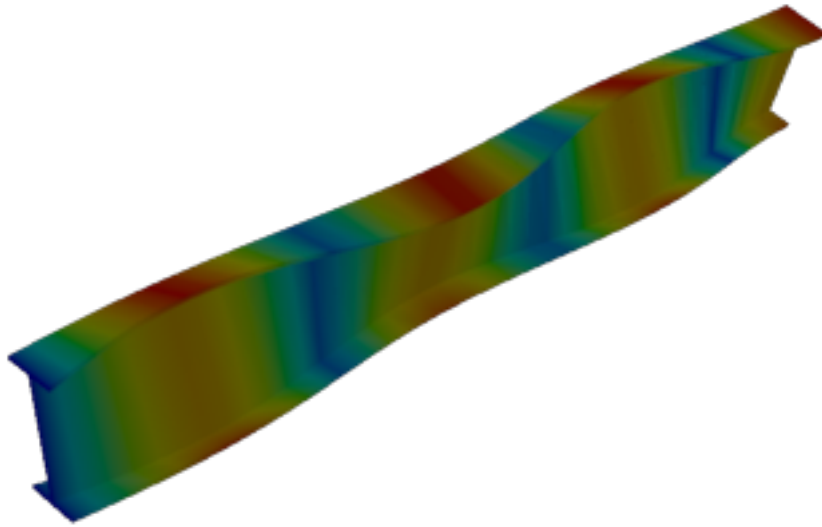
Figure 25: Abaqus — mode 6, 75.296 Hz
