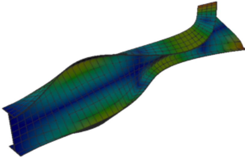
Figure 155: Abaqus — mode 11, 252.486 Hz
