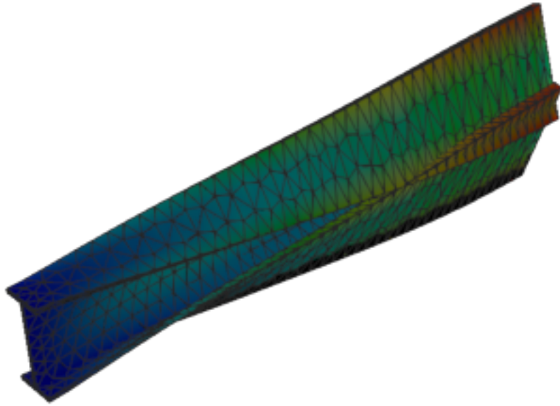
Figure 435: Sesam — mode 6, 132.478 Hz
