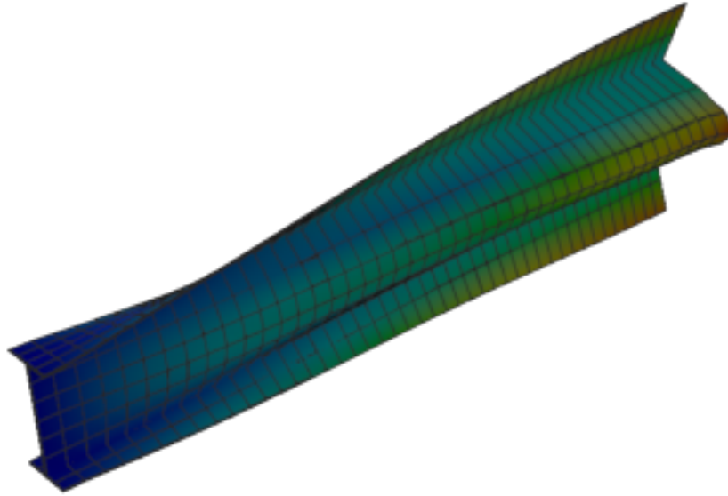
Figure 138: Sesam — mode 6, 125.116 Hz
