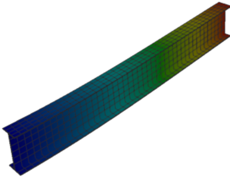
Figure 235: Code_Aster — mode 3, 51.970 Hz
