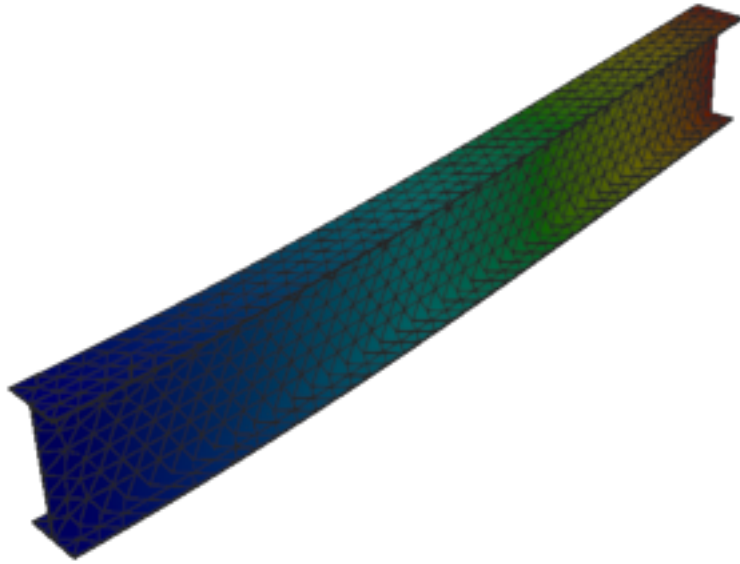
Figure 181: Abaqus — mode 1, 12.756 Hz
