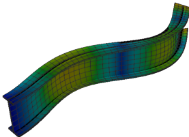
Figure 355: Abaqus — mode 6, 223.139 Hz
