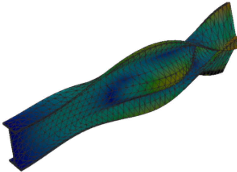
Figure 440: Abaqus — mode 8, 178.118 Hz
