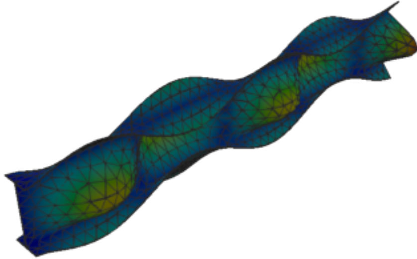
Figure 110: Code_Aster — mode 10, 235.115 Hz
