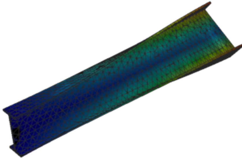
Figure 85: Calculix — mode 2, 36.690 Hz
