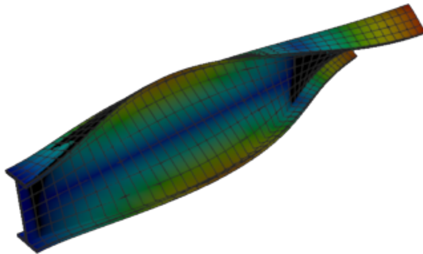
Figure 172: Calculix — mode 7, 365.100 Hz
