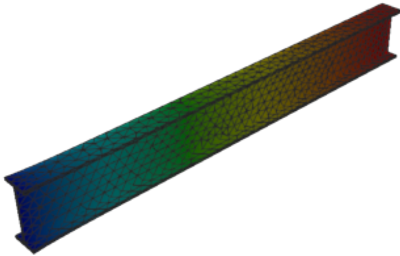
Figure 320: Calculix — mode 8, 432.360 Hz
