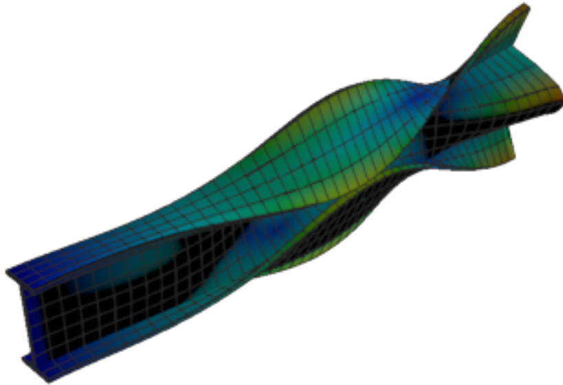
Figure 284: Calculix — mode 8, 165.981 Hz
