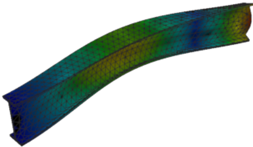
Figure 194: Calculix — mode 4, 75.185 Hz
