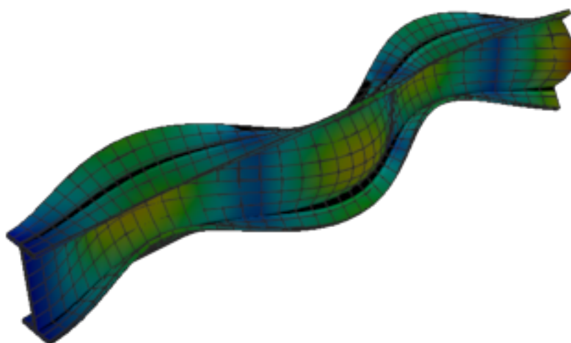
Figure 368: Calculix — mode 9, 407.869 Hz
