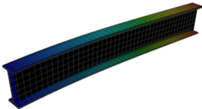
Figure 162: Calculix — mode 2, 53.262 Hz
