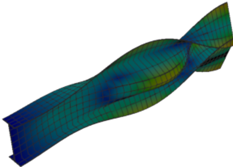
Figure 145: Code_Aster — mode 8, 167.974 Hz
