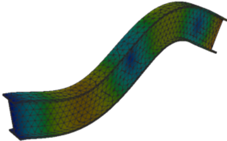
Figure 334: Sesam — mode 11, 598.200 Hz
