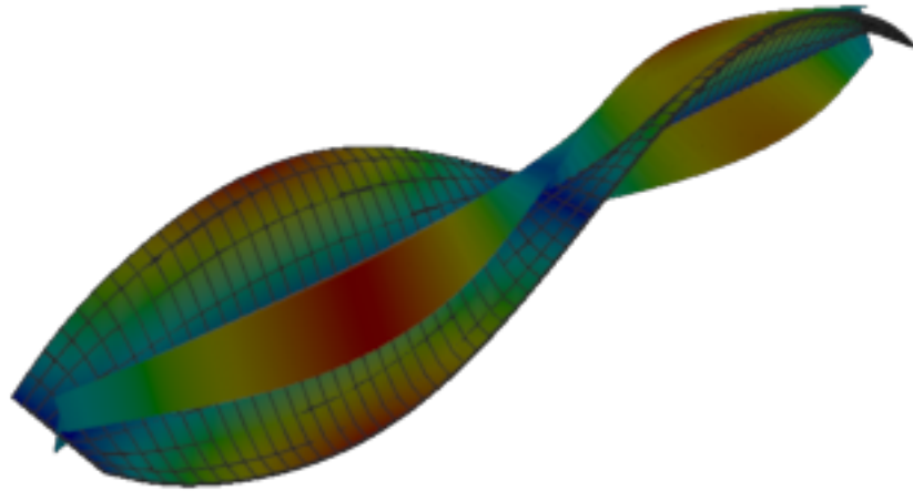
Figure 566: Abaqus — mode 4, 106.618 Hz
