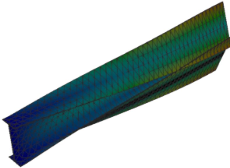
Figure 204: Sesam — mode 6, 125.173 Hz
