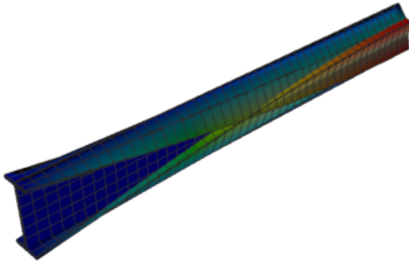
Figure 406: Abaqus — mode 10, 159.952 Hz
