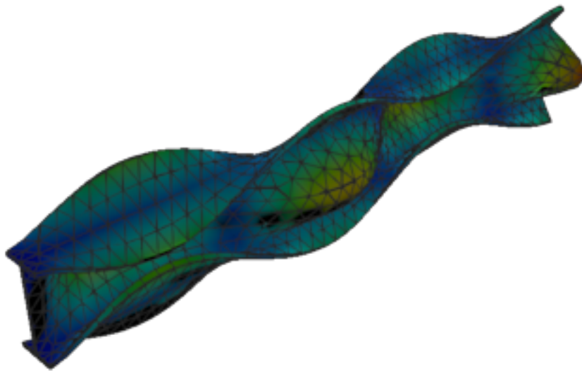
Figure 214: Calculix — mode 9, 194.014 Hz
