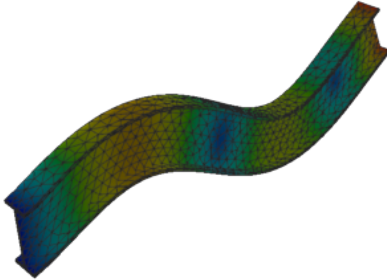
Figure 329: Code_Aster — mode 10, 601.586 Hz
