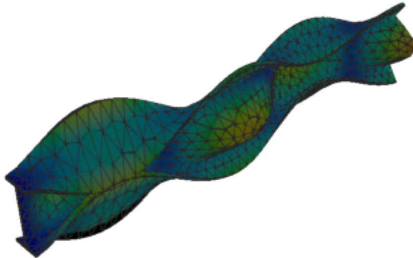
Figure 446: Code_Aster — mode 9, 219.497 Hz
