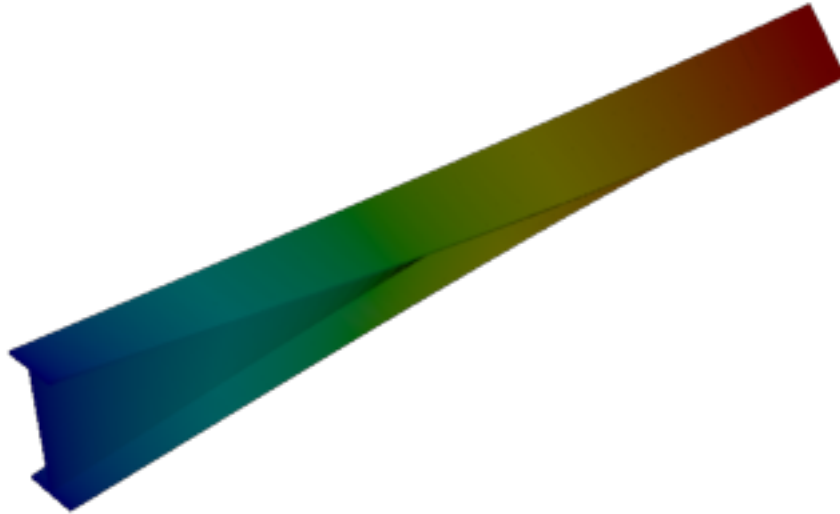
Figure 8: Sesam — mode 1, 12.245 Hz
