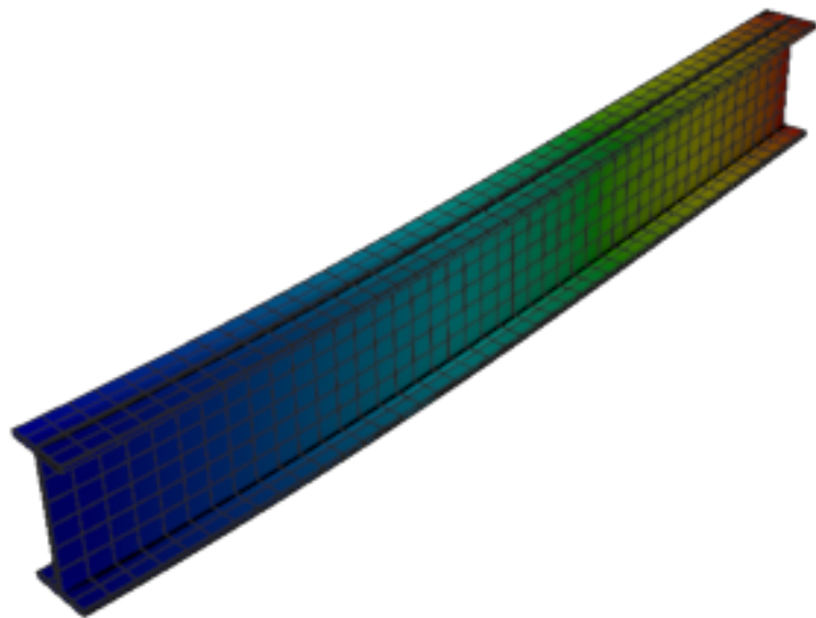
Figure 380: Calculix — mode 1, 14.302 Hz
