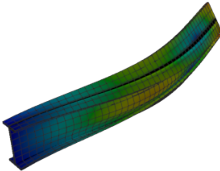
Figure 394: Abaqus — mode 6, 74.866 Hz
