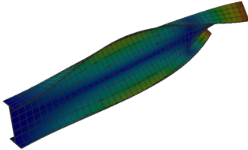
Figure 134: Sesam — mode 5, 95.930 Hz
