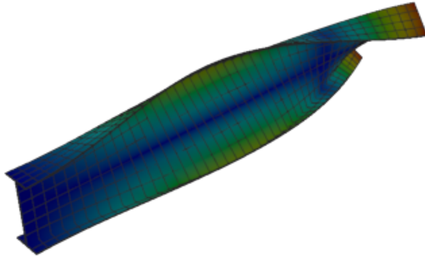
Figure 243: Code_Aster — mode 5, 95.889 Hz
