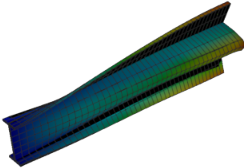
Figure 477: Calculix — mode 6, 131.365 Hz
