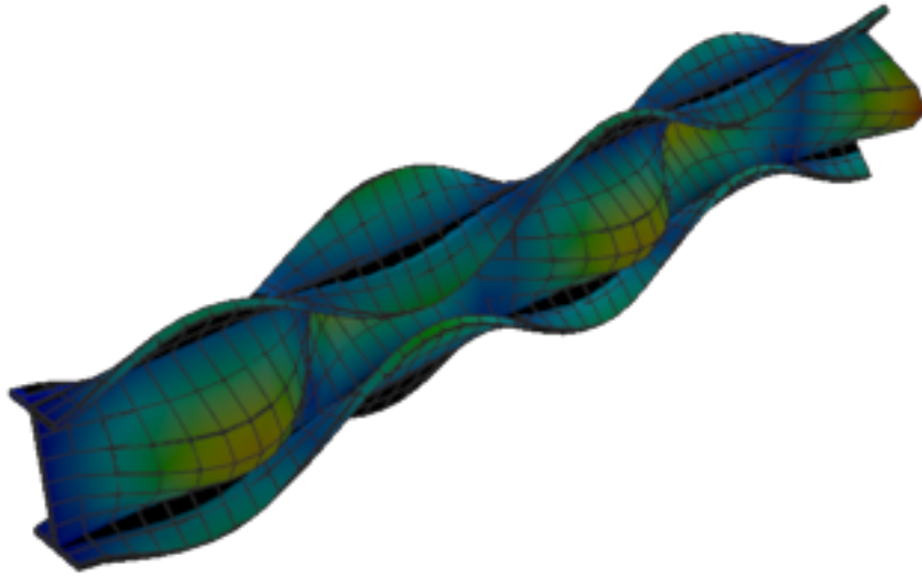
Figure 493: Calculix — mode 10, 251.347 Hz
