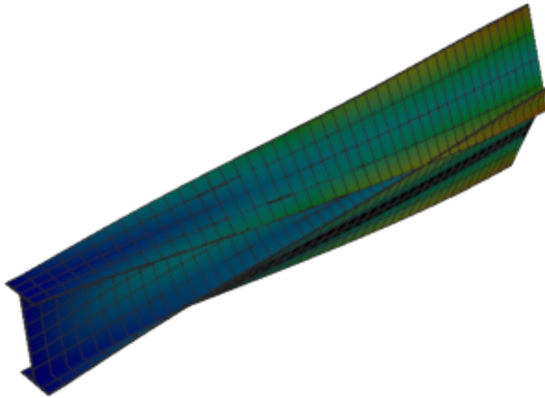
Figure 248: Sesam — mode 6, 124.987 Hz
