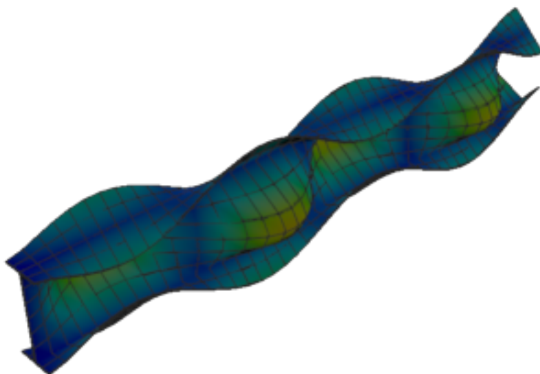
Figure 261: Abaqus — mode 10, 232.867 Hz
