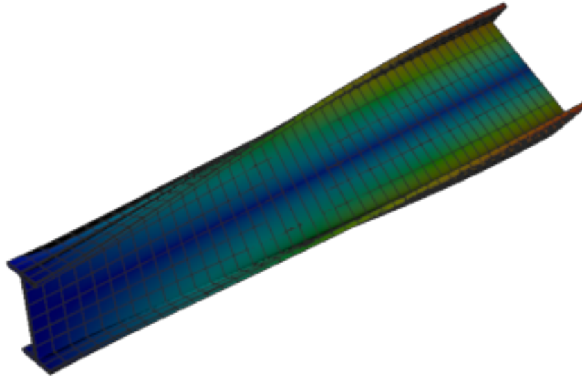
Figure 389: Calculix — mode 4, 116.873 Hz
