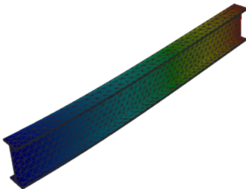
Figure 422: Code_Aster — mode 3, 50.540 Hz
