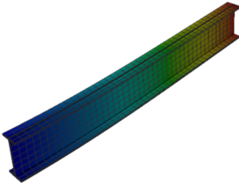
Figure 345: Code_Aster — mode 3, 50.825 Hz
