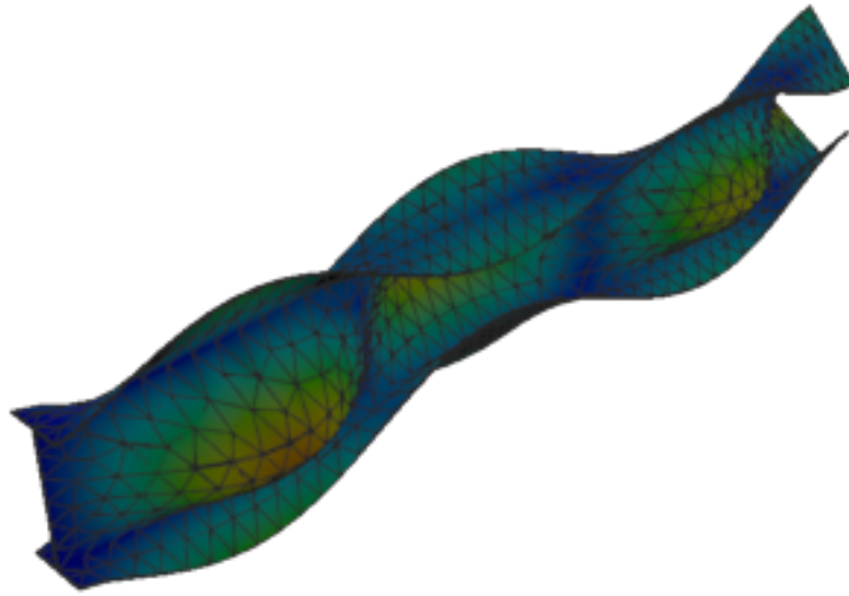
Figure 213: Abaqus — mode 9, 192.840 Hz
