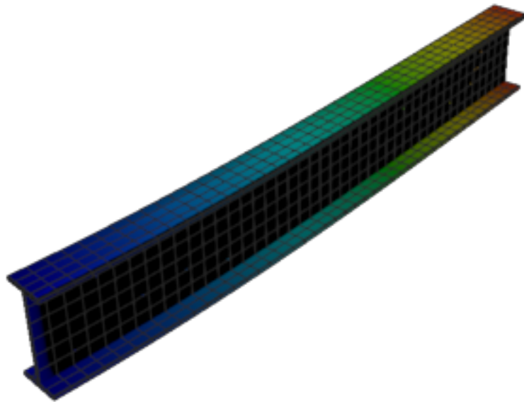
Figure 270: Calculix — mode 1, 12.756 Hz
