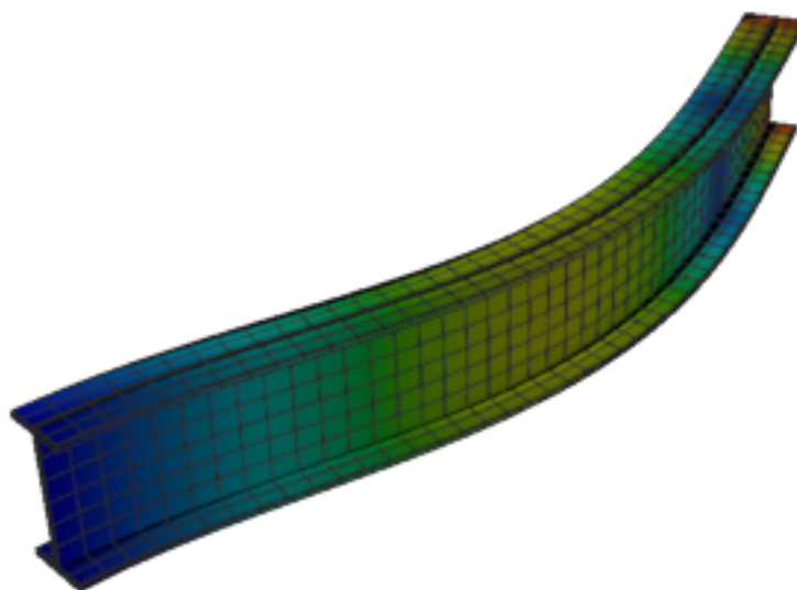
Figure 386: Calculix — mode 3, 88.233 Hz
