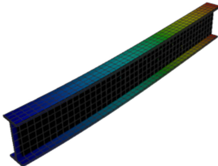
Figure 160: Calculix — mode 1, 14.256 Hz
