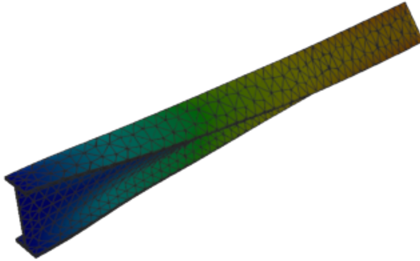
Figure 305: Code_Aster — mode 4, 116.512 Hz
