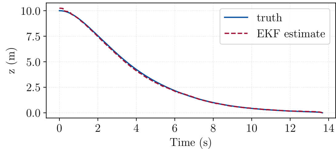
EKF estimate vs truth (closed loop on estimate)
