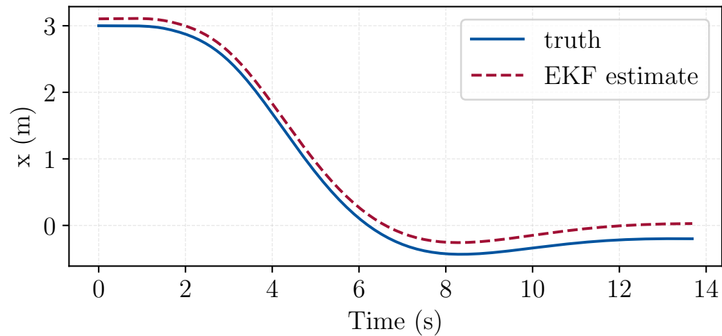
EKF estimate vs truth (closed loop on estimate)
