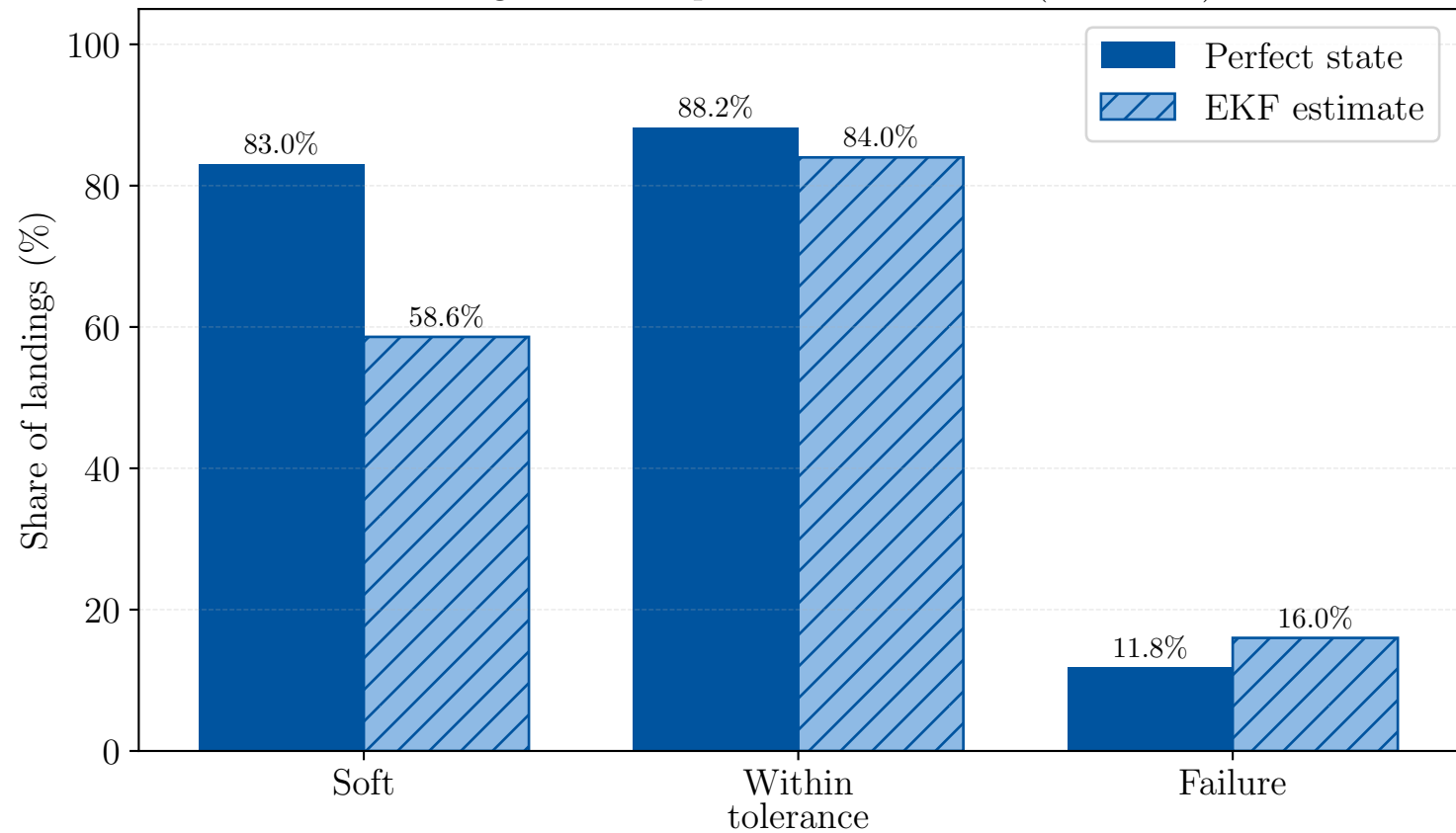
Landing outcomes: perfect state vs EKF ( N = 1000 )
