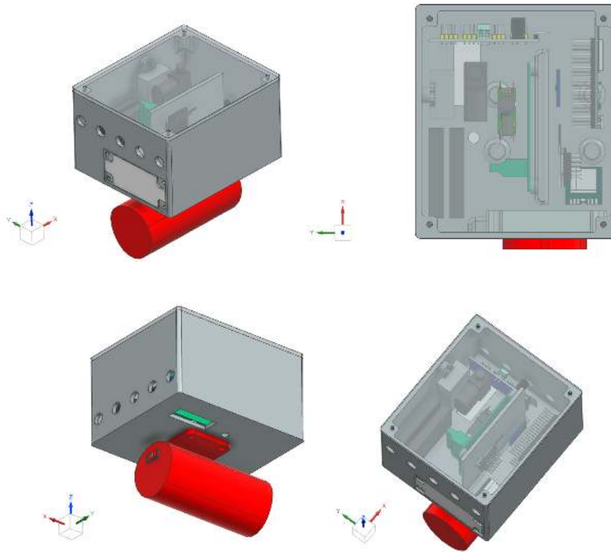
Figure 26: Electronics Housing
