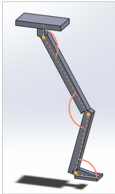
Figure 63: Hind Limb Simplified Model with Notated Joint Angles
