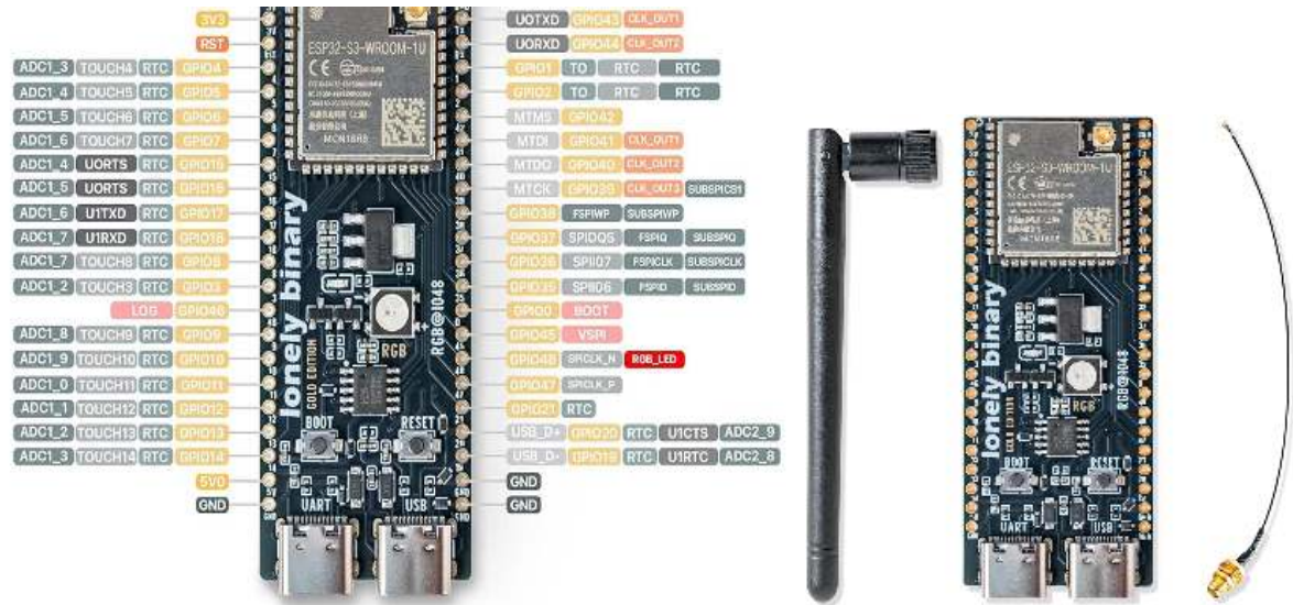
Figure 47: ESP32-S3-WROOM-1U
