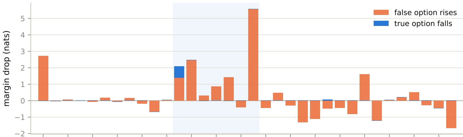
a. Image->Question knockout, per layer (n = 7790 correct items)
