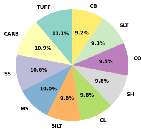
Lithology Distribution
