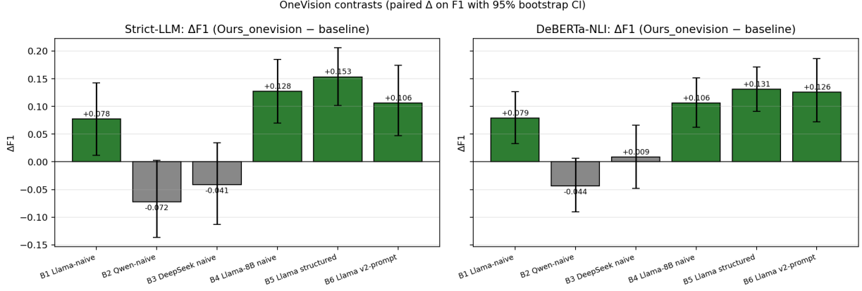
Figure 3: Paired \Delta F_1 (ONEVISION – baseline) on each baseline, under both judges. Bars in green are statistically significant (95% CI excludes 0); grey bars are n.s. (CI crosses 0). ONEVISION significantly beats four of six baselines under both judges (B1, B4, B5, B6 ); ties two (B2 and B3, both n.s.). The B6 contrast is the architecture-vs.-prompt control and is the headline of this paper.
