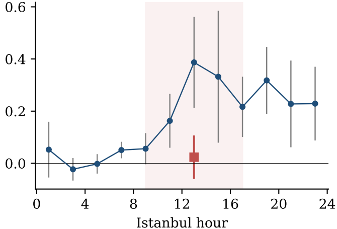
(b) large-trade flow toward the band, \hat{\theta}
