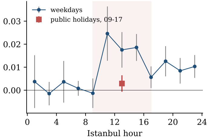
(a) price side: \hat{\kappa} per 5 min
