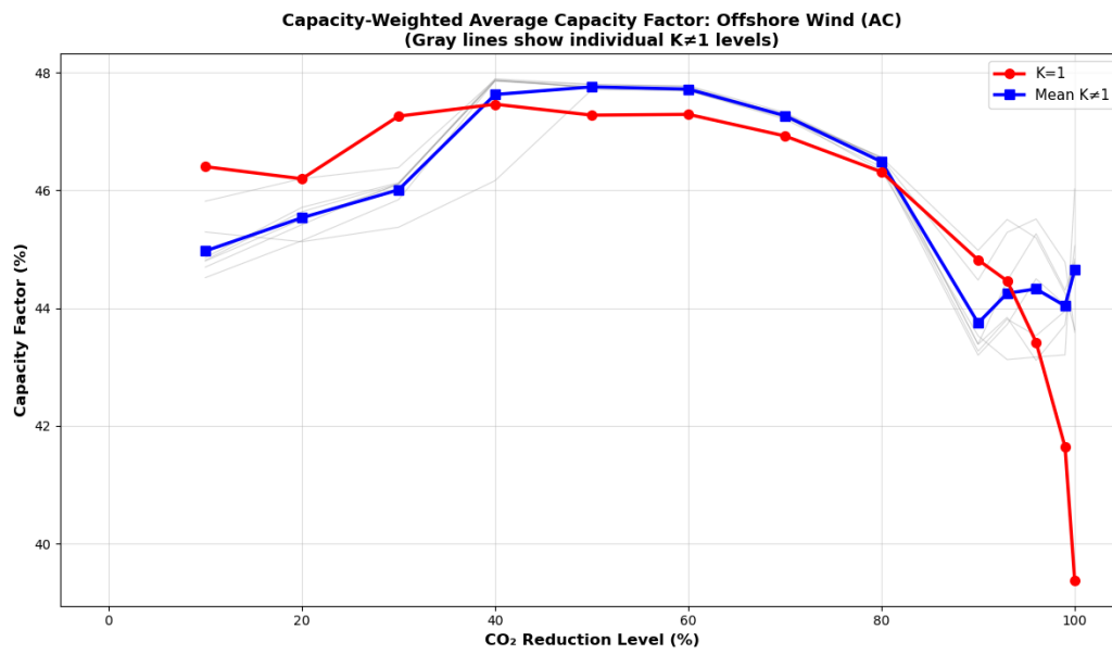
Figure 38: Mean capacity factor for offshore wind (AC) across K-constraints and decarbonization levels.
