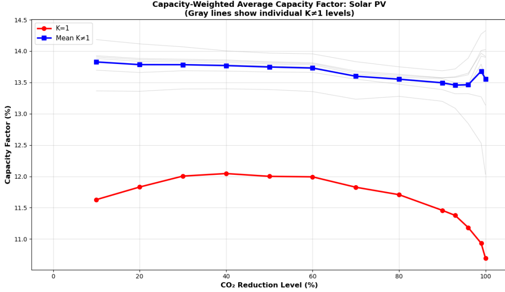
Figure 28: Mean capacity factor for solar PV across K-constraints and decarbonization levels.
