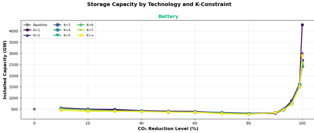
Figure 30: Installed battery and hydrogen storage capacity across K-constraints and decarbonization levels.
