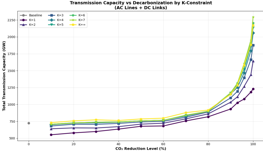
Figure 29: Total installed transmission capacity across K-constraints and decarbonization levels.
