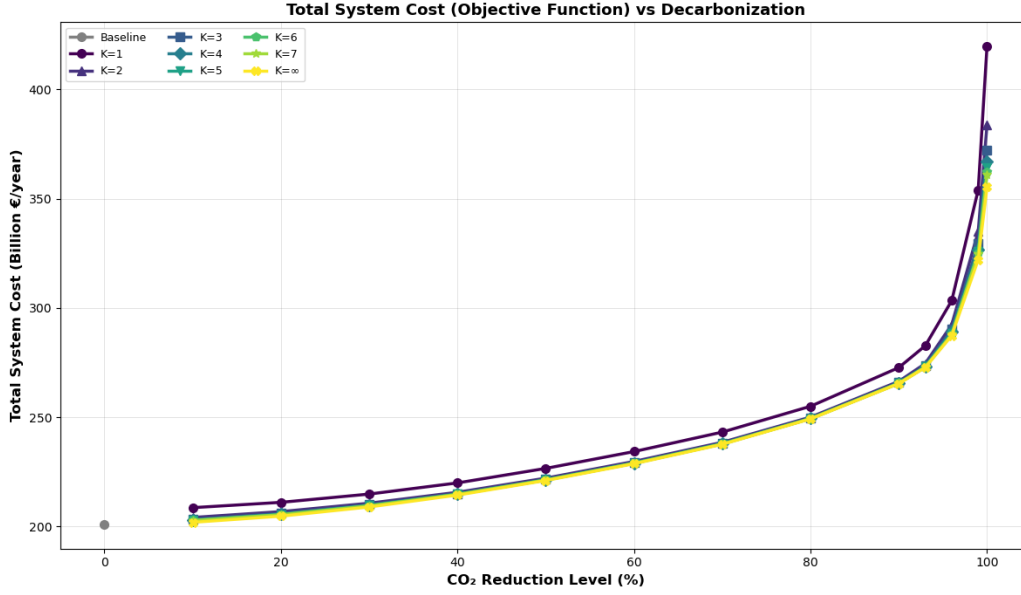
Figure 33: Total system cost across K-constraints and decarbonization levels.
