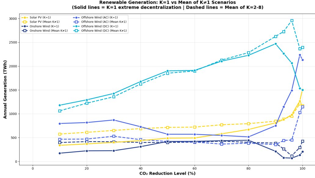
Figure 36: Total annual generation from renewable sources across K-constraints and decarbonization levels .
