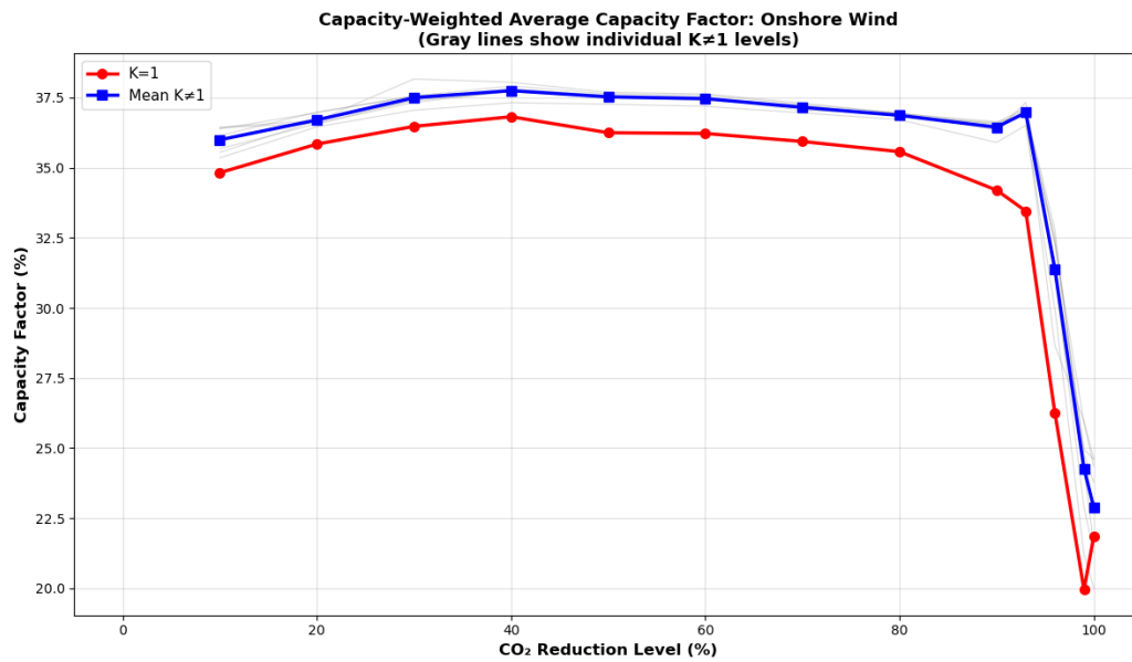
Figure 37: Mean capacity factor for onshore wind across K-constraints and decarbonization levels.
