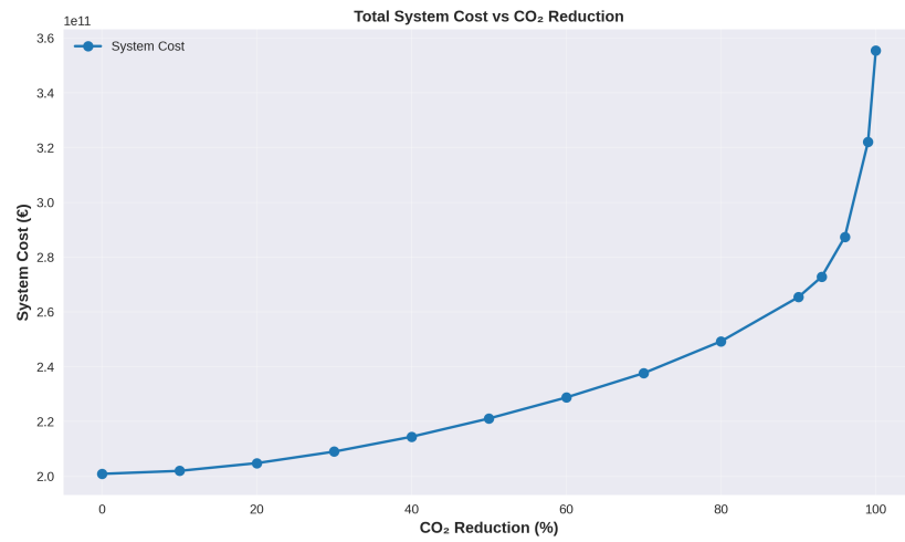
Figure 21: Total system cost in least-cost systems
