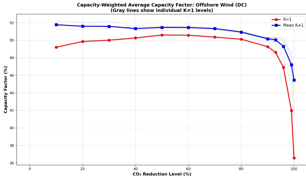
Figure 39: Mean capacity factor for offshore wind (DC) across K-constraints and decarbonization levels.
