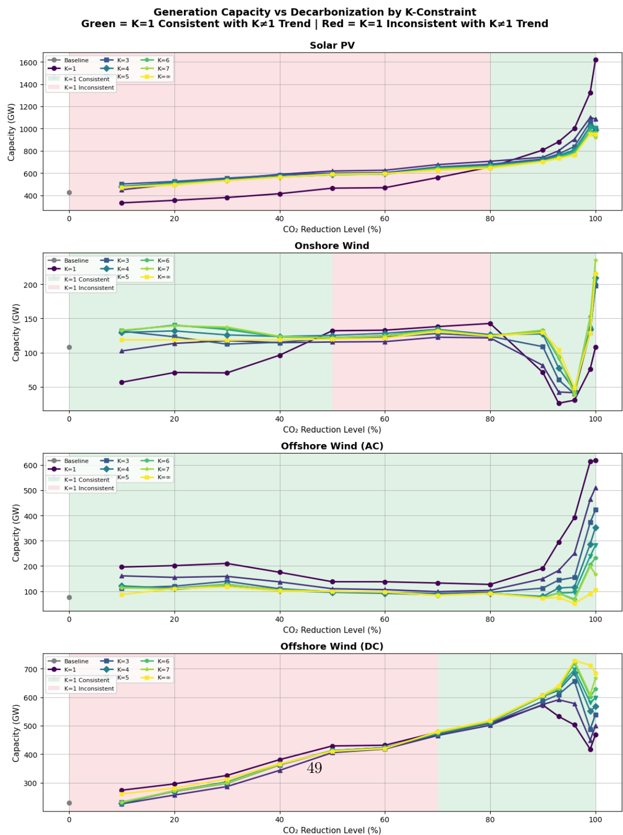
Figure 26: Total installed renewable generation capacity across K-constraints and decar-
