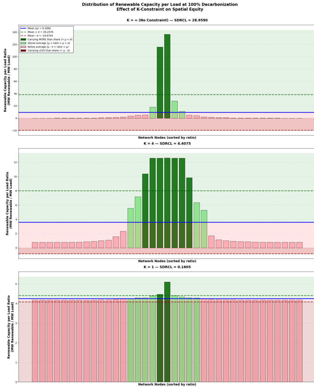
Figure 35: Distribution of renewable capacity to load ratio at 100% decarbonization for different K-constraints.
